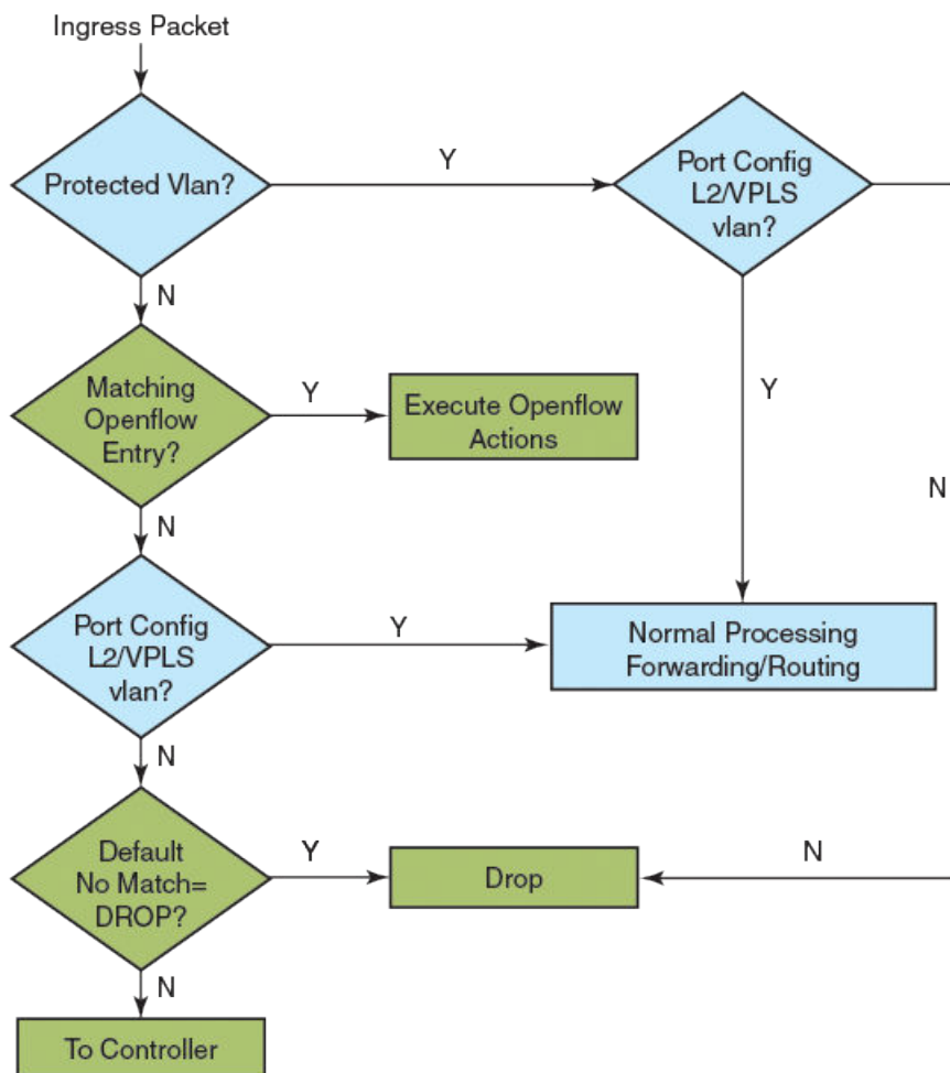
FIGURE 9 Packet flow diagram for Layer 2 support
