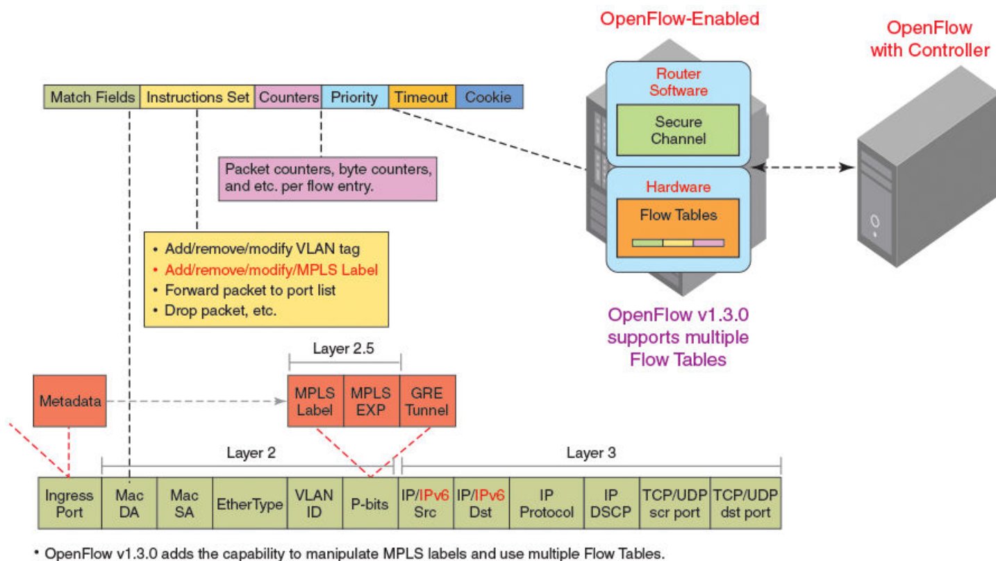
FIGURE 6 OpenFlow 1.3.0 flow table entries
