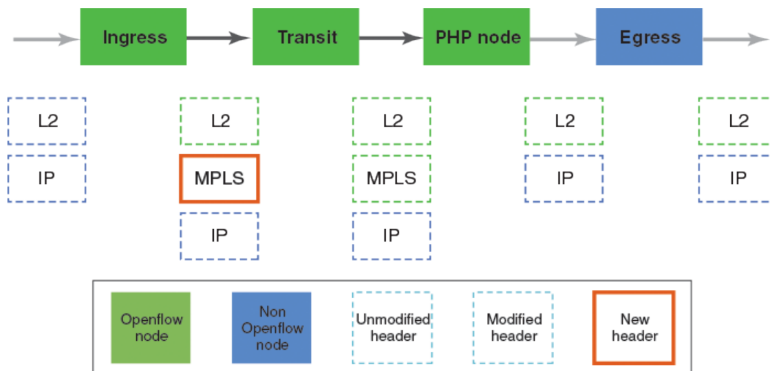
FIGURE 10 Packet modification at each node for IPv4 over MPLS
