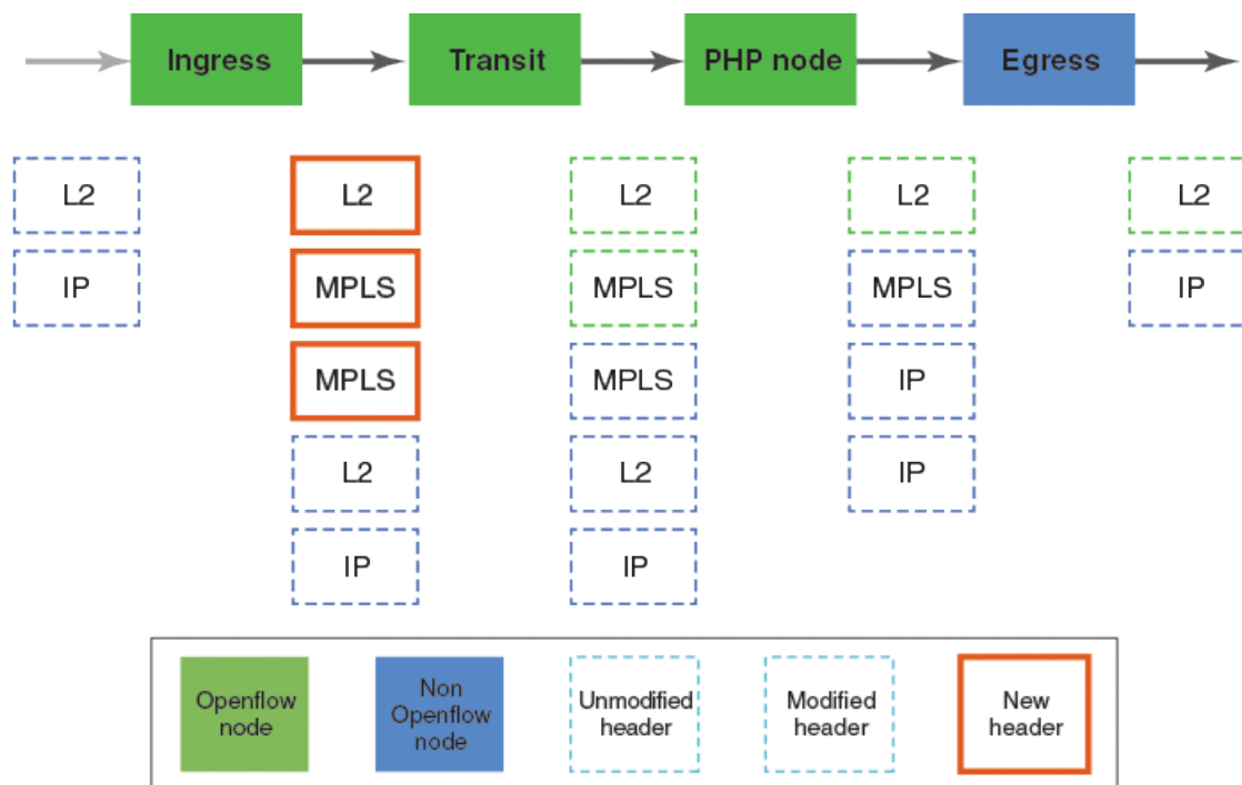
FIGURE 12 Packet modification at each node for L2VPN
