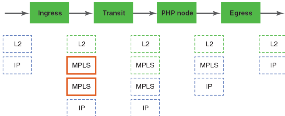
FIGURE 11 Packet modification at each node for IPv4-L3VPN
