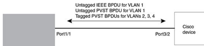
FIGURE 60 Default VLAN 1 for untagged BPDUs
