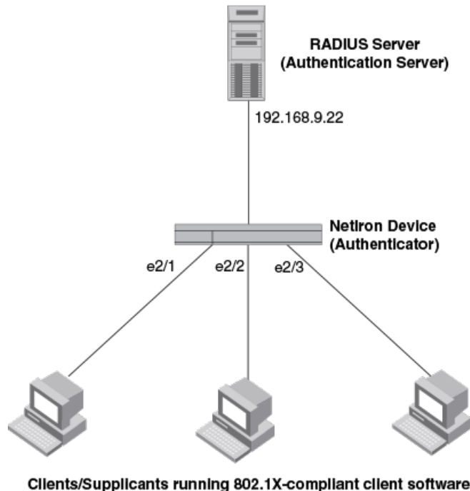
FIGURE 22 Sample point-to-point 802.1x configuration
