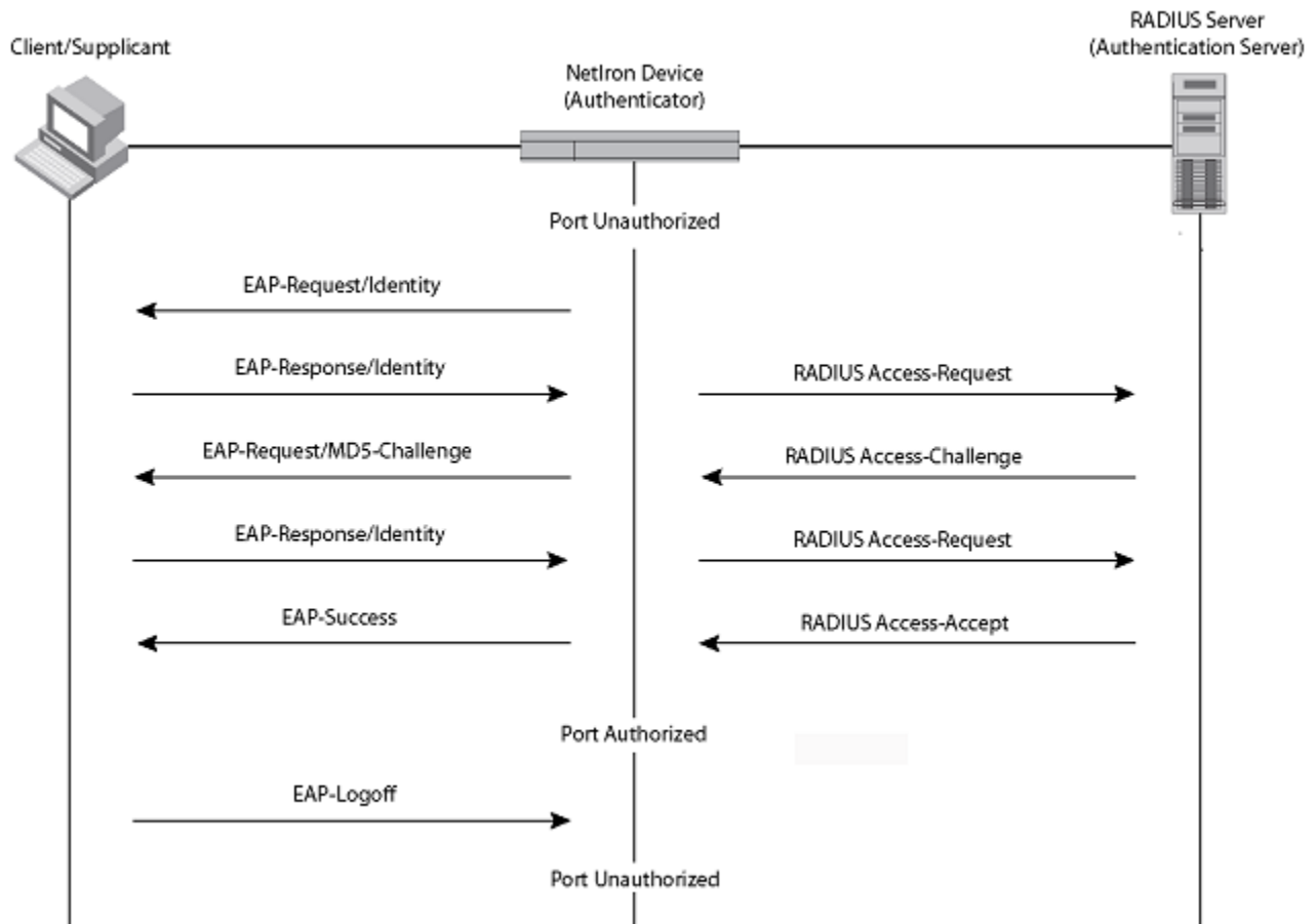
FIGURE 20 Message exchange during authentication
