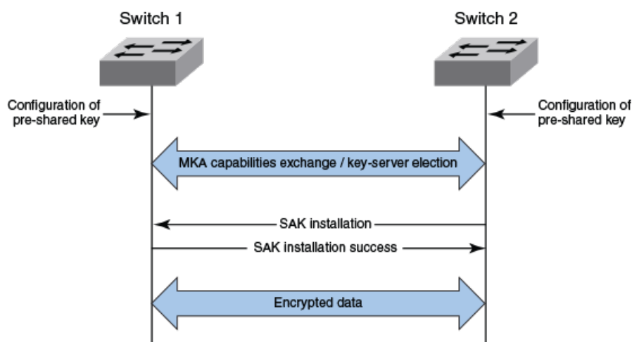
FIGURE 11 MKA pre-shared key and key name exchange between two switches
