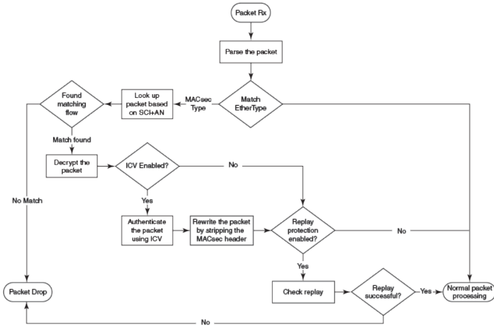
FIGURE 14 MACsec incoming frames
