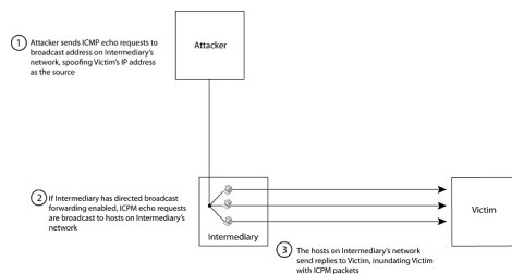
FIGURE 16 How a smurf attack floods a victim with ICMP replies
