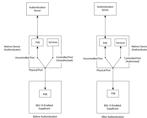
FIGURE 19 Controlled and uncontrolled ports before and after client authentication
