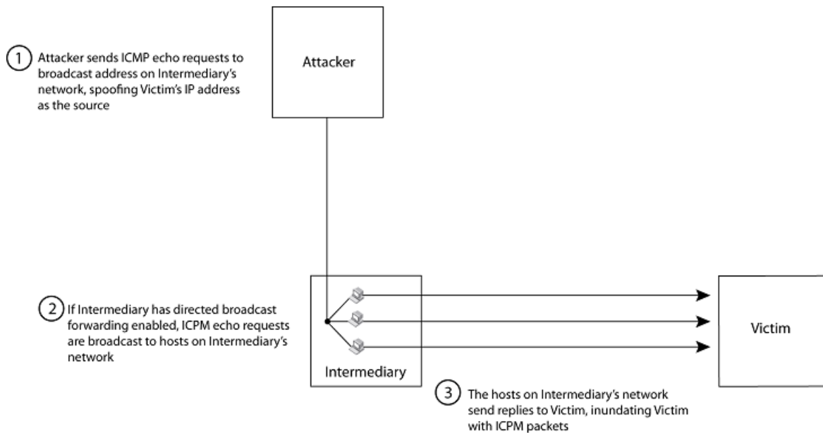
FIGURE 16 How a smurf attack floods a victim with ICMP replies
