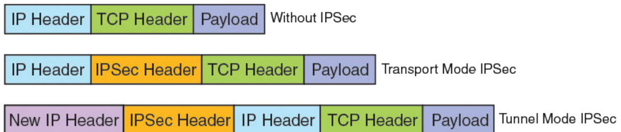
FIGURE 2 IPsec tunnel mode versus transport mode
