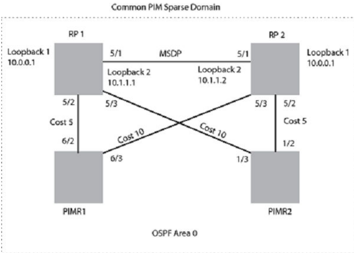
FIGURE 16 Example of a MDSP Anycast RP network
