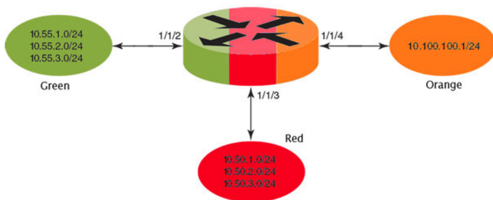
FIGURE 46 Static Inter-VRF leaking
