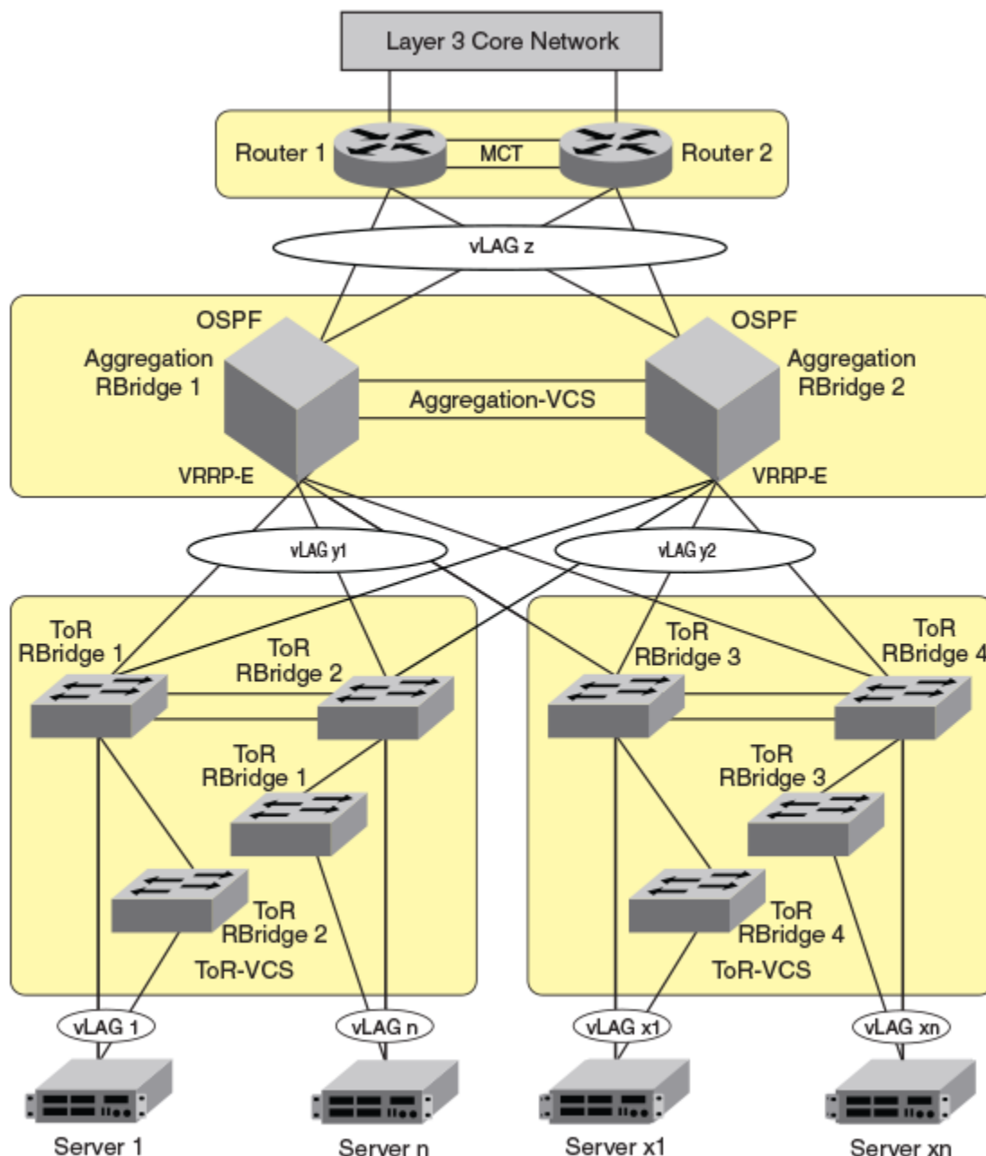
FIGURE 3 Two-tier VCS deployment
