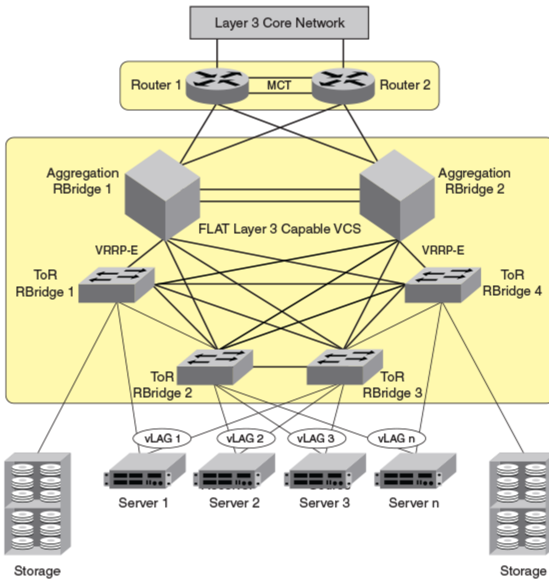
FIGURE 2 Single-tier VCS deployment
