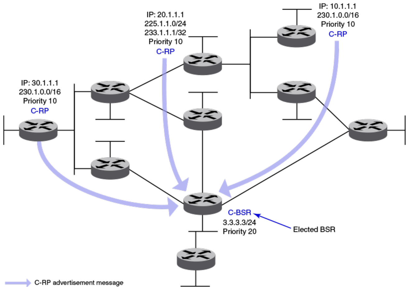
FIGURE 5 Candidate RP advertisement and RP-set formation
