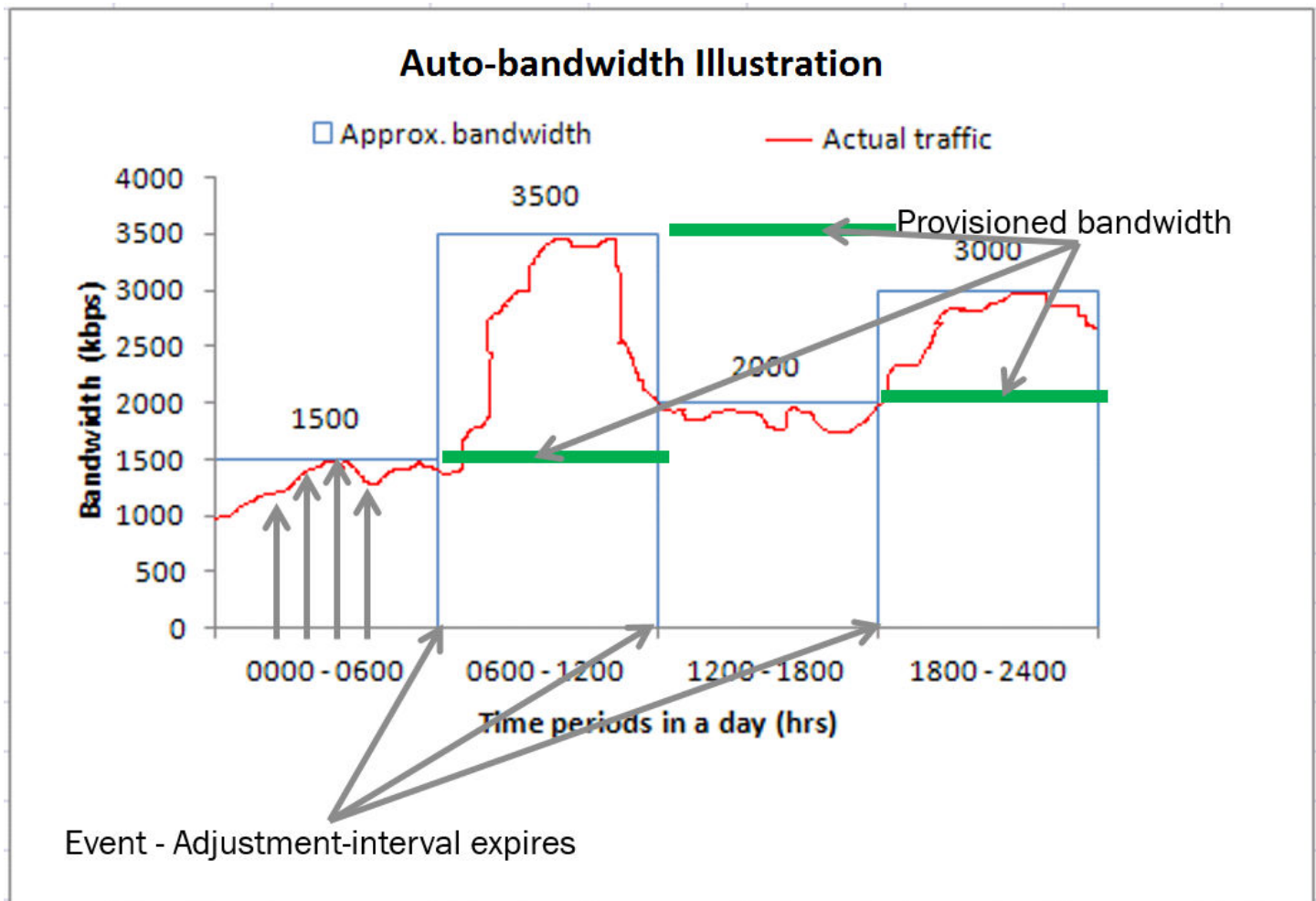
FIGURE 25 Basic auto-bandwidth functionality
