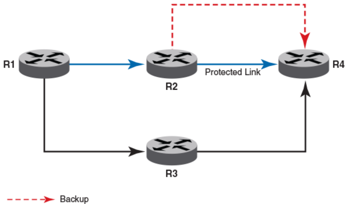
FIGURE 21 Link protection
