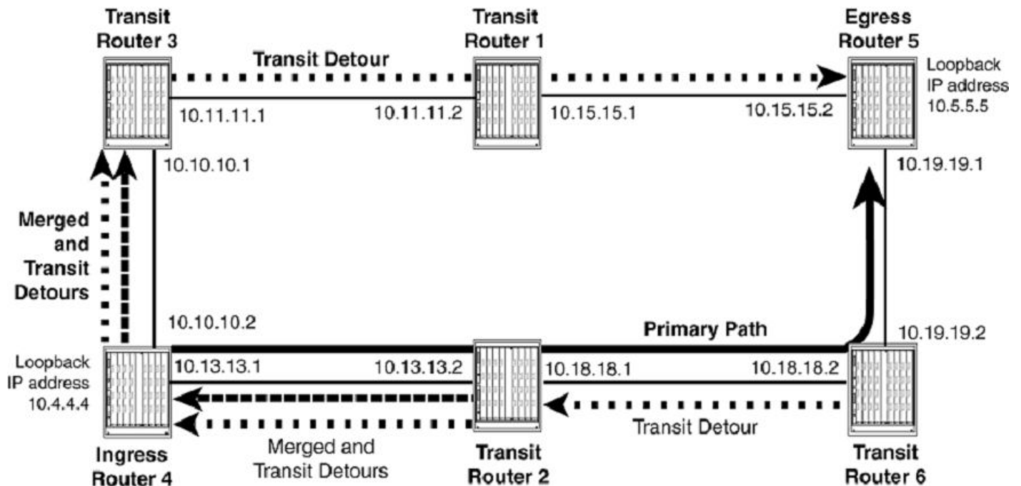
FIGURE 24 MPLS Fast Reroute Loop configuration
