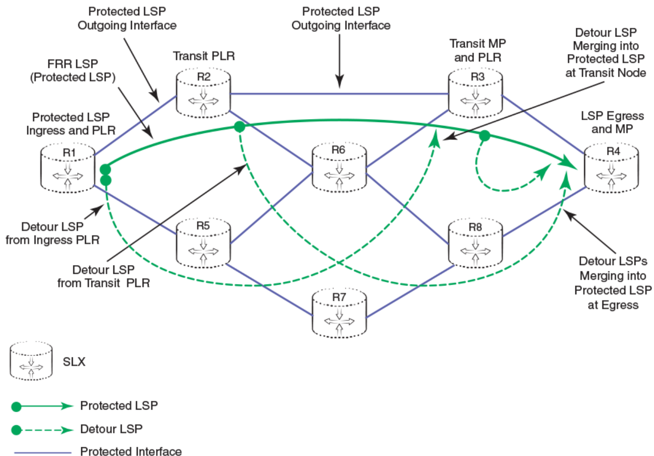
FIGURE 10 FRR (Protected) LSP, Detour LSP, PLR, and MP
