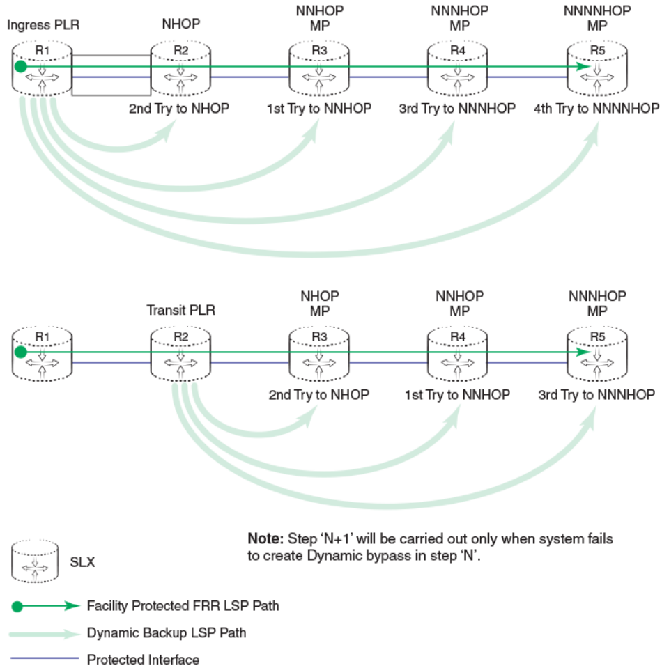
FIGURE 20 Dynamic bypass creation order
