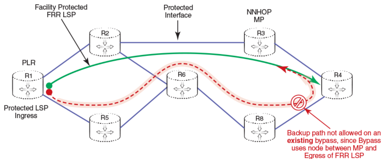
FIGURE 16 Regular bypass LSP selection
