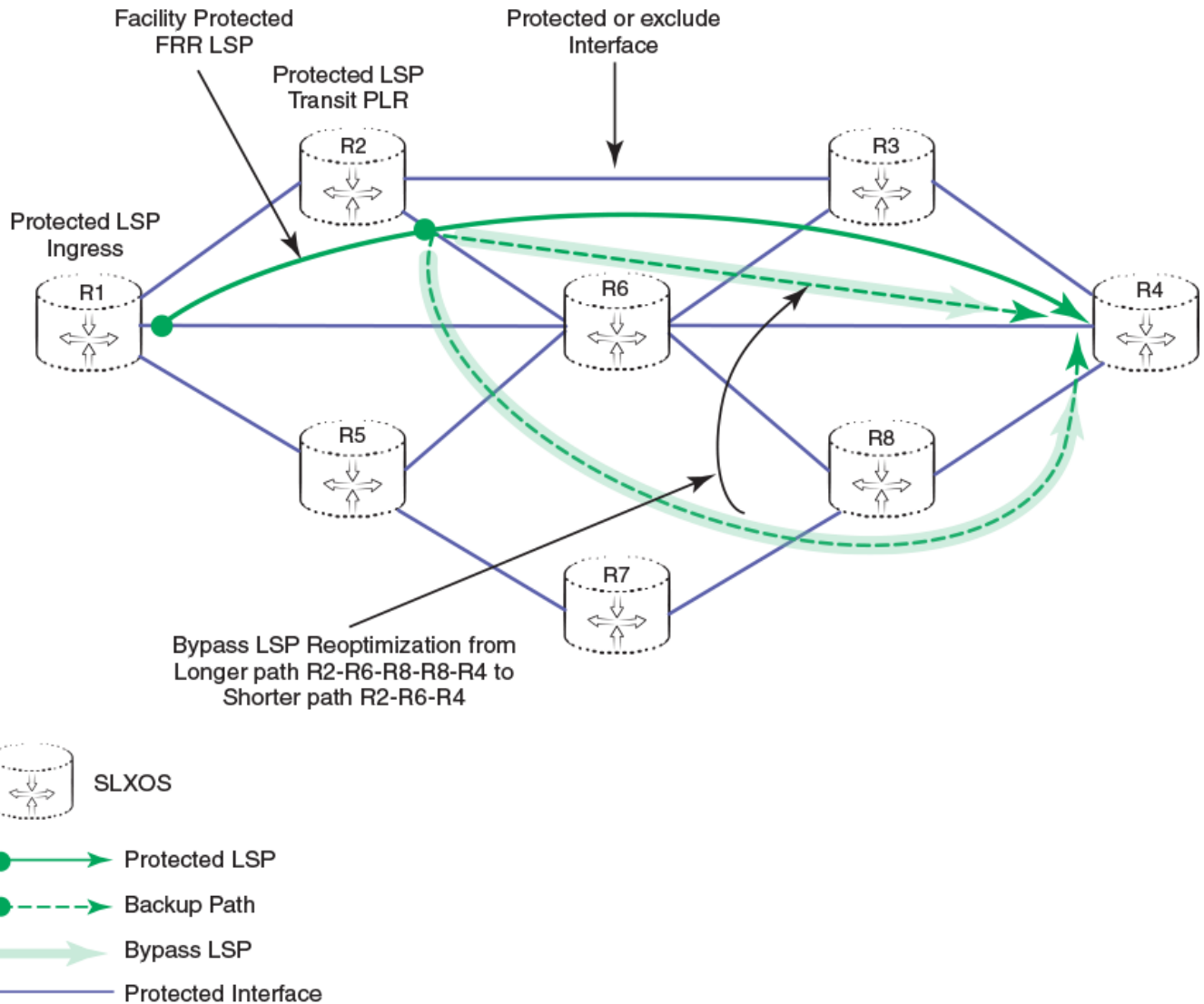
FIGURE 15 Bypass LSP re-optimization at FRR LSP transit PLR
