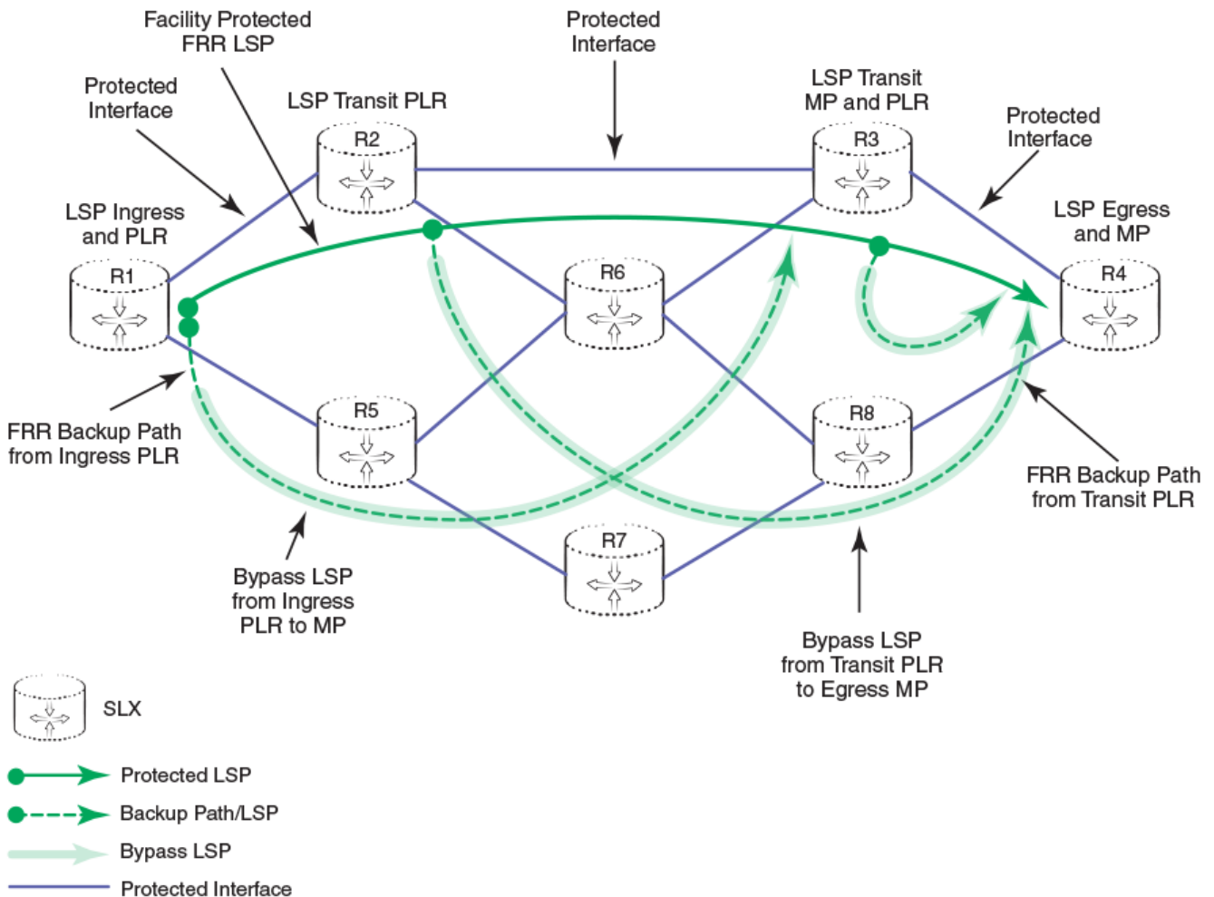
FIGURE 11 Facility-protected LSP, bypass LSP, and backup protection
