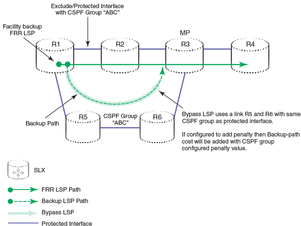
FIGURE 18 Backup path bypass using the same CSPF group as a protected interface
