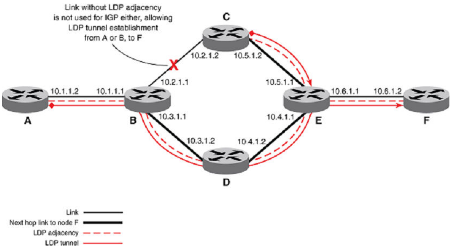
FIGURE 27 Example with LDP-IGP synchronization
