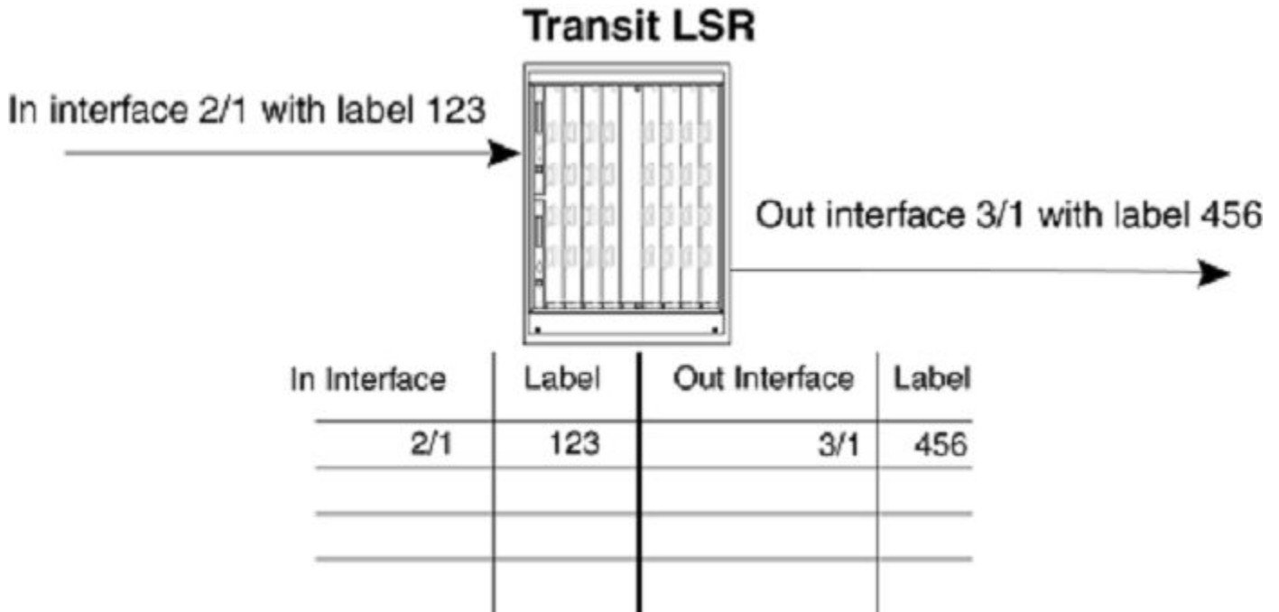
FIGURE 29 LDP-enabled LSR configuration
