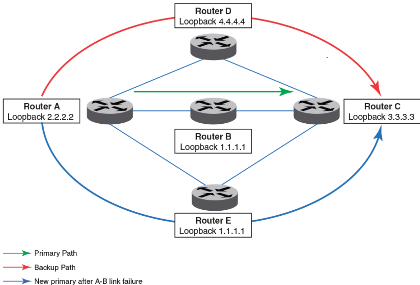
FIGURE 23 Sample topology for global revertiveness
