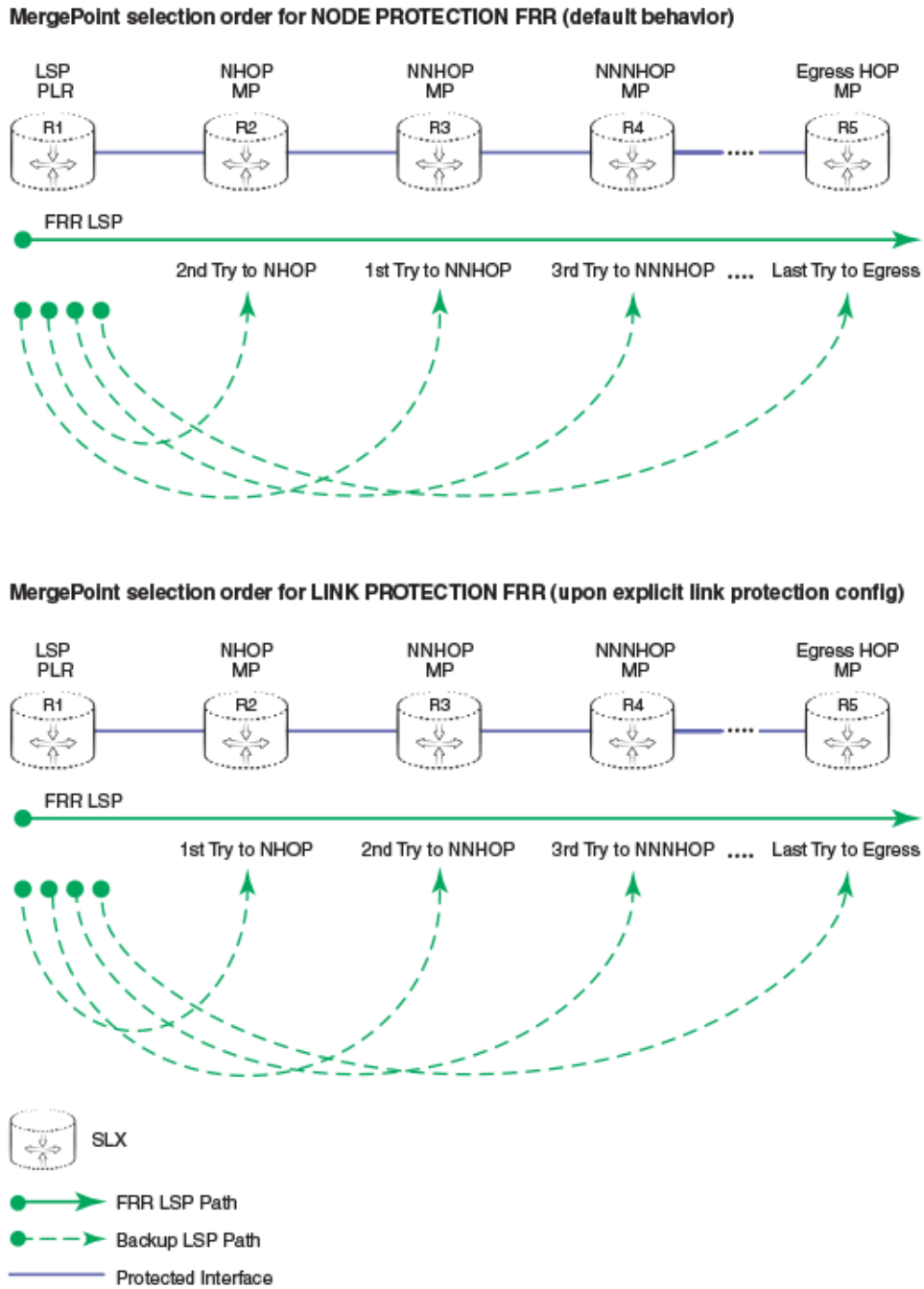
FIGURE 12 Merge Point selection order for node protection and link protection FRR
