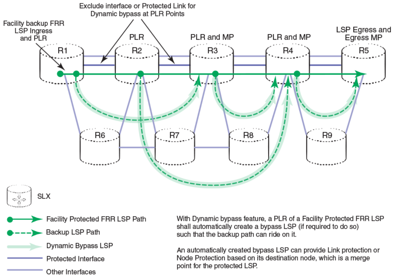
FIGURE 19 Dynamic bypass protected interface and possible dynamic bypasses at a FRR LSP PLRs
