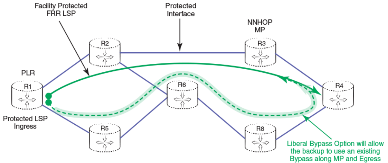
FIGURE 17 Liberal bypass LSP selection
