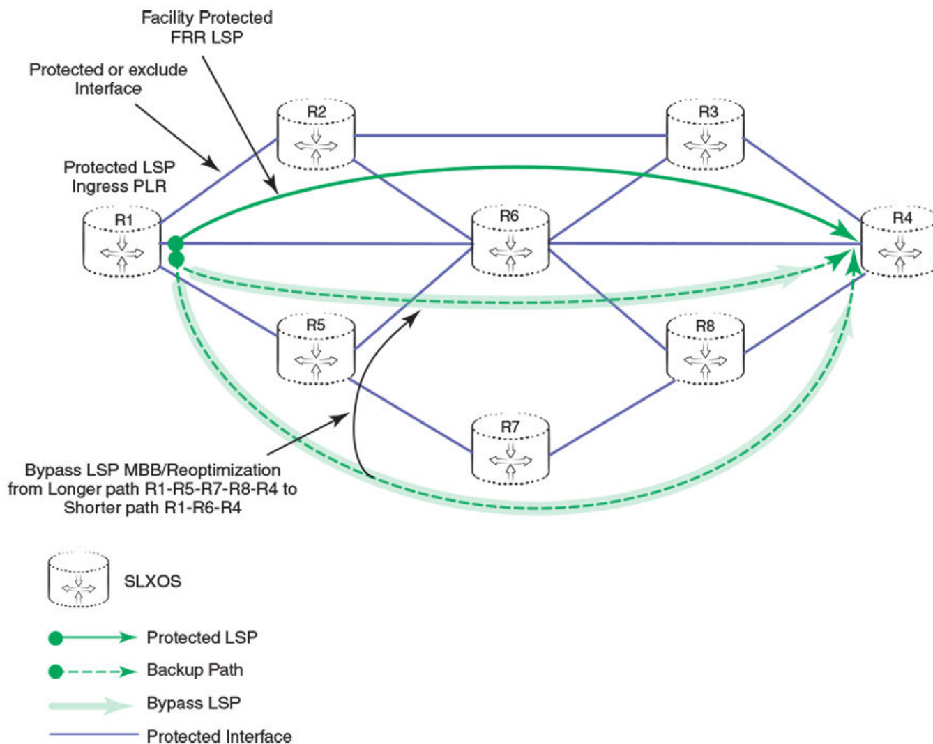
FIGURE 14 Bypass LSP re-optimization at FRR LSP ingress
