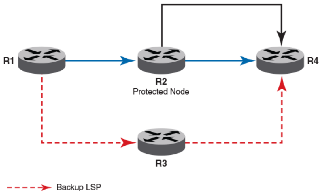
FIGURE 22 Node protection
