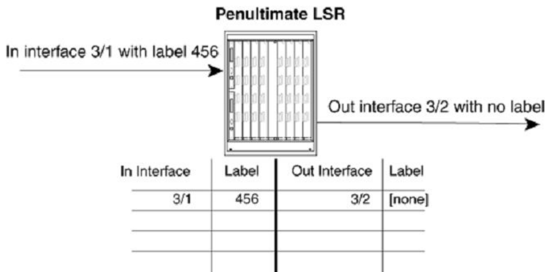
FIGURE 4 Penultimate hop popping
