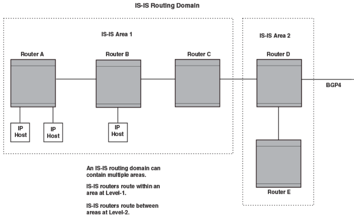
FIGURE 14 An IS-IS network contains Intermediate Systems (ISs) and host systems
