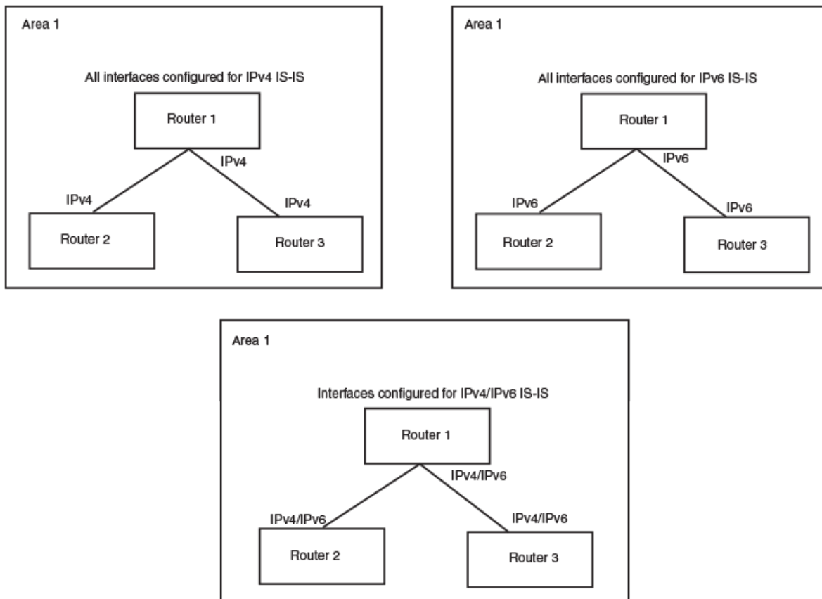
FIGURE 18 IPv6 IS-IS in single-topology mode
