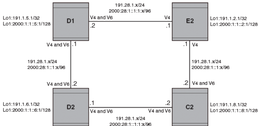
FIGURE 21 IPv6 IS-IS MT configuration
