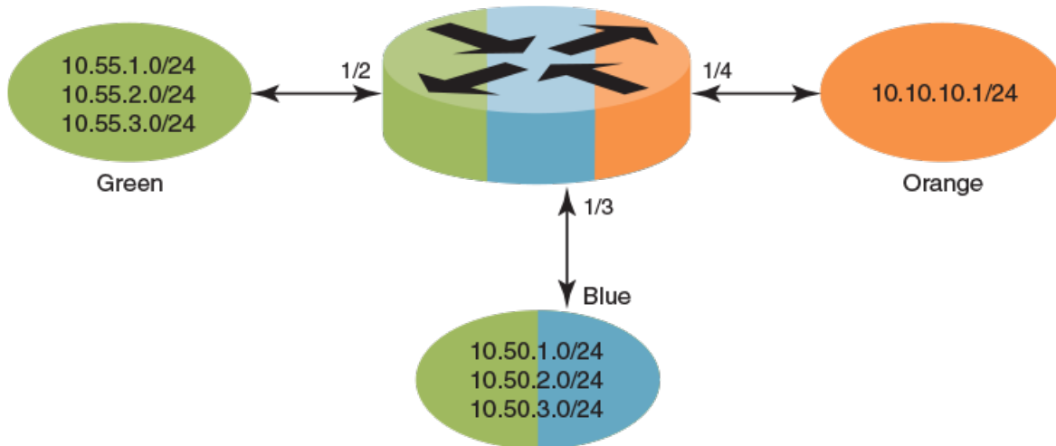
FIGURE 24 Static inter-VRF route leaking
