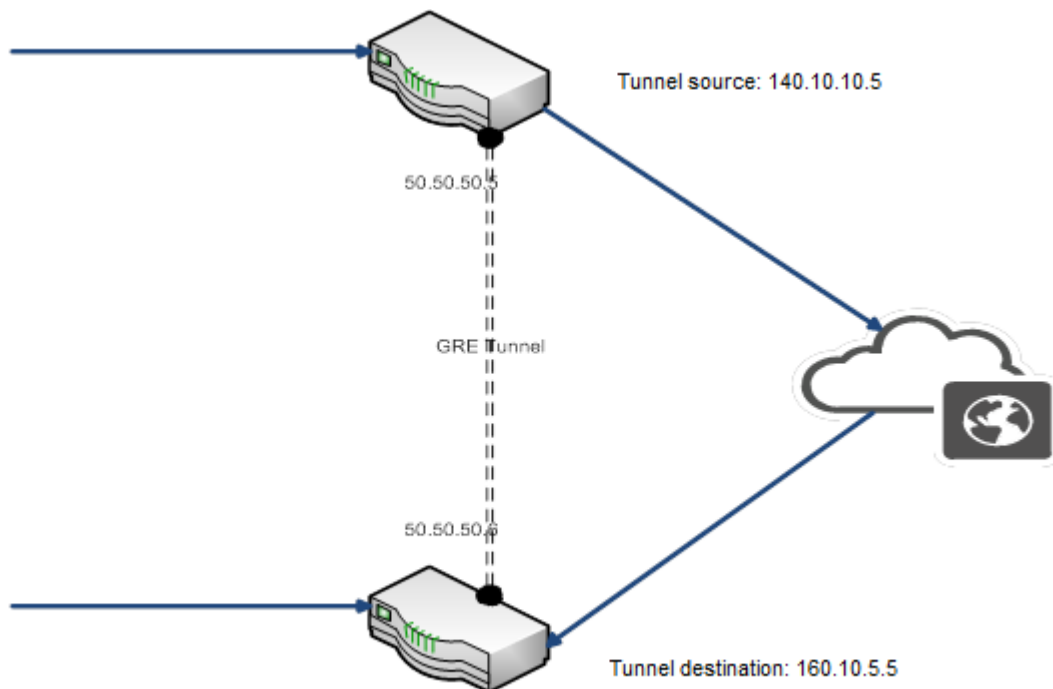
FIGURE 11 GRE tunnel
