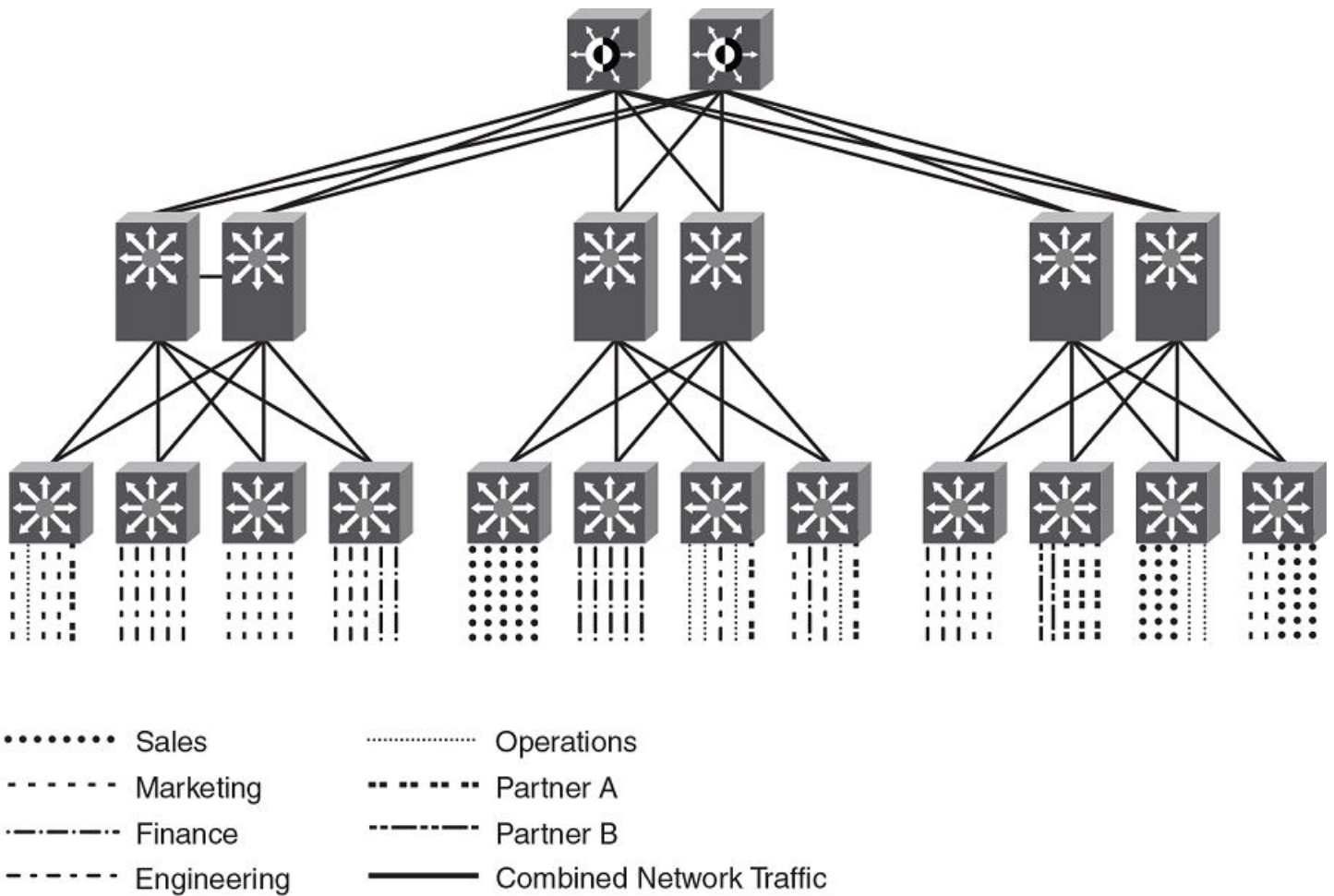
FIGURE 22 Example high-level Multi-VRF topology
