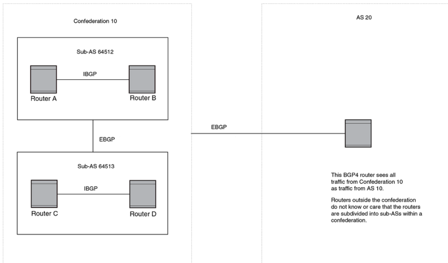
FIGURE 13 Example BGP4 confederation
