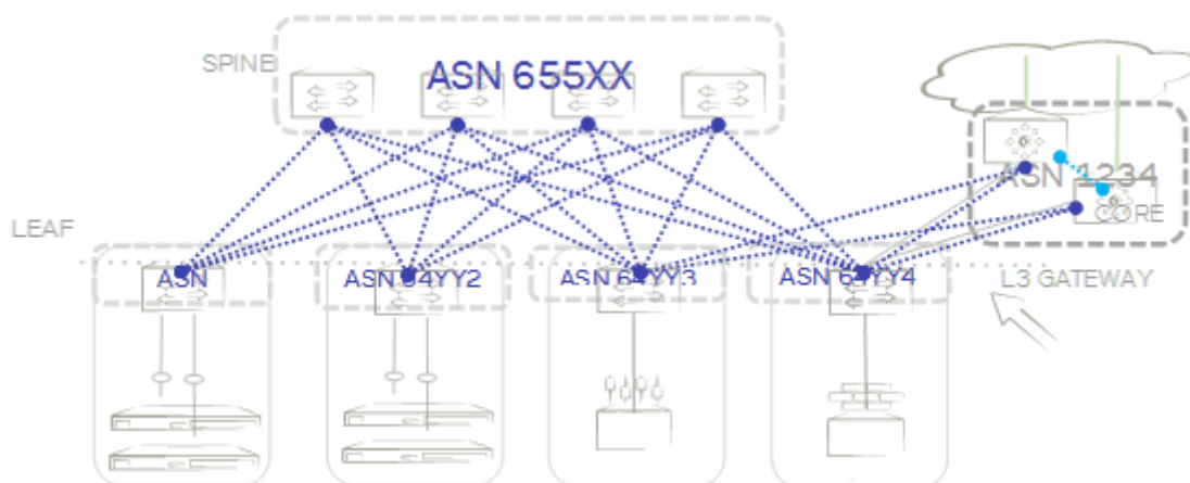
FIGURE 22 eBGP spine and leaf
