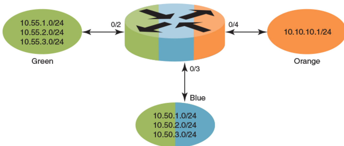
FIGURE 44 Static inter-VRF route leaking
