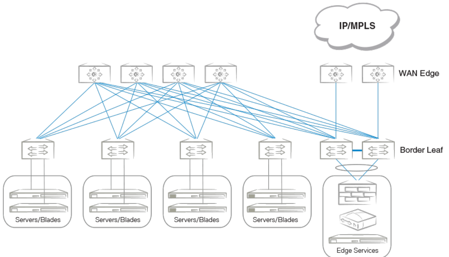
FIGURE 23 Border and service leaf
