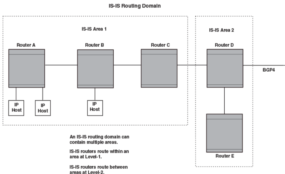
FIGURE 28 An IS-IS network contains Intermediate Systems (ISs) and host systems
