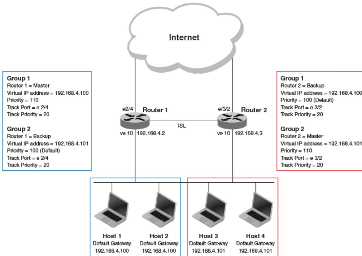
FIGURE 51 Multigroup VRRP routing topology
