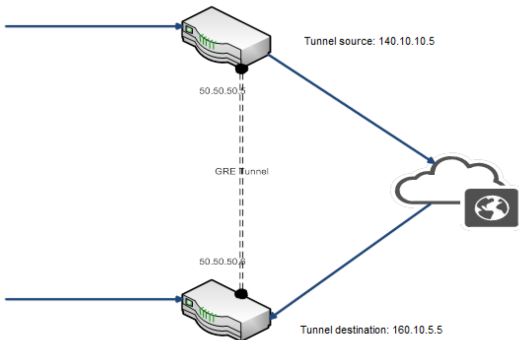
FIGURE 27 GRE tunnel
