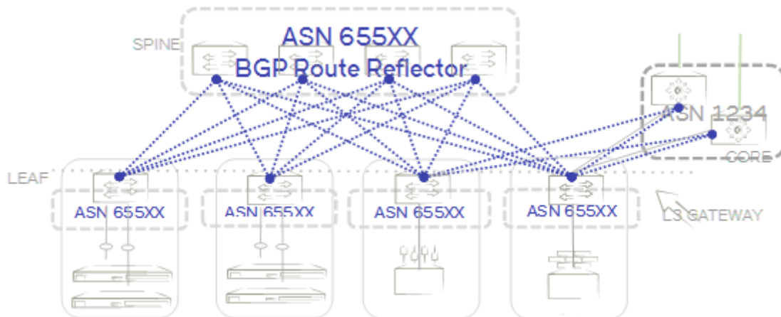
FIGURE 21 iBGP spine and leaf
