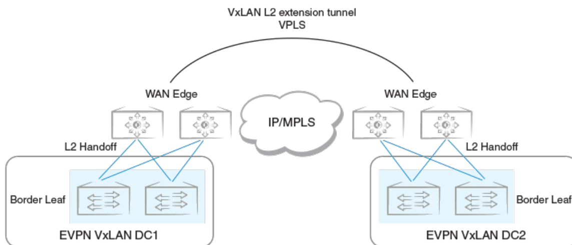
FIGURE 26 Layer 2 handoff-based DCI
