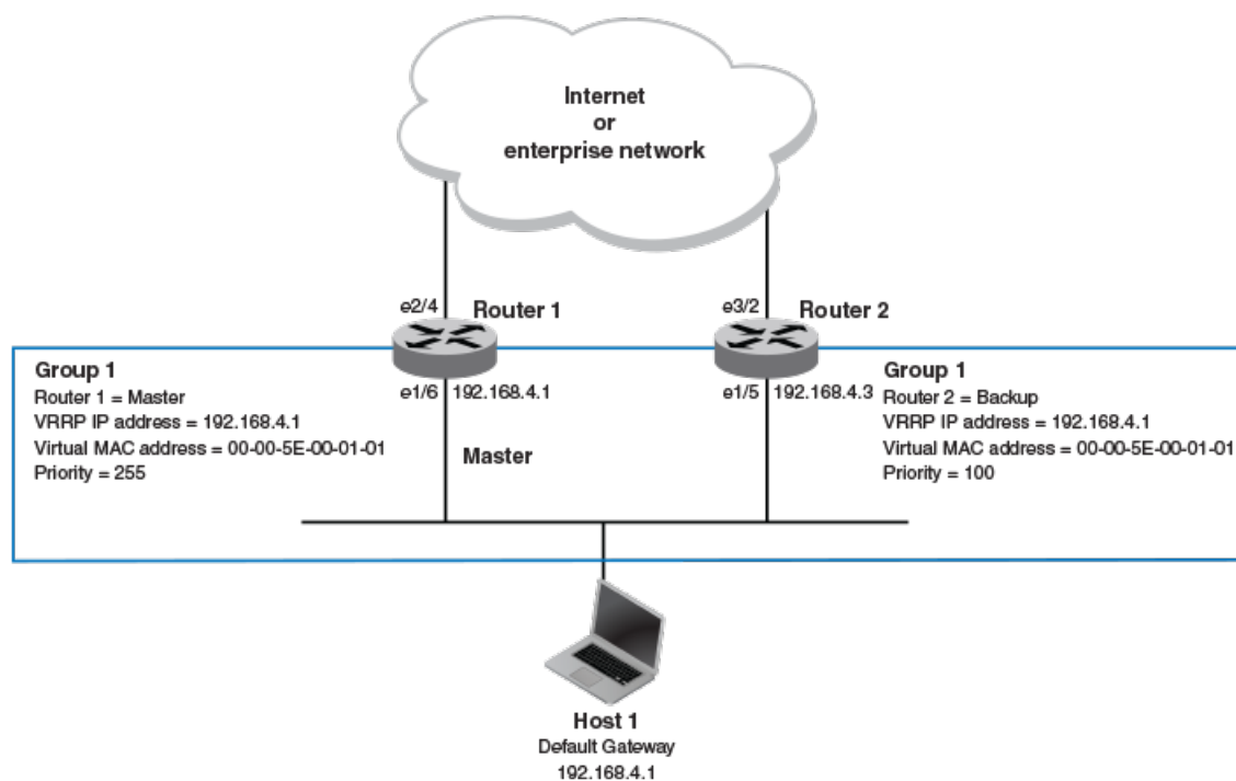
FIGURE 48 Devices configured as VRRP virtual routers for redundant network access for Host 1
