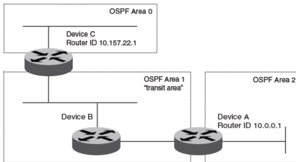
FIGURE 39 Defining OSPF virtual links within a network
