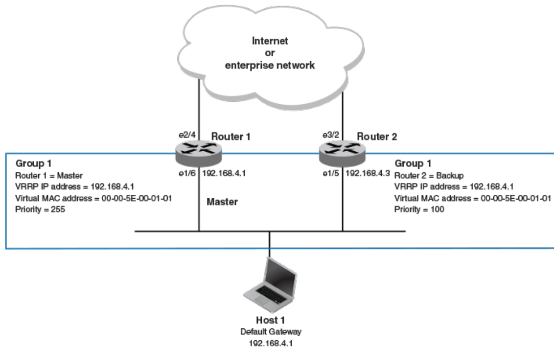
FIGURE 49 Basic VRRP topology
