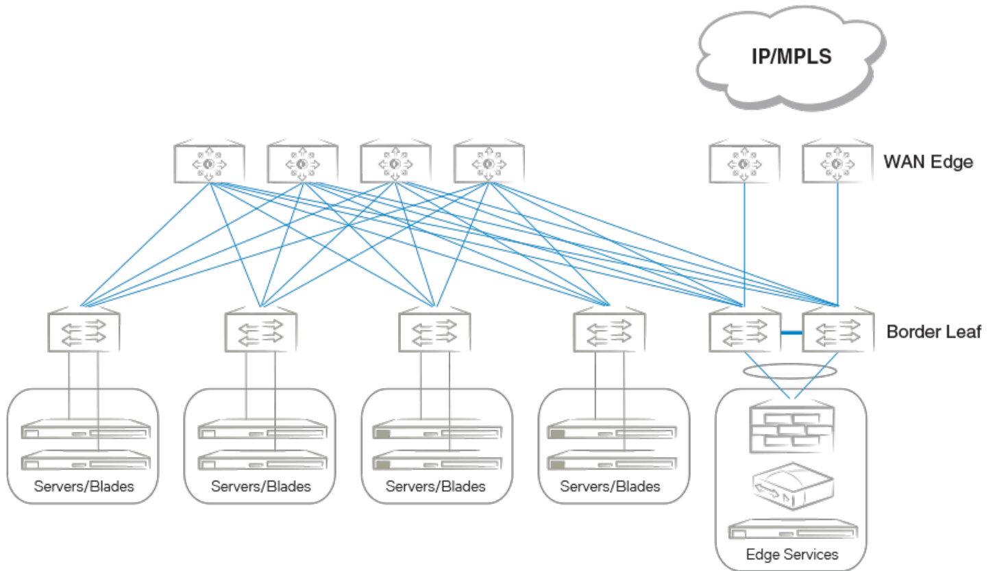
FIGURE 24 Colocated spine and border leaf
