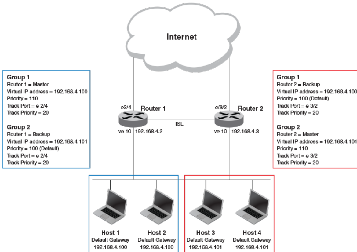
FIGURE 50 Two routers configured for dual redundant network access for the host
