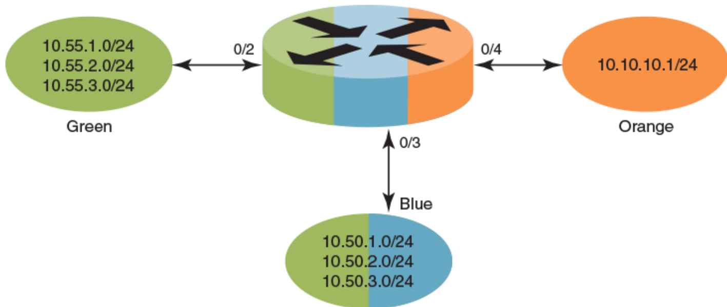
FIGURE 24 Static inter-VRF route leaking
