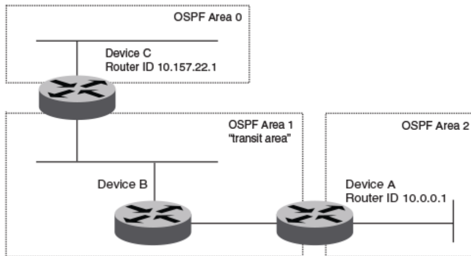
FIGURE 30 Defining OSPF virtual links within a network
