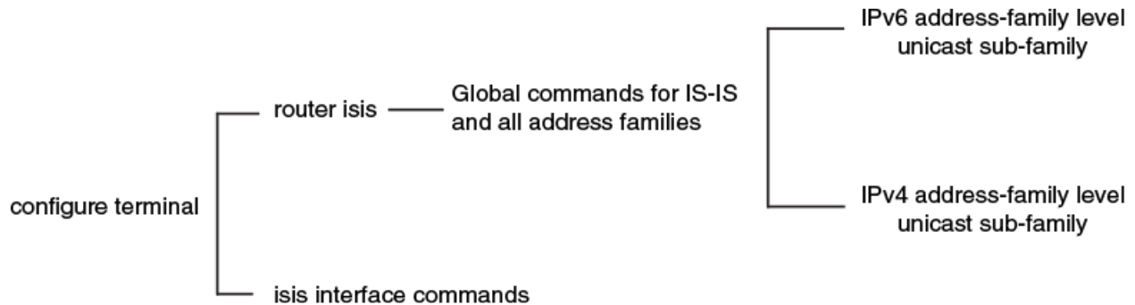
FIGURE 20 IS-IS CLI levels
