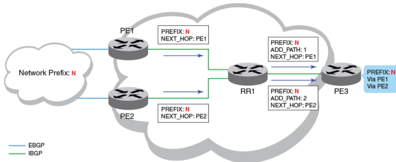
FIGURE 16 BGP additional-paths
