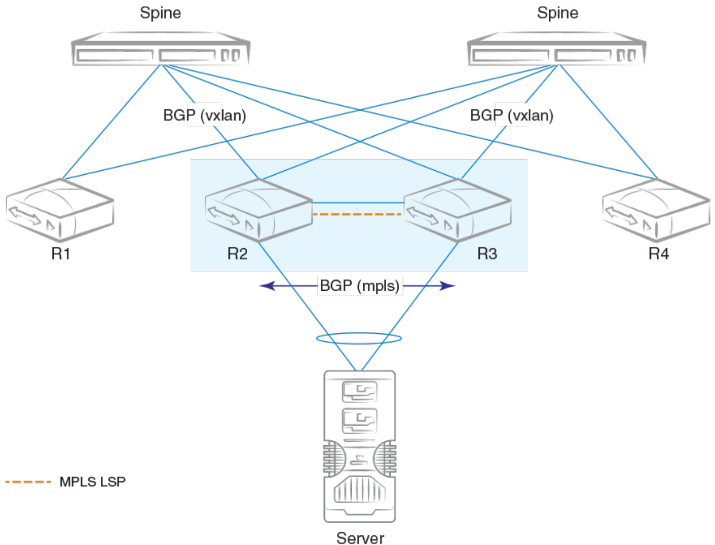
FIGURE 26 MCT with LVTEP and direct BGP peering
