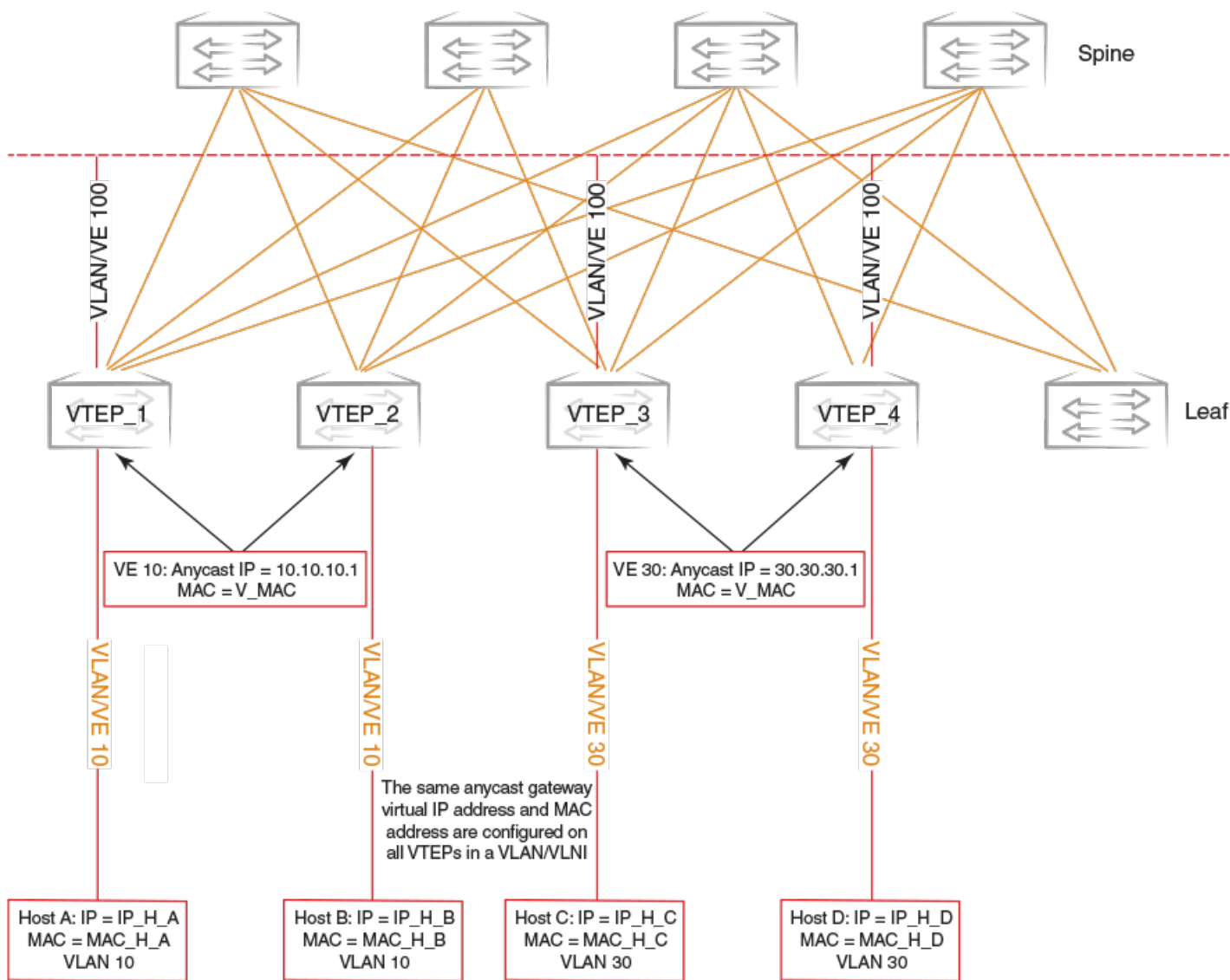
FIGURE 30 Static anycast gateway
