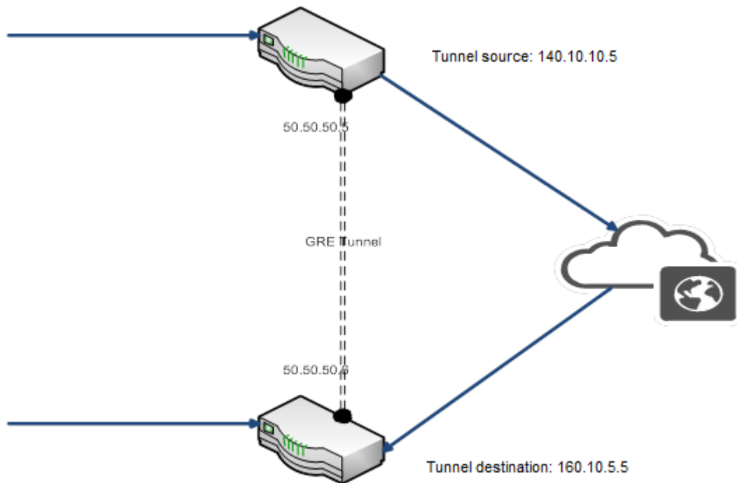
FIGURE 32 GRE tunnel
