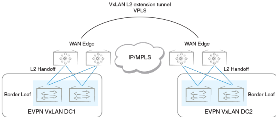
FIGURE 28 Layer 2 handoff-based DCI
