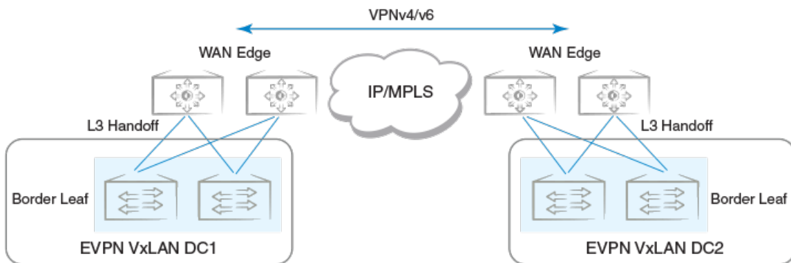
FIGURE 29 Layer 3 handoff-based DCI
