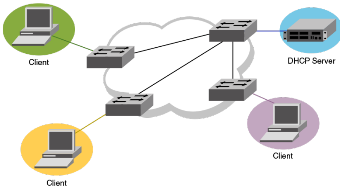
FIGURE 50 Inter-VRF route leaking example for connecting clients to a DHCP server in a different VRF.
