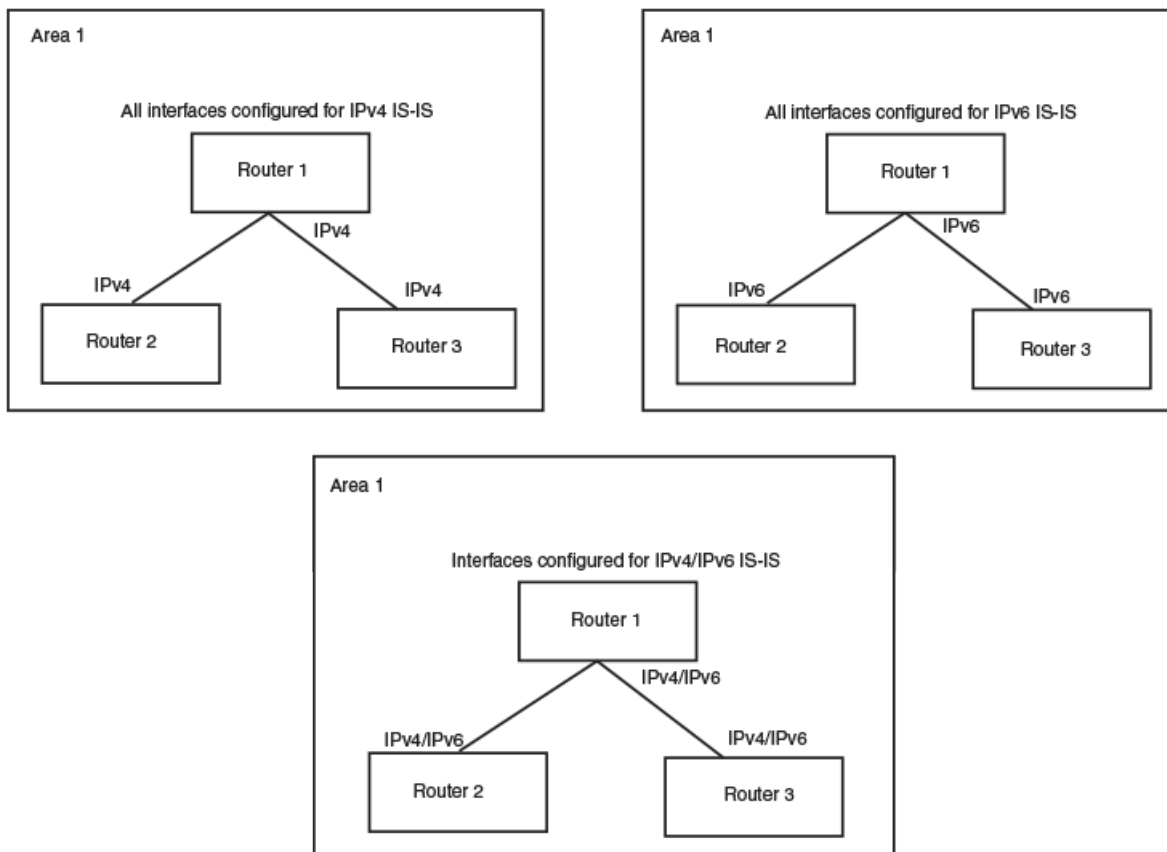
FIGURE 37 IPv6 IS-IS in single-topology mode
