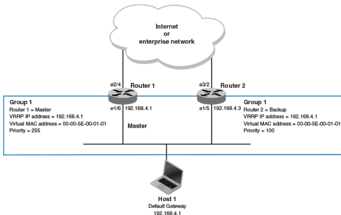
FIGURE 53 Devices configured as VRRP virtual routers for redundant network access for Host 1
