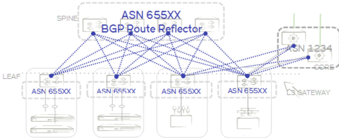
FIGURE 22 iBGP spine and leaf
