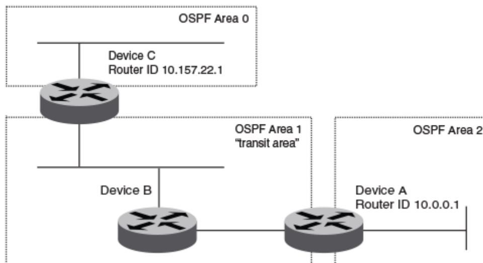
FIGURE 44 Defining OSPF virtual links within a network
