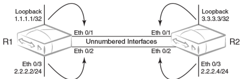
FIGURE 31 IP unnumbered and donor interfaces
