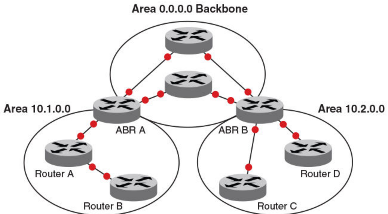
FIGURE 41 OSPF operating in a network
