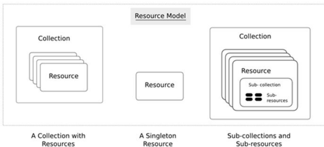
FIGURE 1 Resource Model
