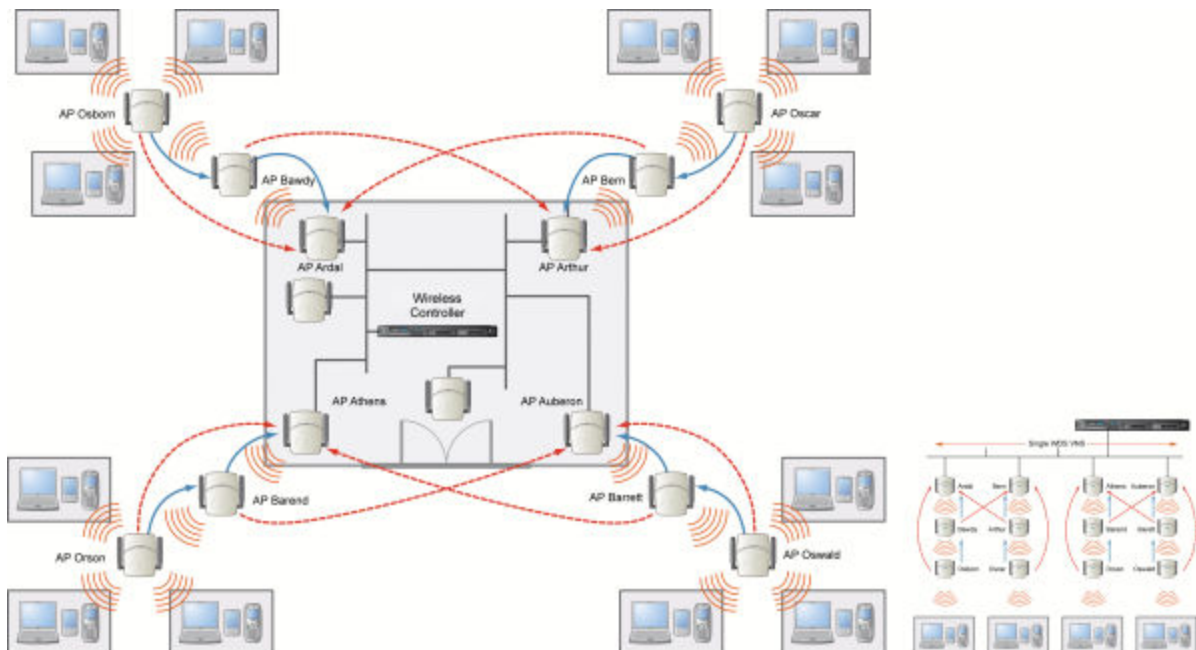
Figure 58: WDS Deployment
