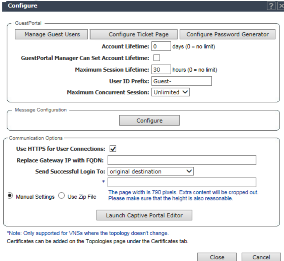
Figure 35: Captive Portal Page for Guest Portal Mode
