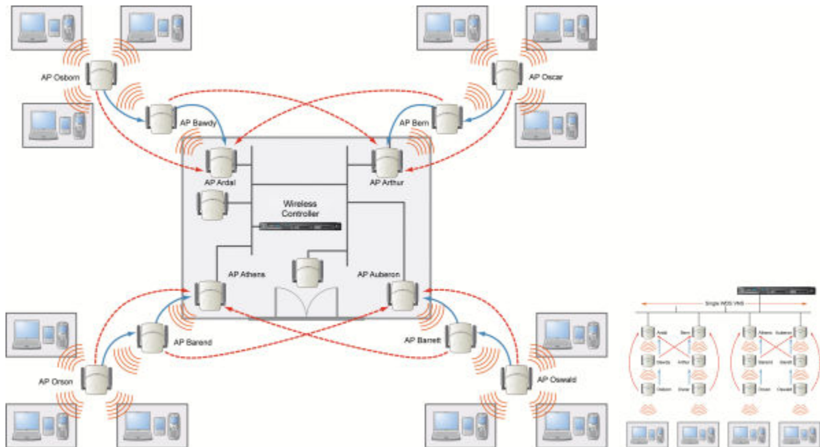
Figure 48: Mesh Deployment
