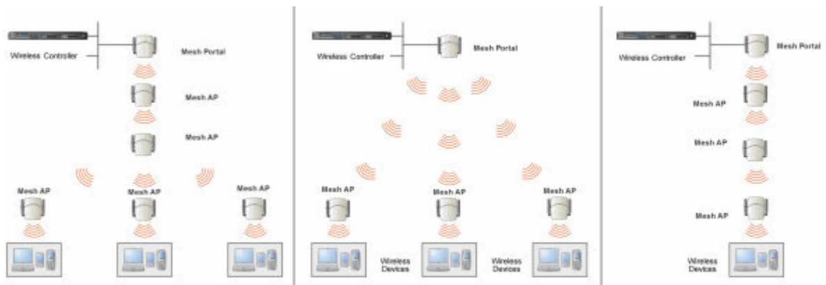
Figure 42: Examples of Mesh Deployment
