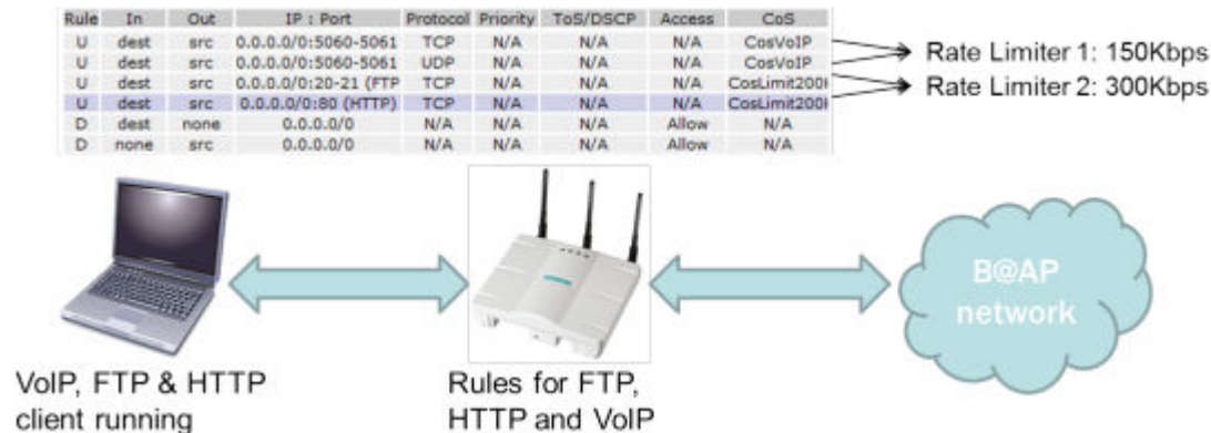
Figure 38: Rate Limiter Example
