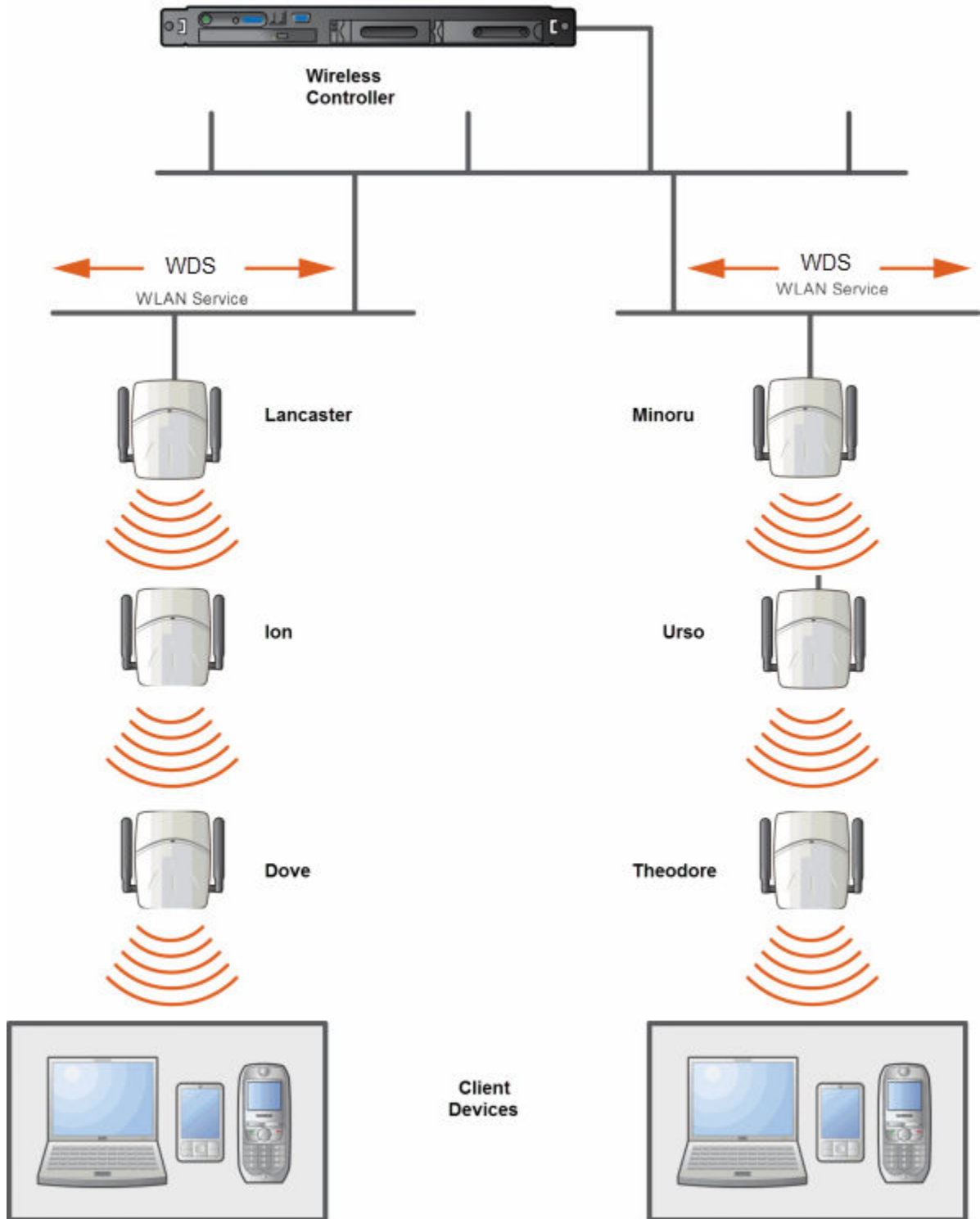
Figure 55: WDS Setup with Multiple WDS WLAN Services
