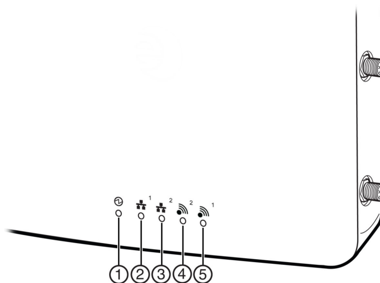
Figure 21: WS-AP3825 LEDs
