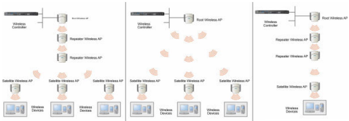
Figure 52: Examples of WDS Deployment
