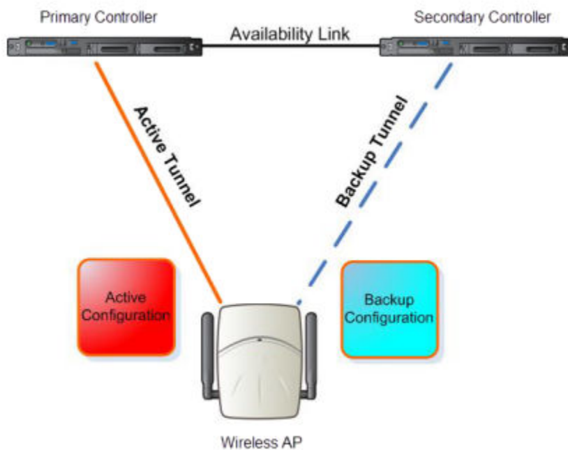
Figure 61: Session Availability Mode
