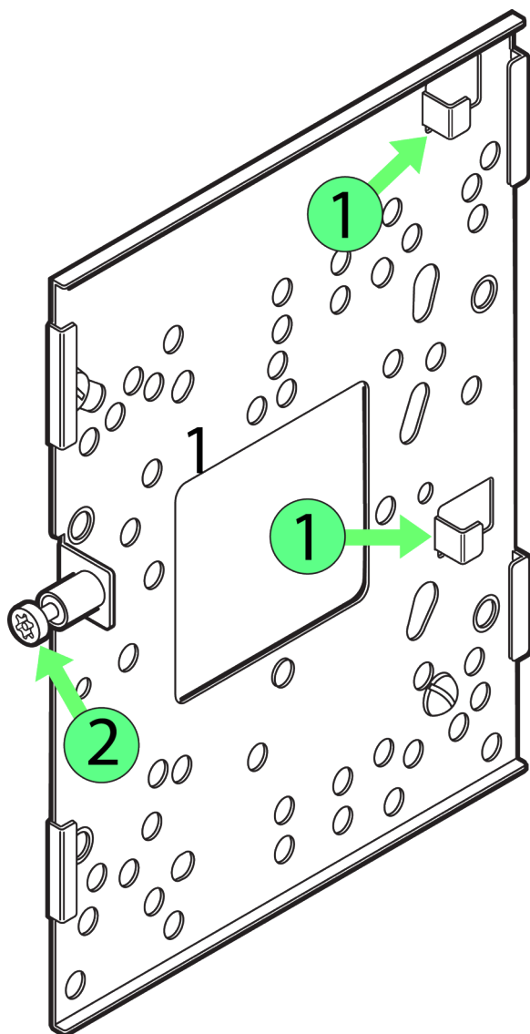
Figure 3: AP3912i Mounting Bracket
