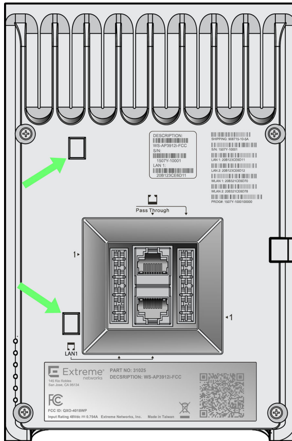
Figure 5: AP3912i Rear View
