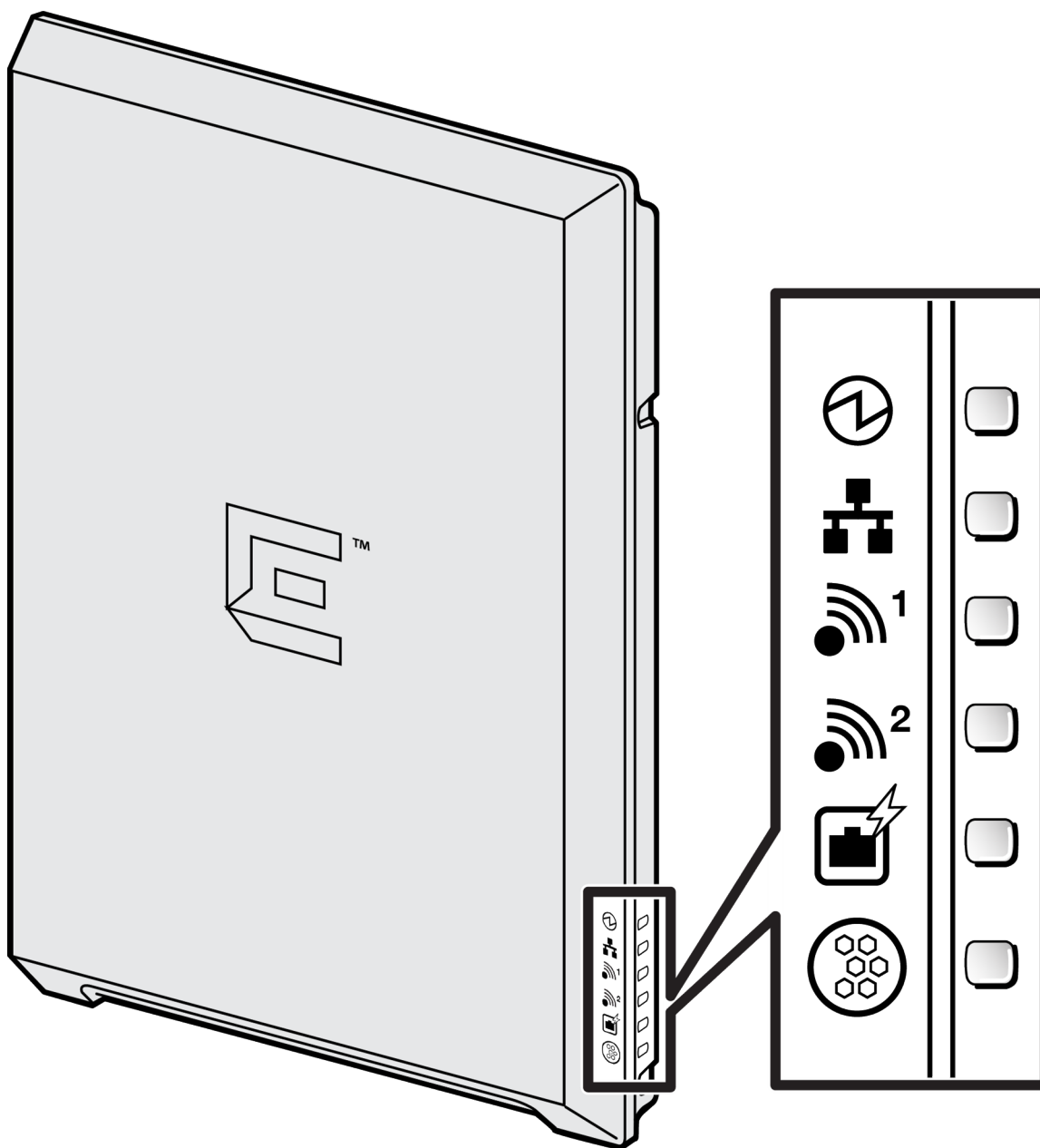
Figure 1: AP3912 LEDs
