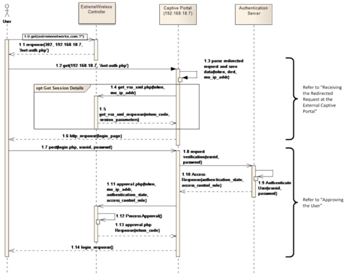
Figure 11: Flow of External Captive Portal with External Authorization
