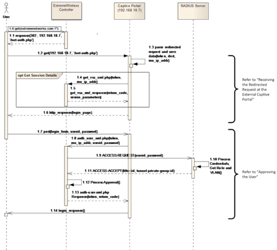
Figure 15: Flow of External Captive Portal with Internal Authorization
