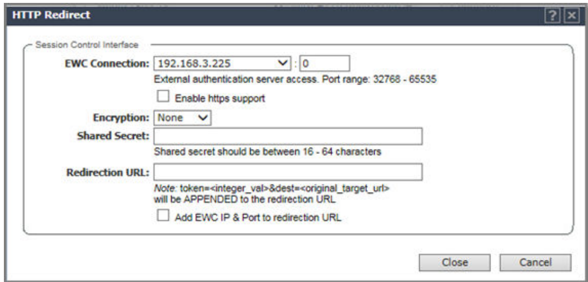
Figure 93: Captive Portal Page for External and 802.1x Modes
