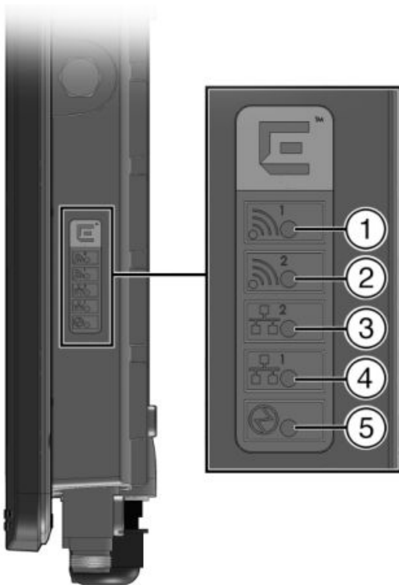
Figure 51: WS-AP3865e LEDs
