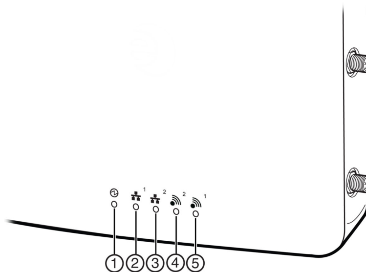
Figure 52: WS-AP3825 LEDs
