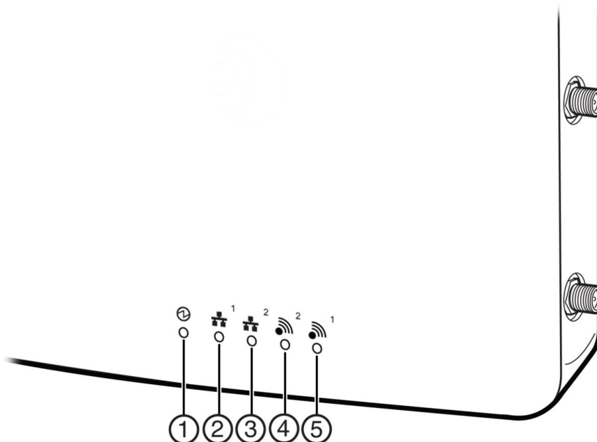
Figure 55: WS-AP3715 LEDs
