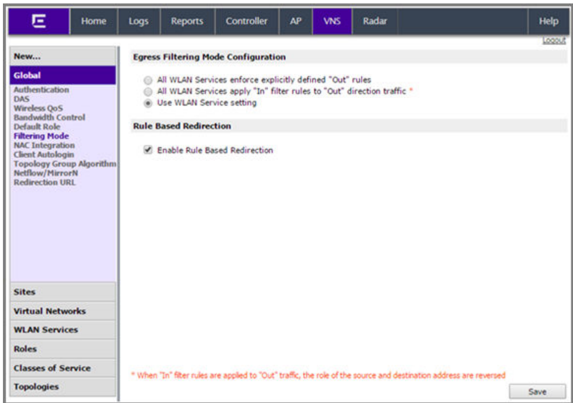
Figure 123: Egress Filtering Mode
