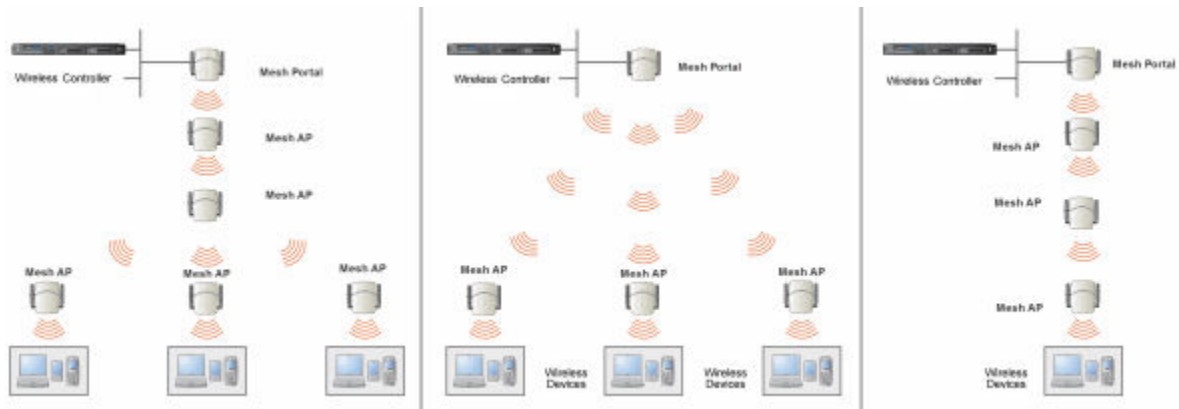
Figure 133: Examples of Mesh Deployment
