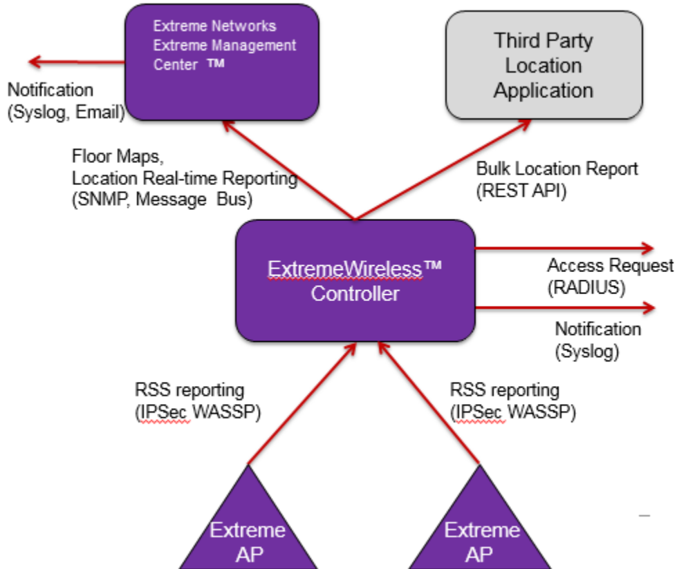
Figure 175: Components of Location Aware Services Solution
