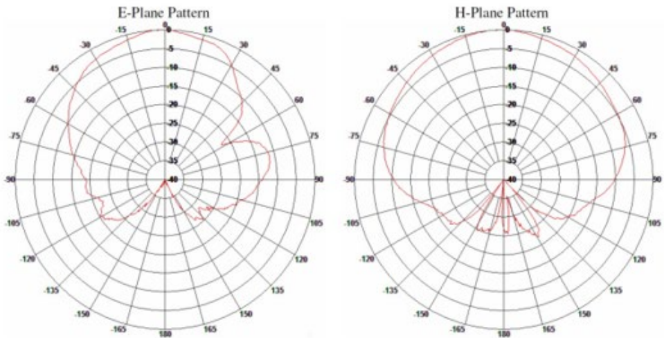
AIO-DD05120-RPSMA 2.5GHz
