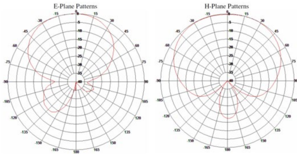
AIO-DD05120-RPSMA 5.5GHz
