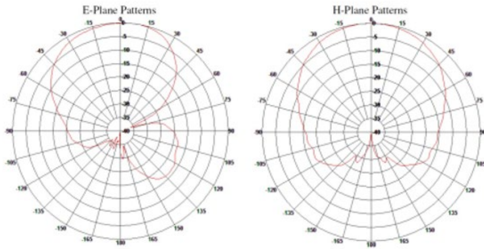
AIO-DD75060-RPSMA 2.4GHz
