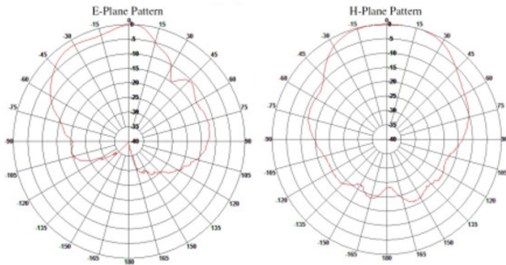
AIO-DD75060-RPSMA 5.5GHz
