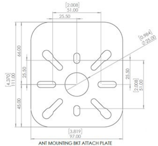
ANT MOUNTING BKT ATTACH PLATE
