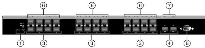
Figure 2 C5 Switch Back Panels
