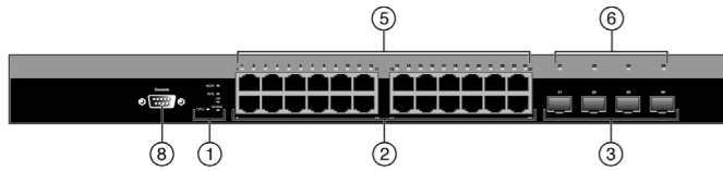
Figure 1 C5 Switch Front Panels
