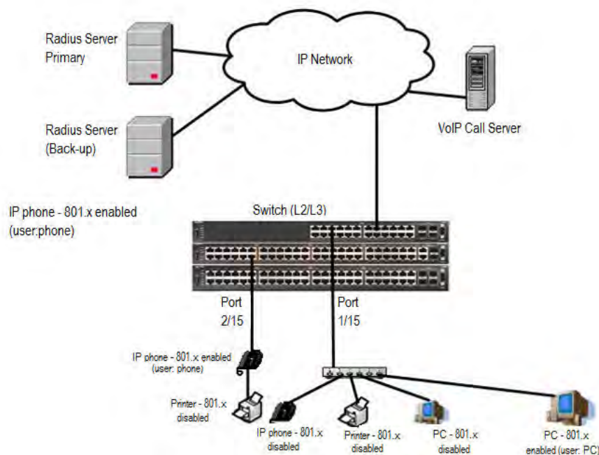
Figure 27: MHSA authentication mode (with or without RADIUS VLAN)
