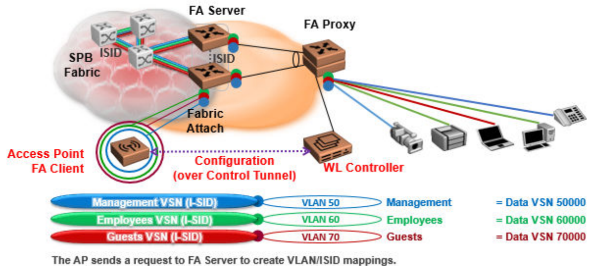
Figure 40: Fabric Attach for FA Clients — Automated Network Services
