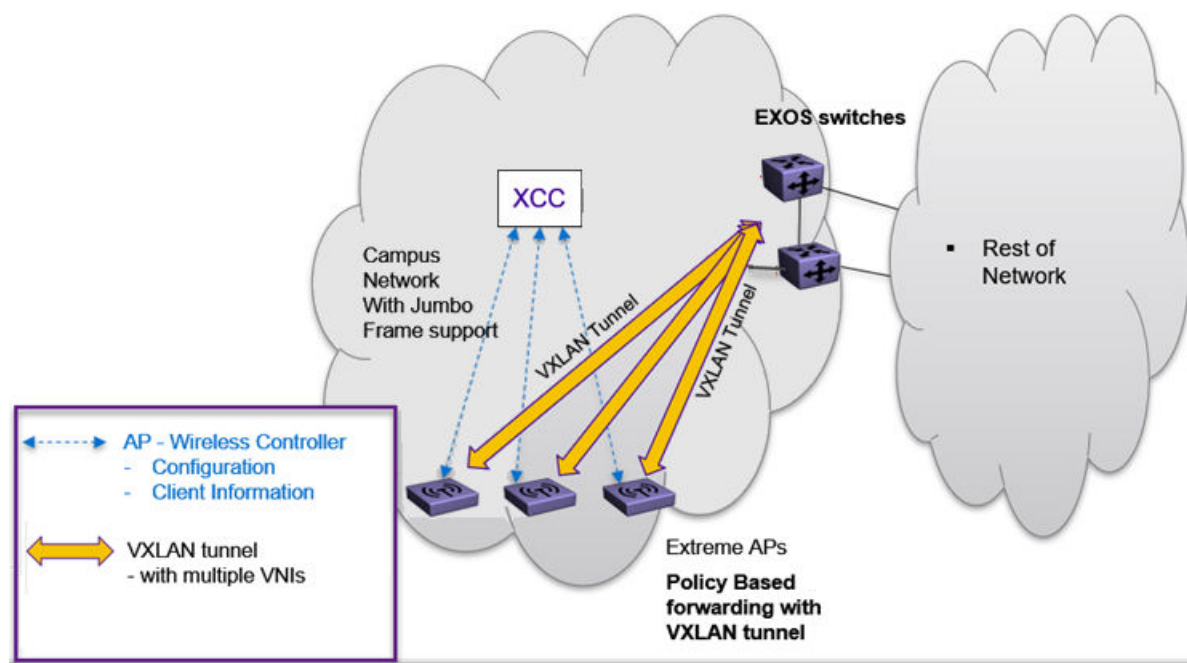
Figure 41: VxLAN Topology
