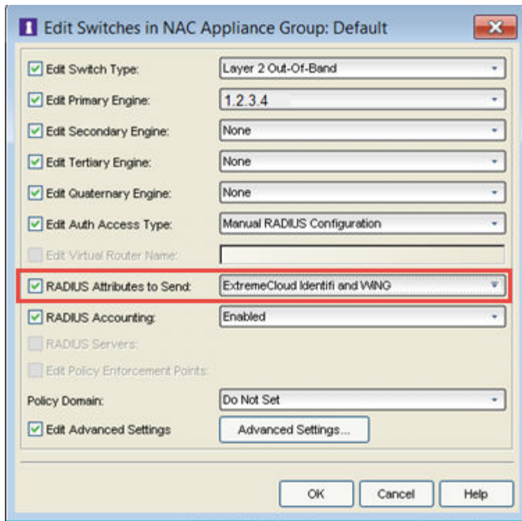
Figure 62: Edit Switch in NAC – Extreme Campus Controller
