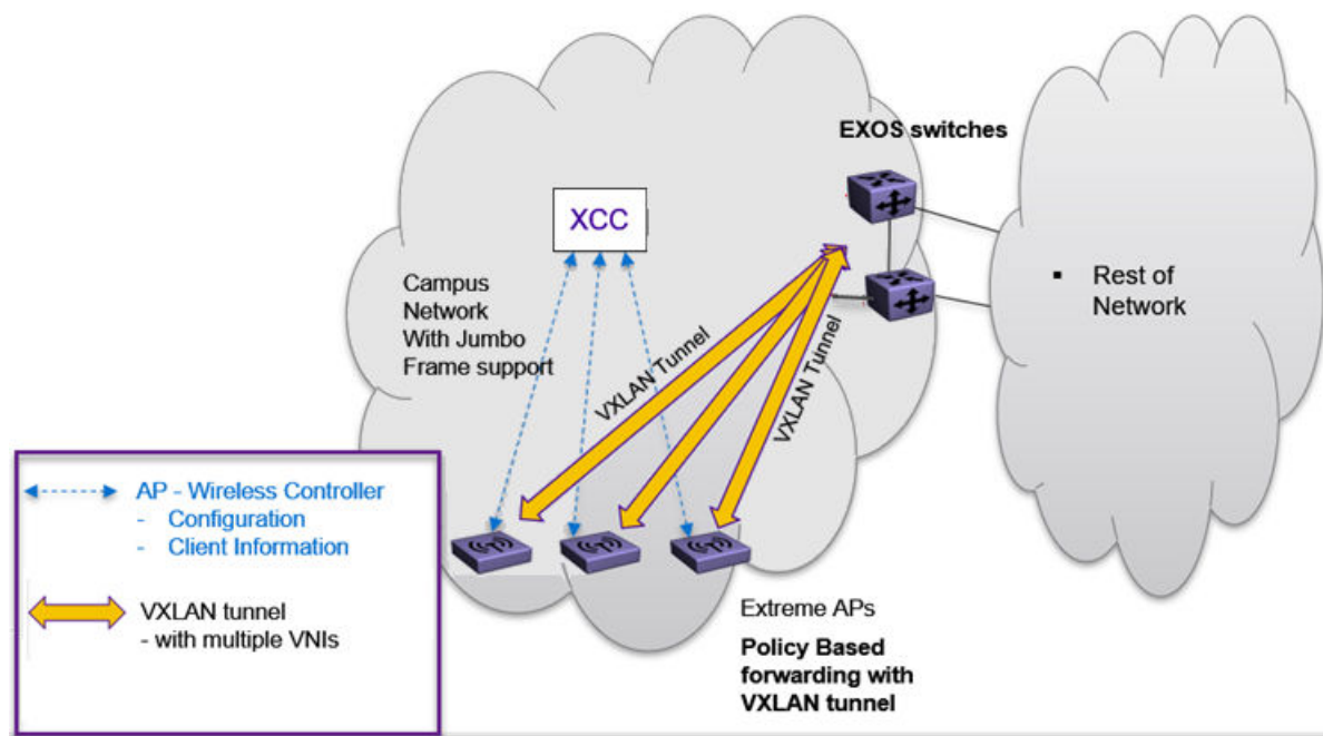
Figure 58: VxLAN Topology
