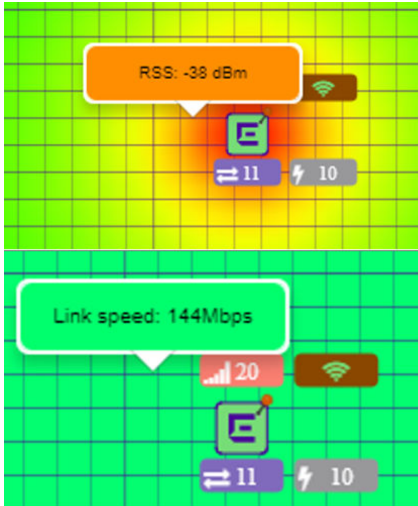
Figure 17: Push-Pin Reading for Heatmap Values
