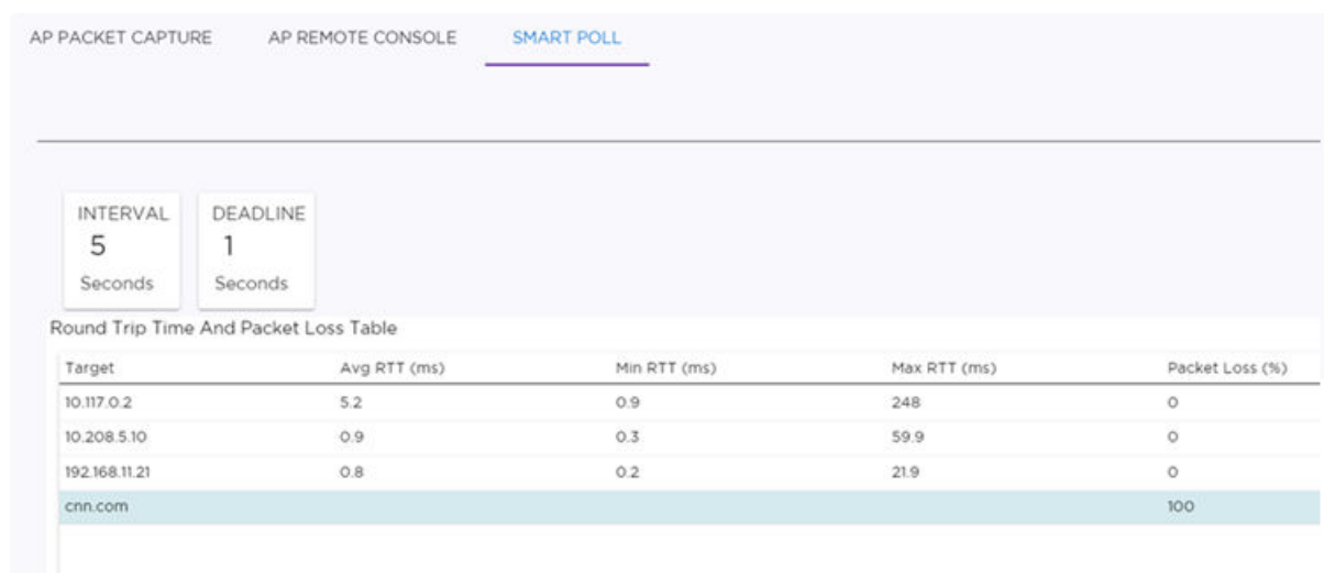
Figure 25: RTT and Packet Loss for Selected AP
