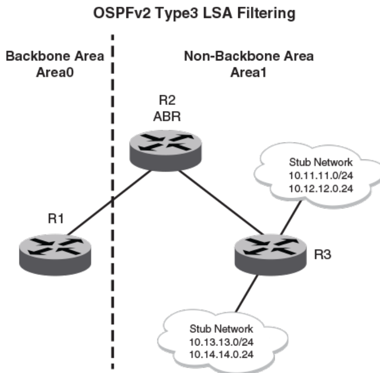
Figure 63: OSPFv2 type 3 LSA filtering
