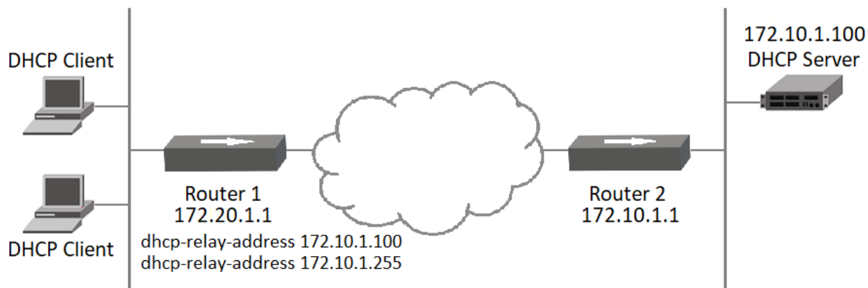
Figure 41: DHCP Relay Configuration
