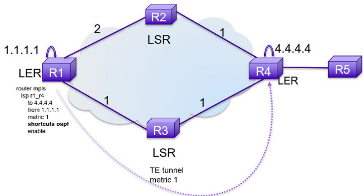
Figure 64: OSPF Shortcuts
