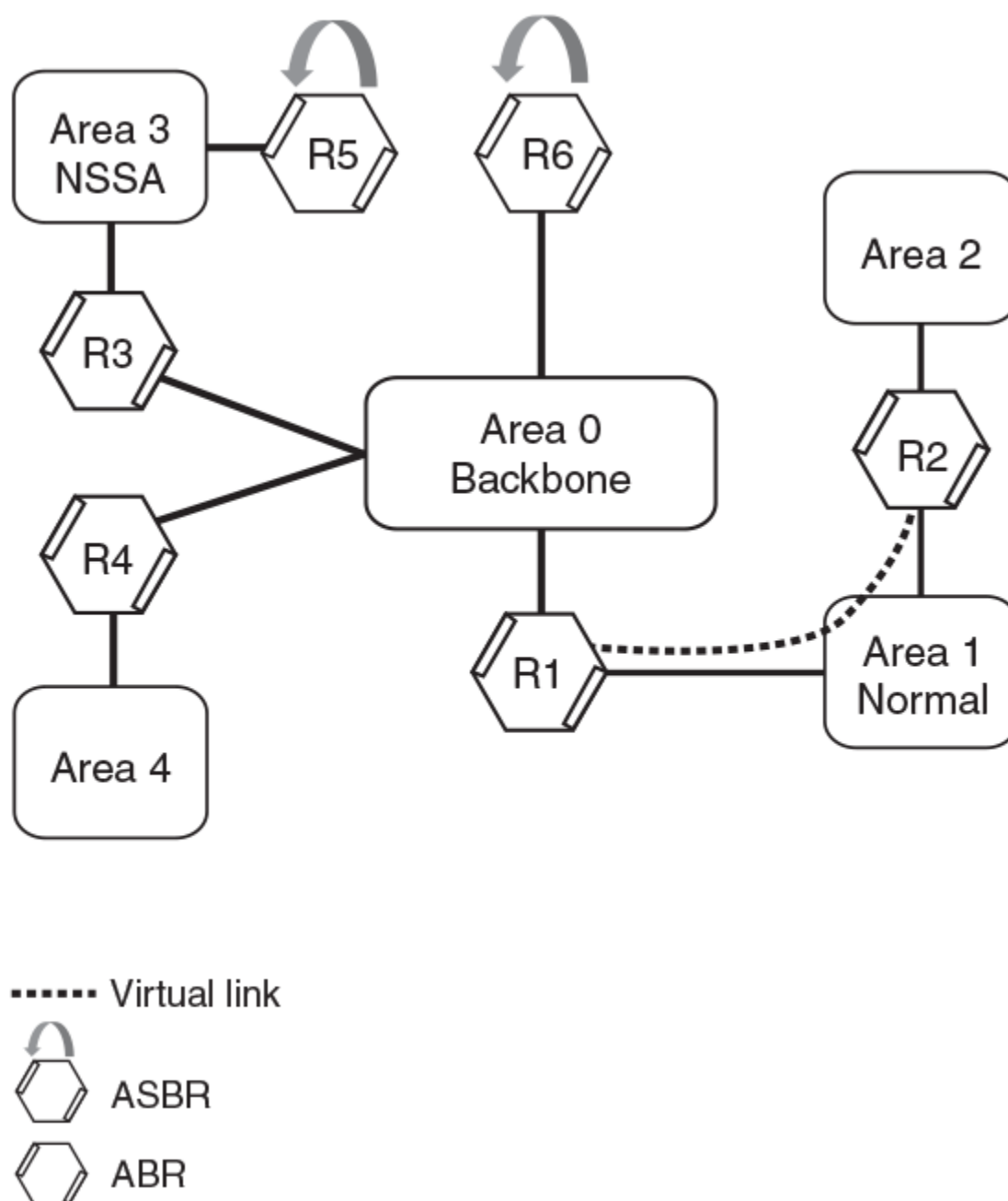
Figure 65: OSPFv3 virtual link
