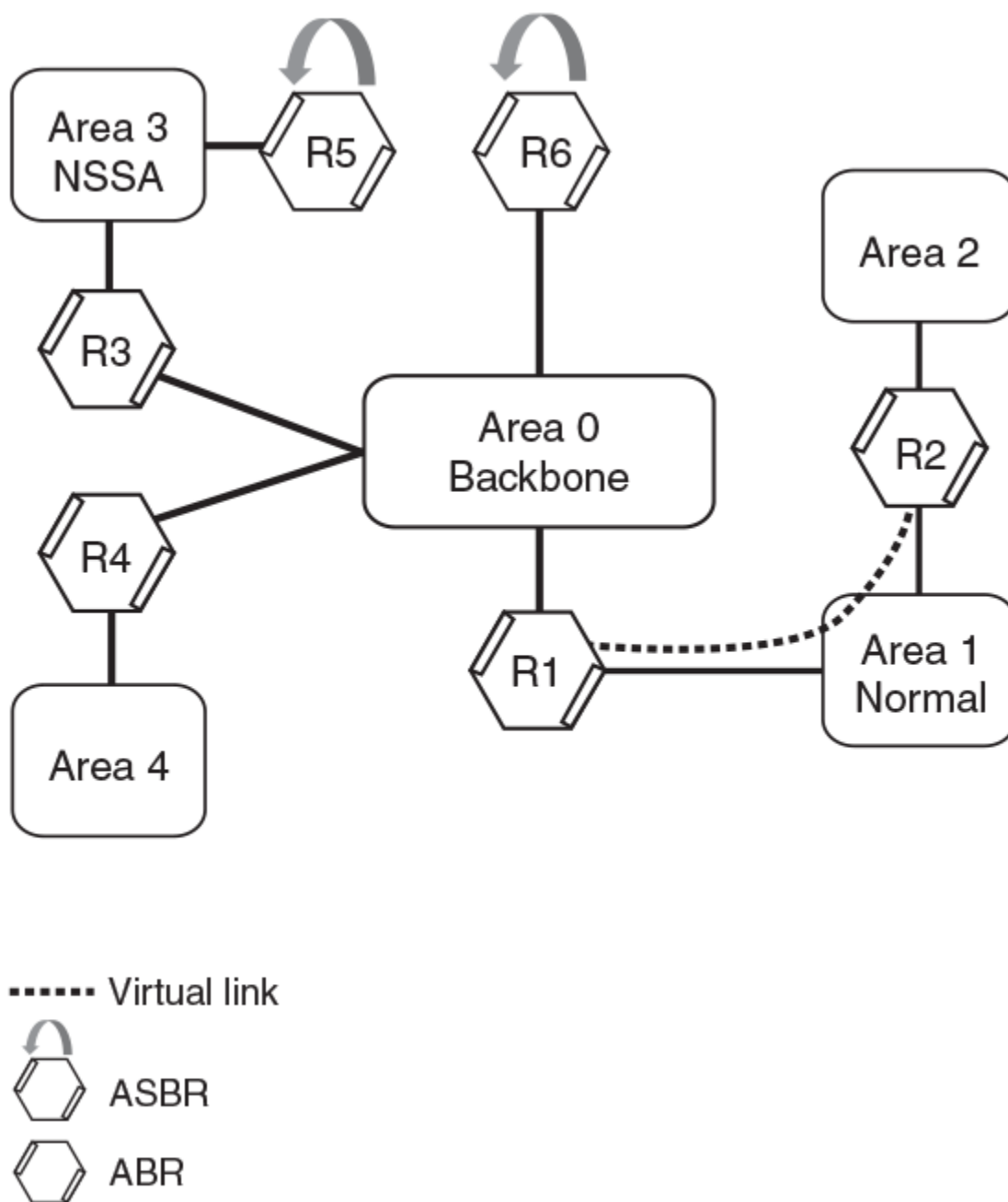
Figure 62: OSPFv3 virtual link
