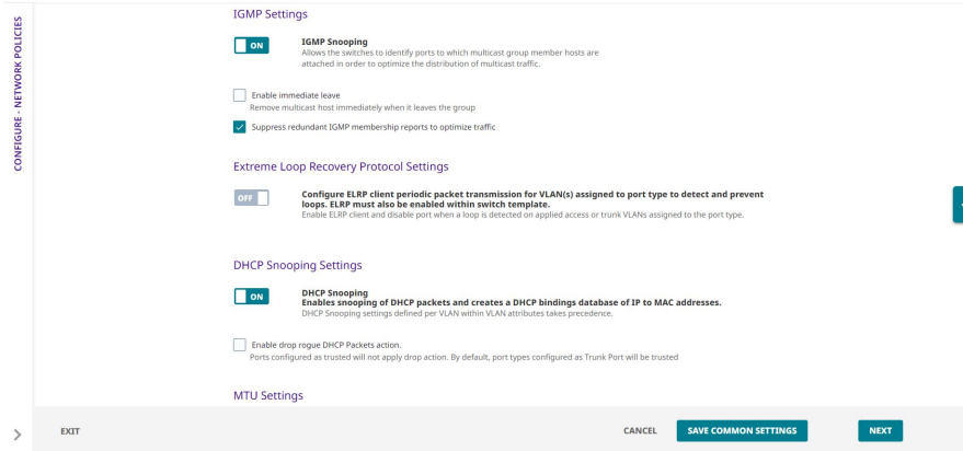
Figure 21: IGMP Snooping Network Policy
