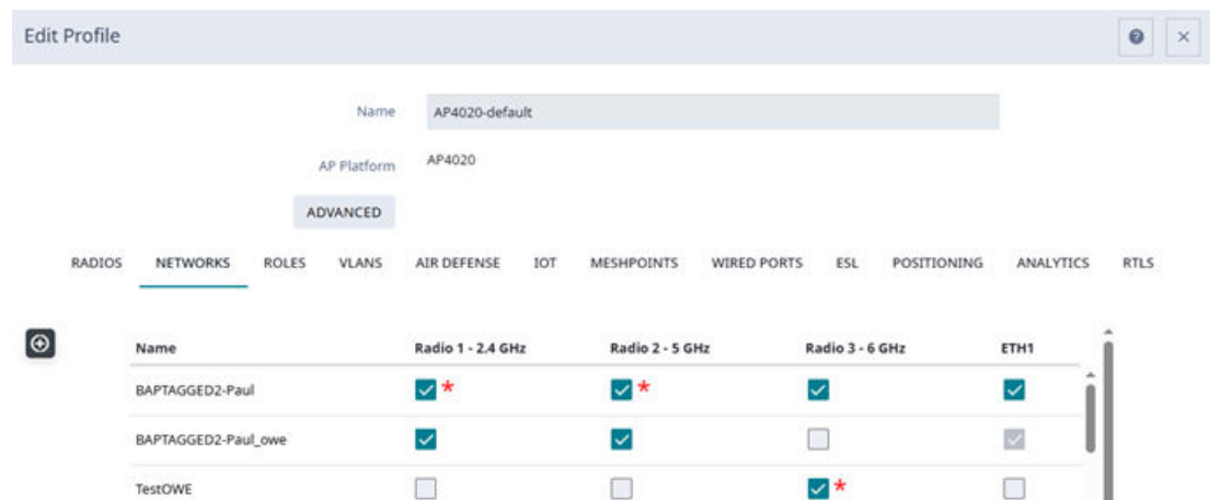
Figure 82: Configuration Profile Network Configuration – Client Bridge
