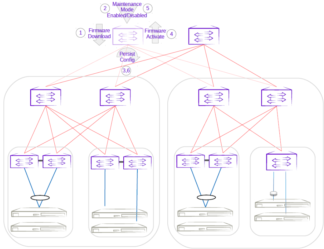
Figure 32: First super-spine firmware upgrade with maintenance mode
