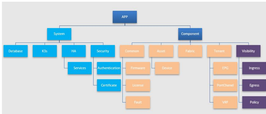
Figure 54: XCO Health Resource Hierarchy
