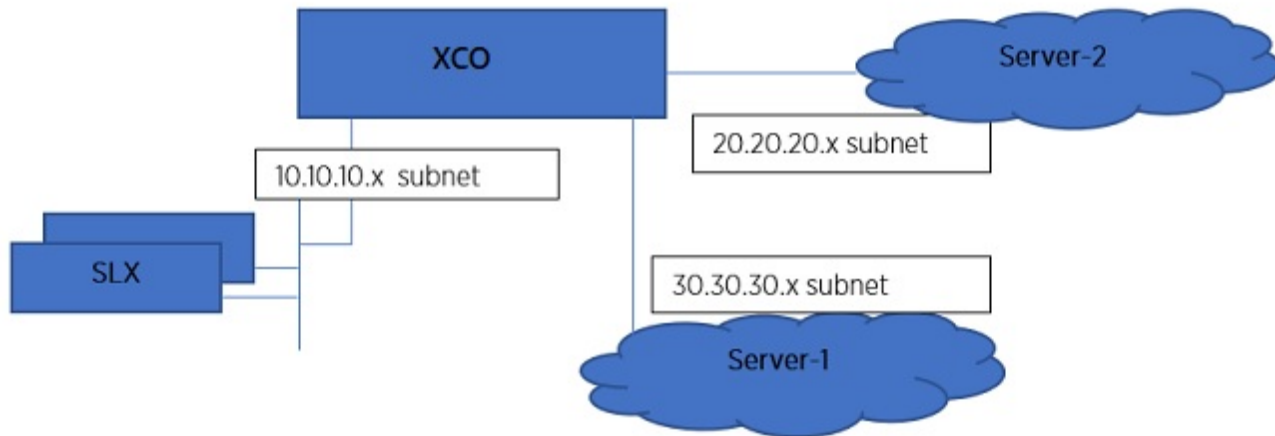
Figure 9: MMIP architecture
