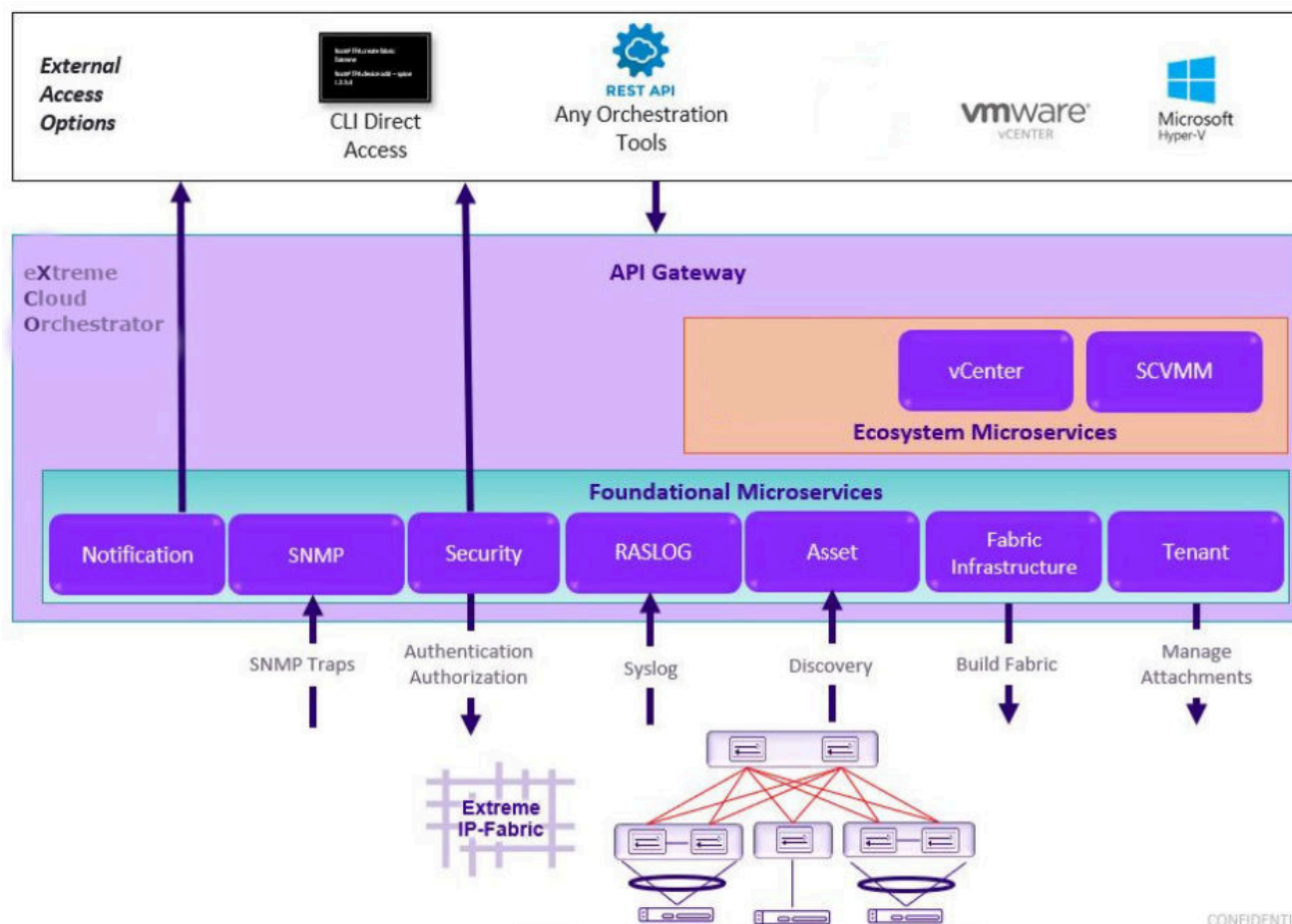
Figure 1: XCO orchestration
