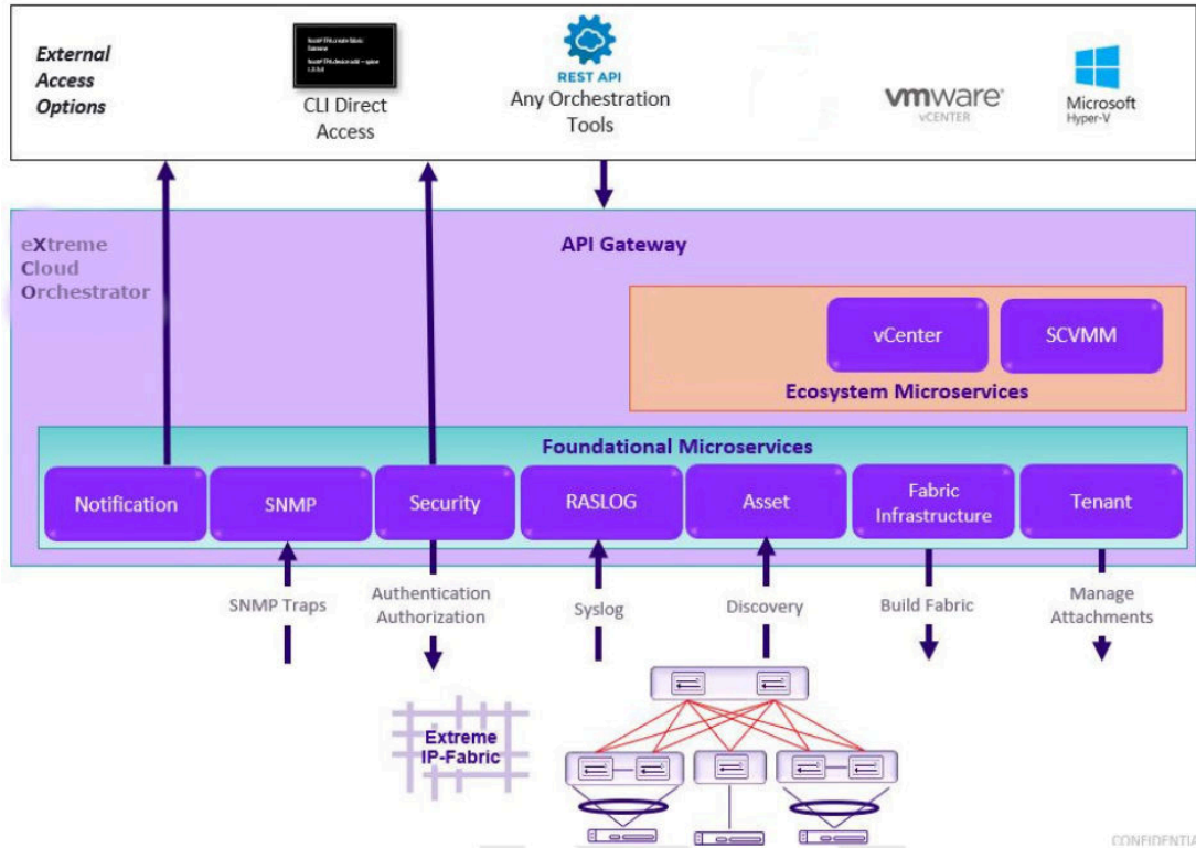
Figure 1: XCO Orchestration
