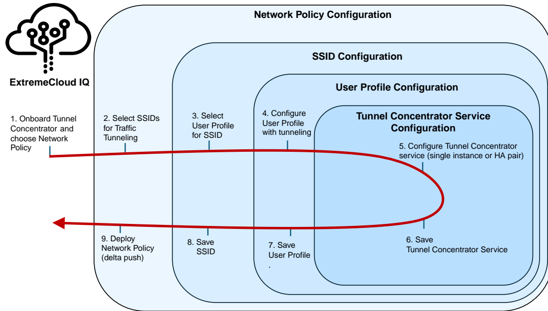
Figure 20: Tunnel Concentrator Configuration using Network Policy (ExtremeCloud IQ)
