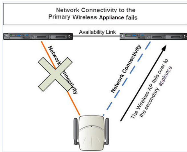
Figure 37: AP Fail Over When Connectivity to Primary Fails
