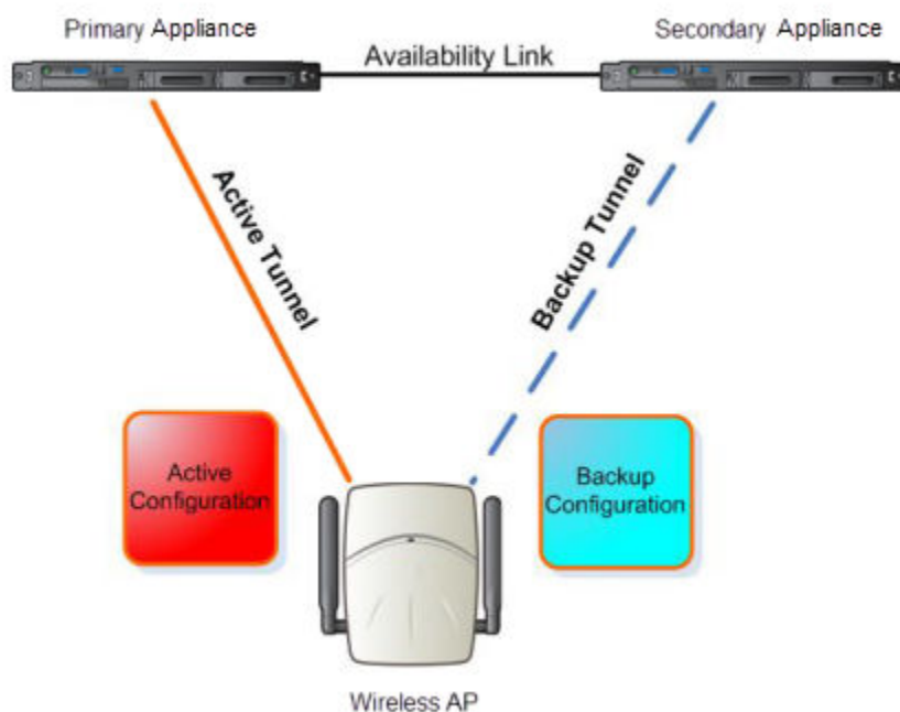
Figure 38: Session Availability Mode
