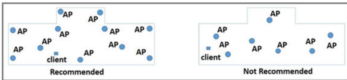
Figure 3: Recommended AP Placement
