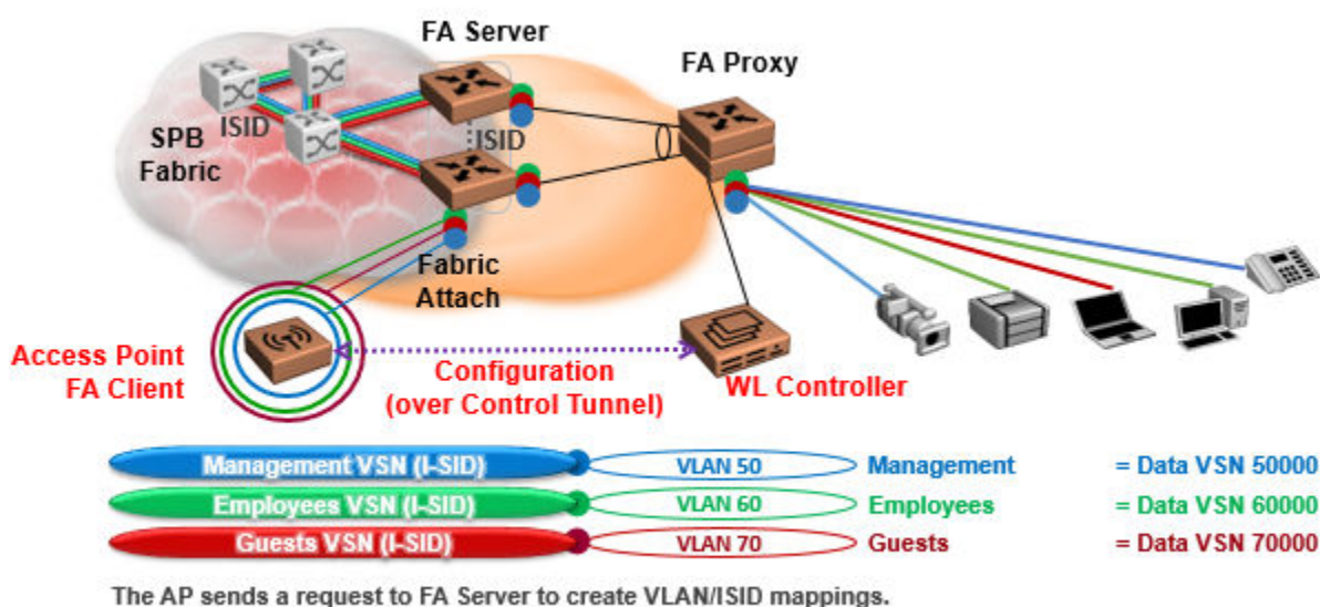
Figure 26: Fabric Attach for FA Clients — Automated Network Services
