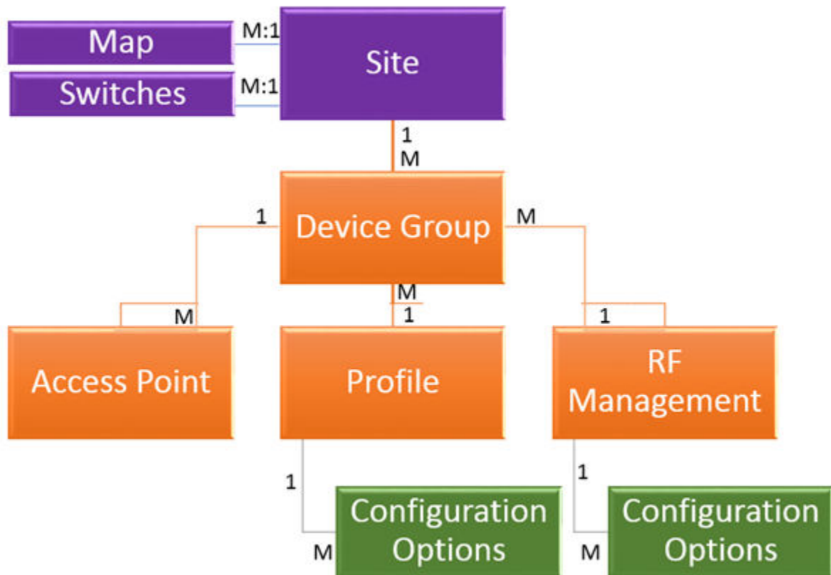
Figure 27: ExtremeCloud Appliance Component Relationship
