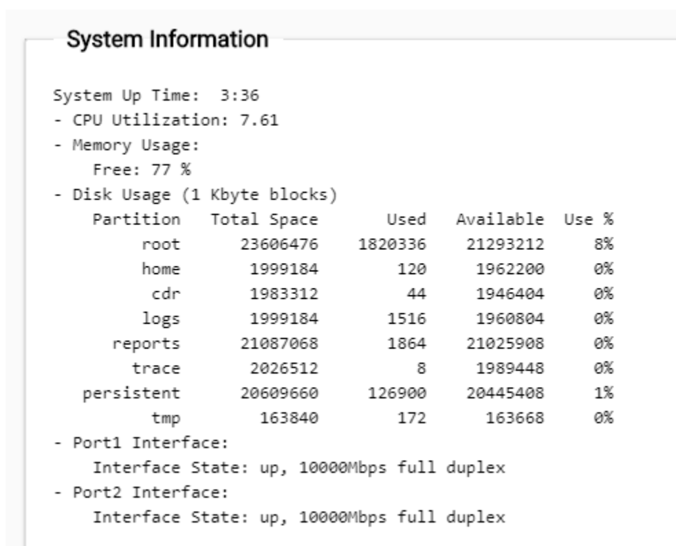
Figure 39: Example System Information
