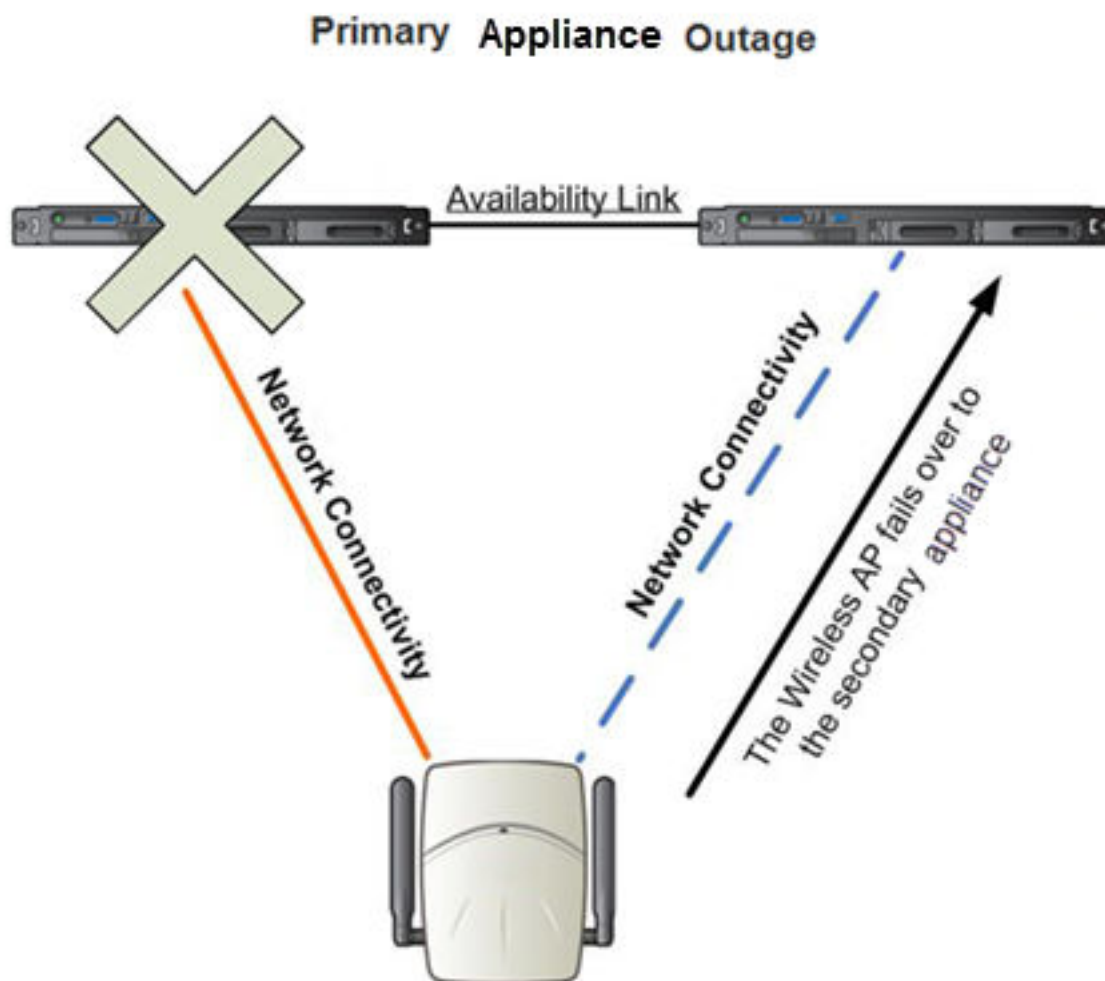
Figure 36: AP Fail Over When Primary Appliance Fails
