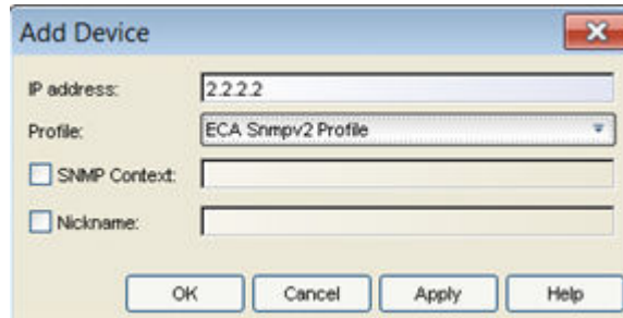
Figure 44: Add Device
