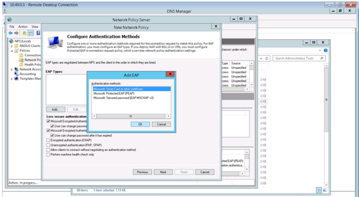
Figure 26: Add EAP
