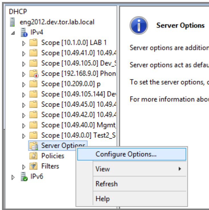
Figure 8: Configure Options
