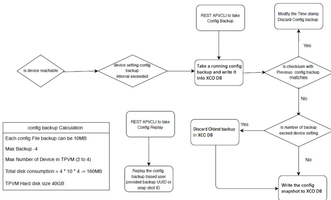
Figure 53: Workflow
