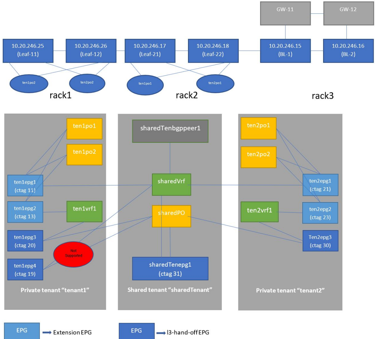
Figure 24: Shared VRF Configuration Overview
