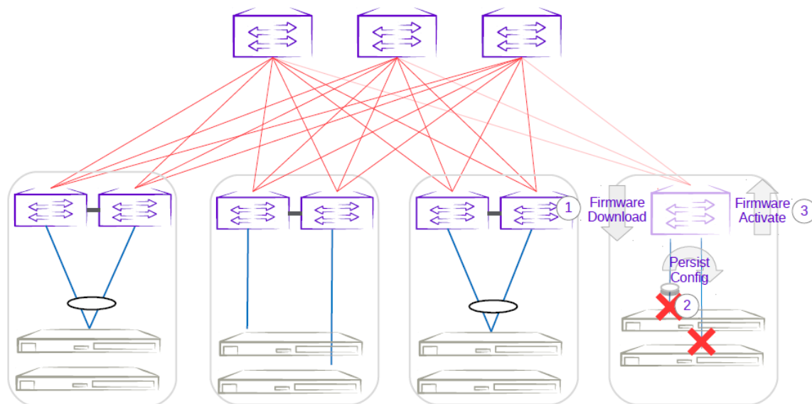
Figure 49: Single-leaf traffic loss
