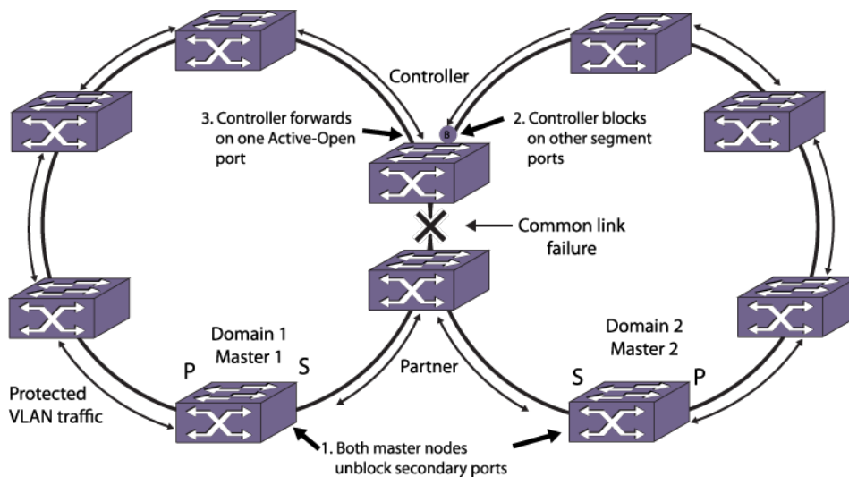
Figure 52: Common Link Failure
