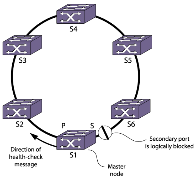
Figure 47: EAPS Operation
