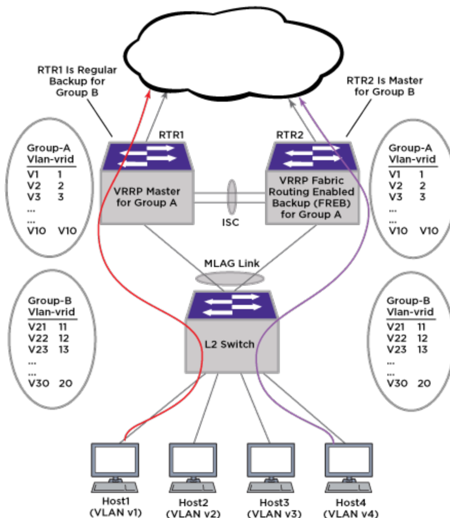
Figure 273: Example VRRP Group Configuration
