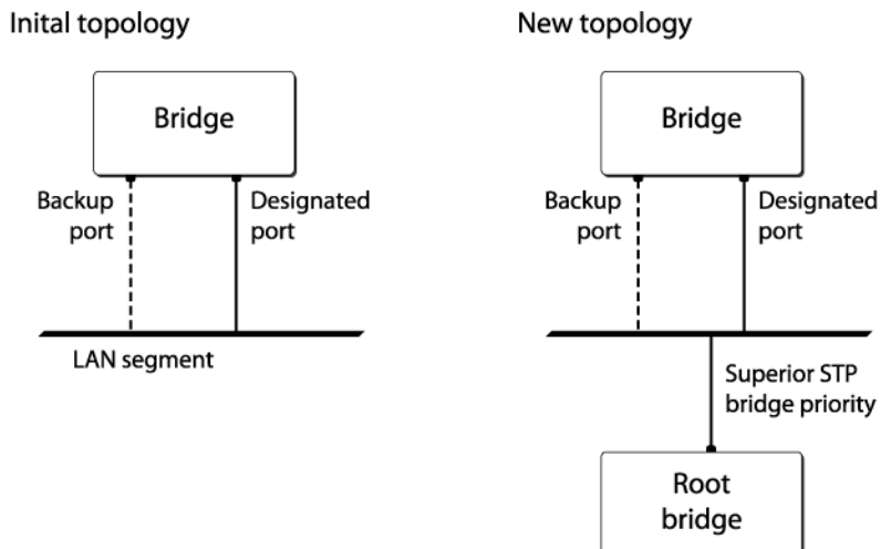
Figure 223: Example of Root Port Rapid Behavior
