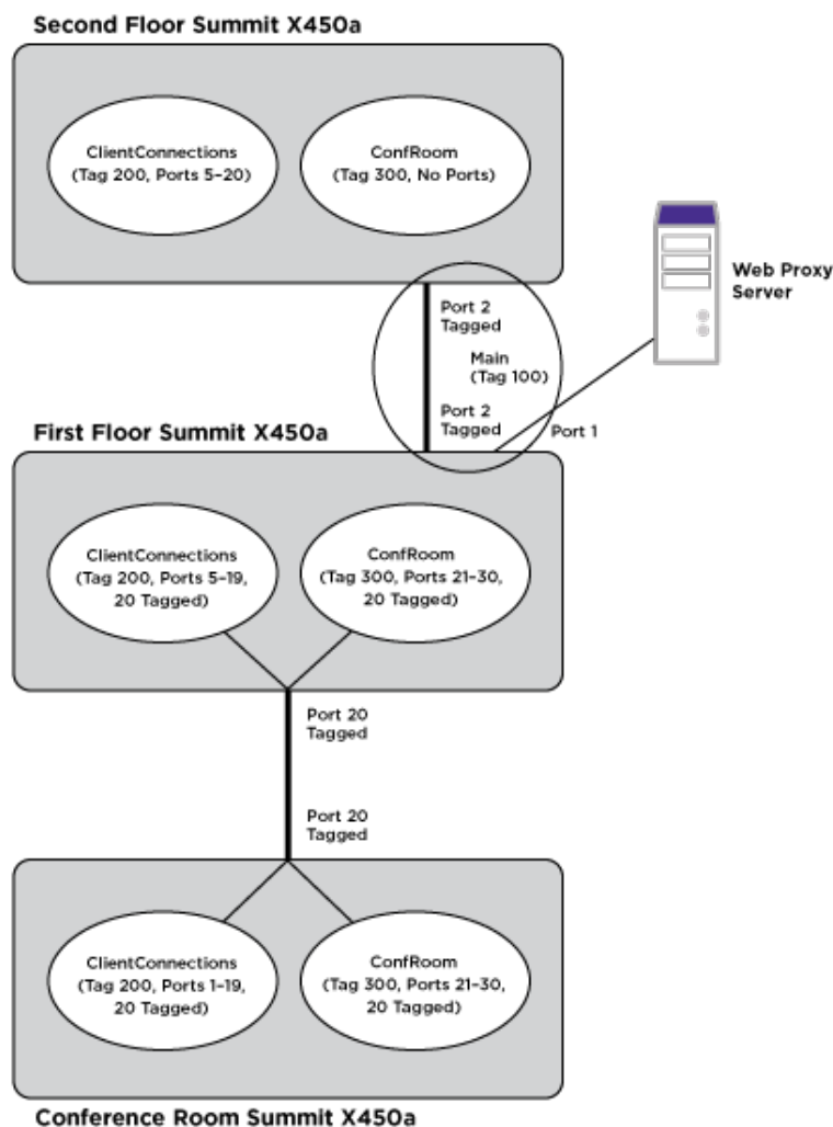
Figure 256: PVLAN Configuration Example 2
