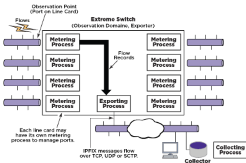
Figure 11: IPFIX Processes
