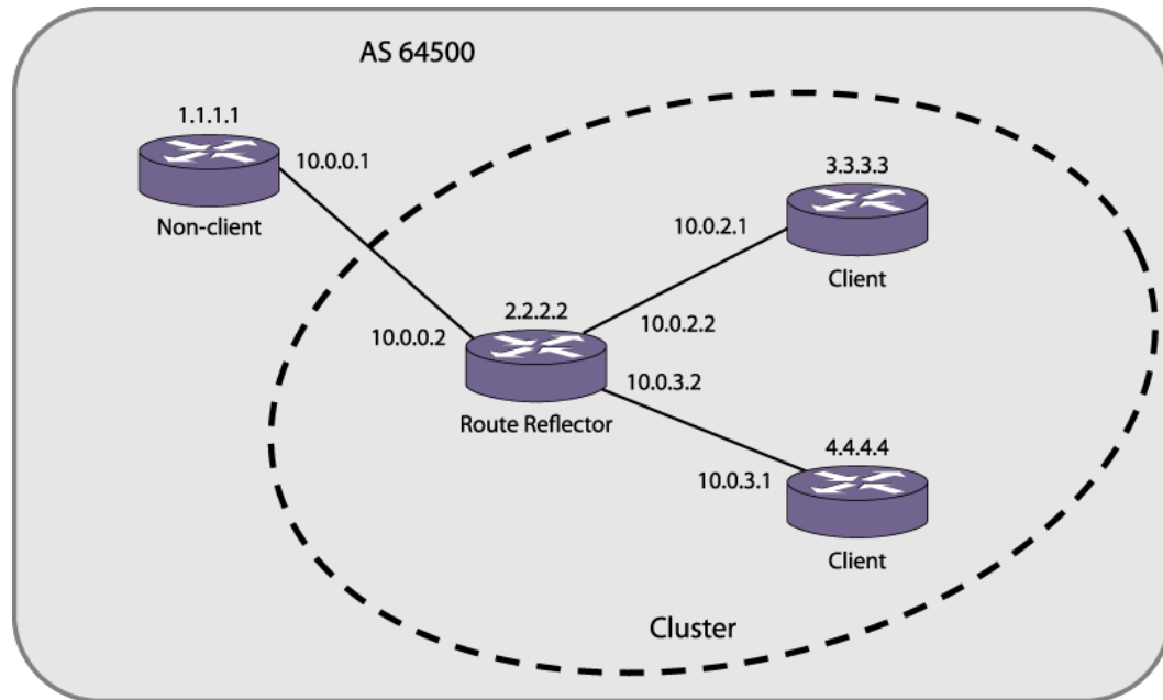
Figure 34: Route Reflectors
