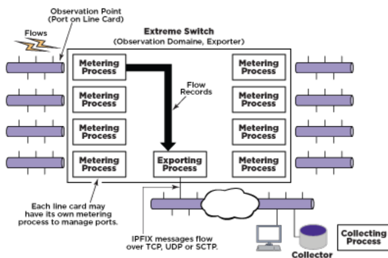
Figure 11: IPFIX Processes
