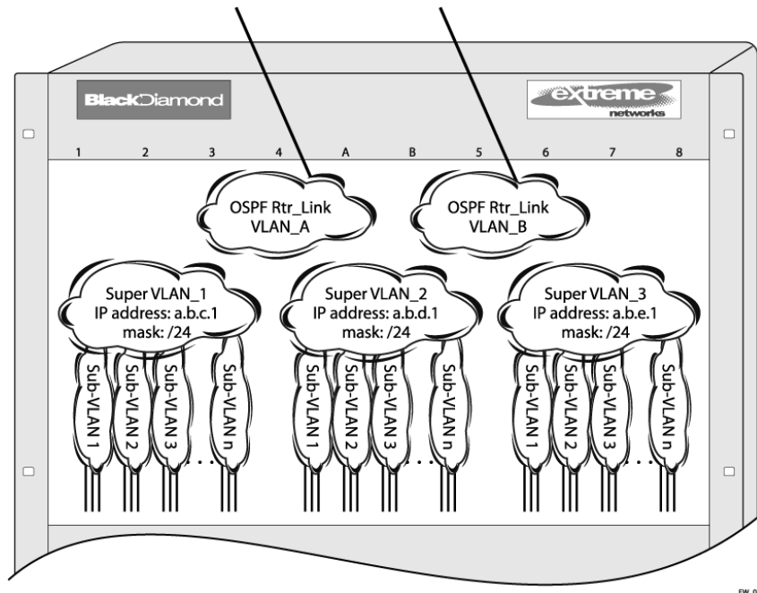
Figure 107: VLAN Aggregation
