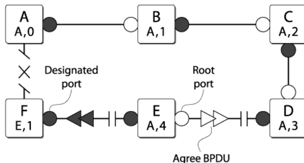
Figure 229: Communicating Port Status to Neighbors
