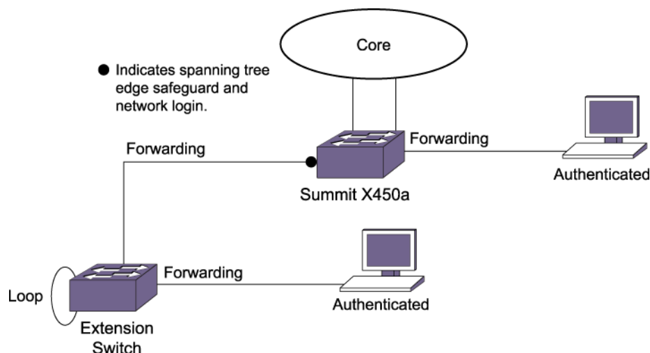
Figure 236: Traffic Monitoring on the Edge Side
