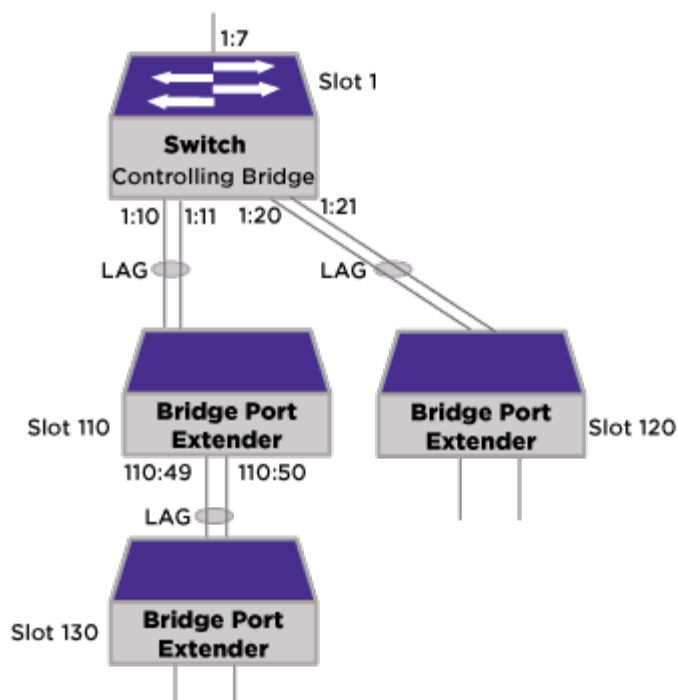
Figure 85: CB with Two-Tier BPEs Topology
