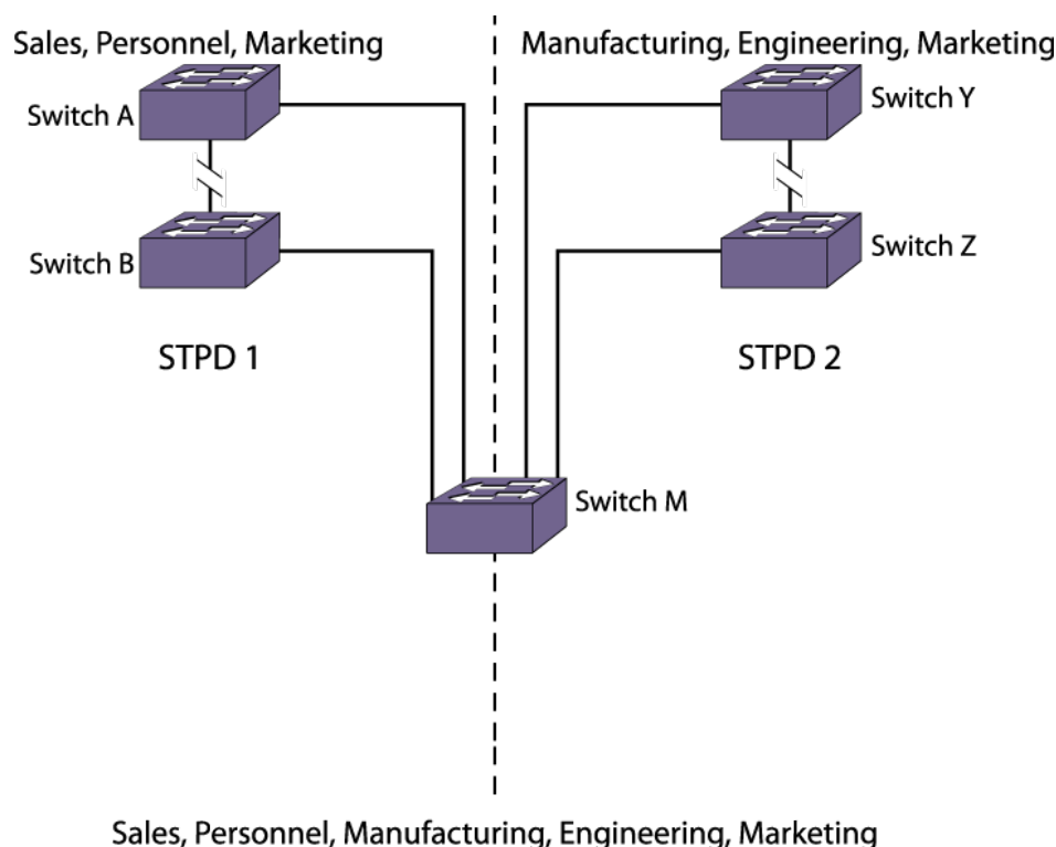
Figure 217: Multiple STPDs
