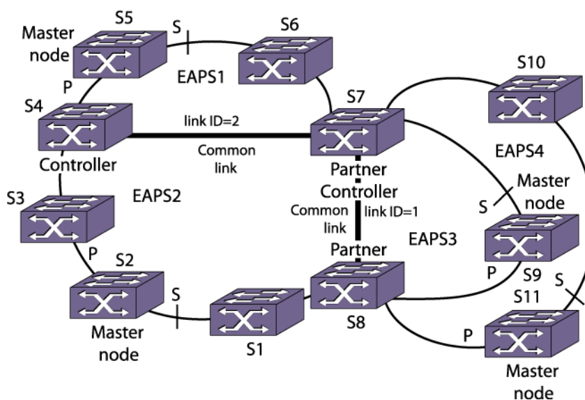
Figure 57: Right-Angle Topology
