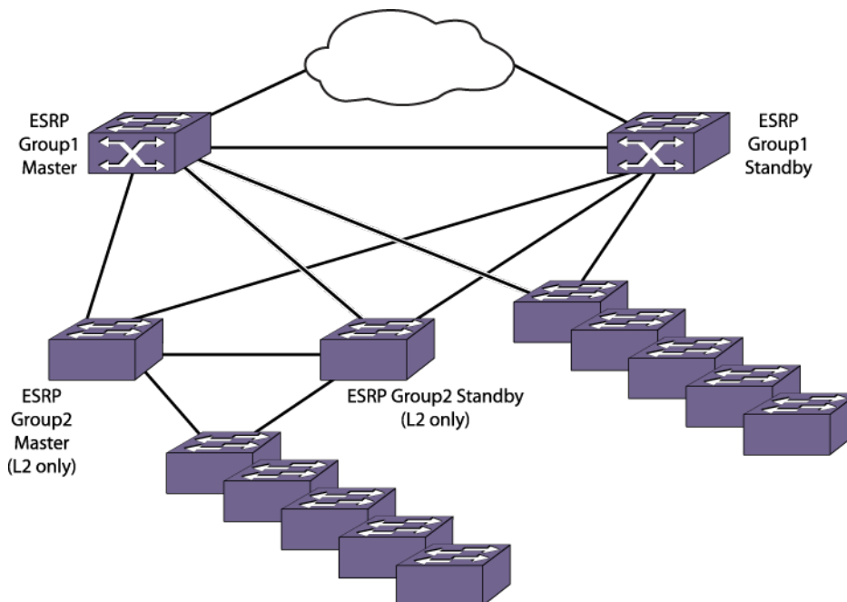
Figure 71: ESRP Groups
