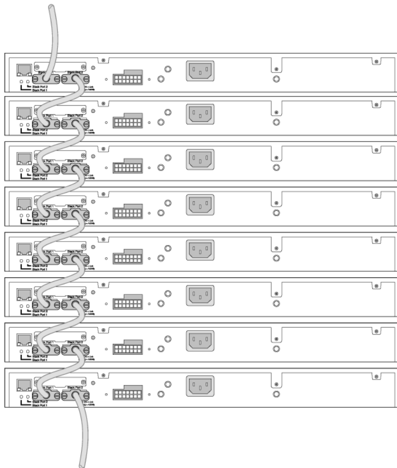
Figure 9: Daisy-Chain Topology
