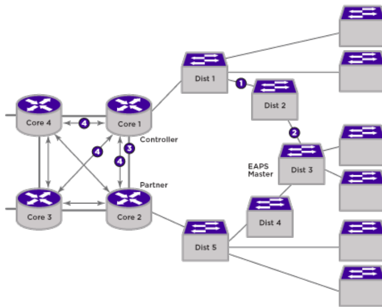
Figure 139: VPLS with Redundant EAPS Configuration Example
