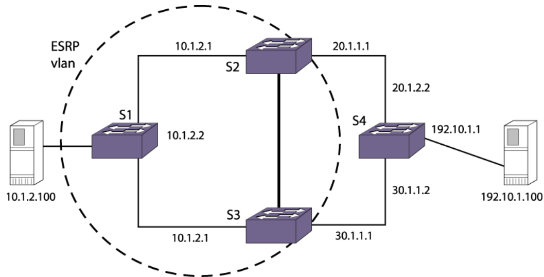
Figure 197: MAC Address Limits and VLANs Participating in ESRP
