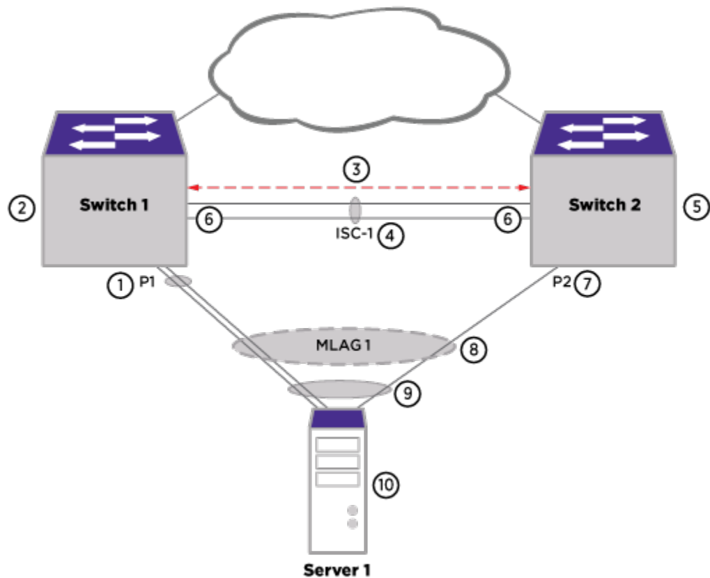
Figure 14: MLAG Elements
