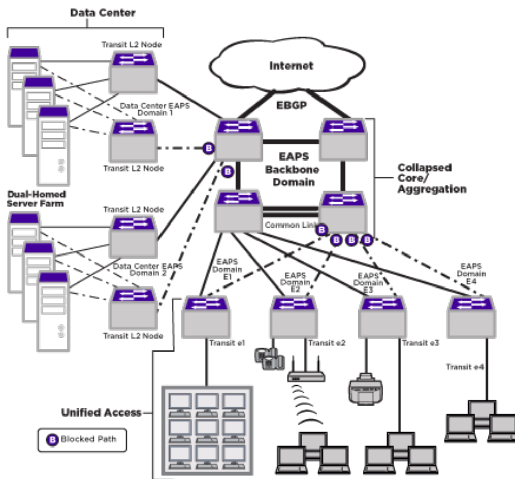
Figure 62: Extreme Networks EAPS Everywhere
