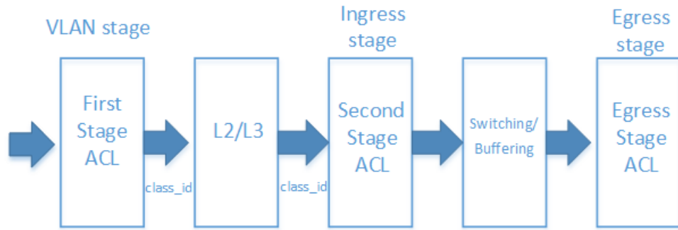
Figure 31: ACL Stages
