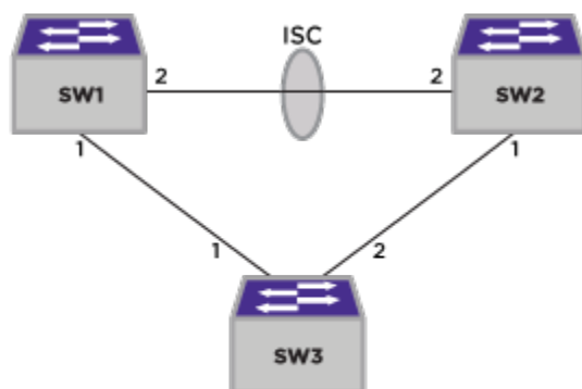
Figure 241: ELRP Egress Port Disable (1)
