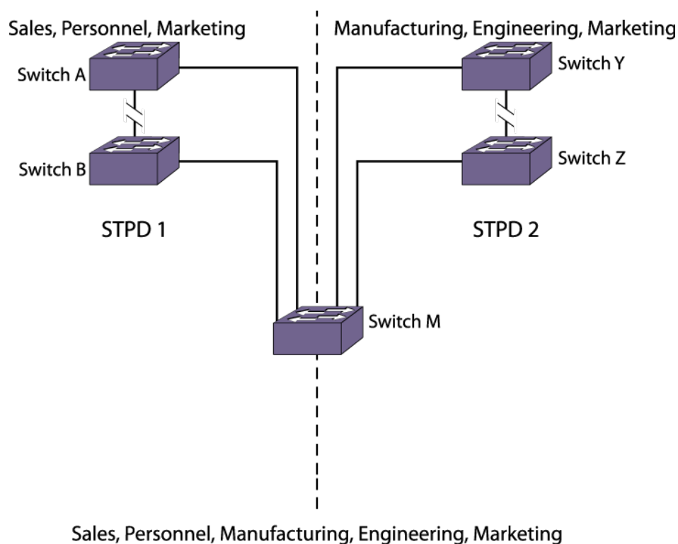
Figure 239: RSTP Example
