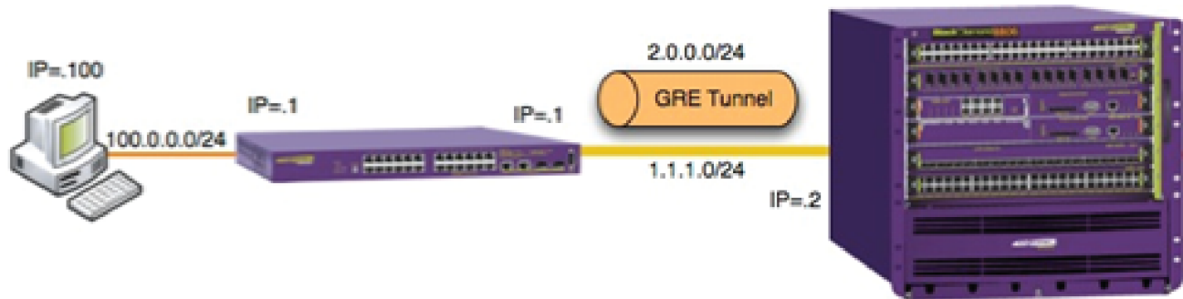
Figure 103: GRE Tunnel Configuration
