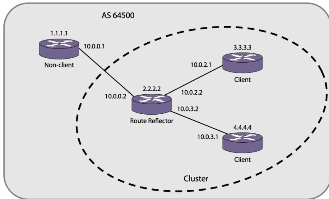
Figure 34: Route Reflectors
