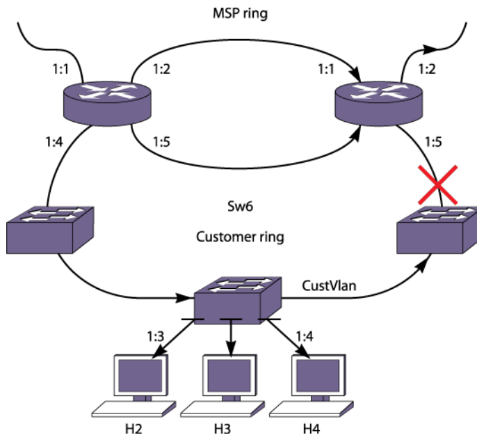
Figure 159: Inter-Multicast VLAN Forwarding
