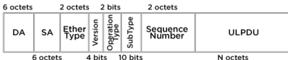
Figure 78: ECPDU Structure
