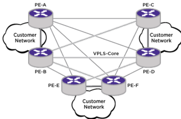
Figure 135: Example Protected Access VPLS Network
