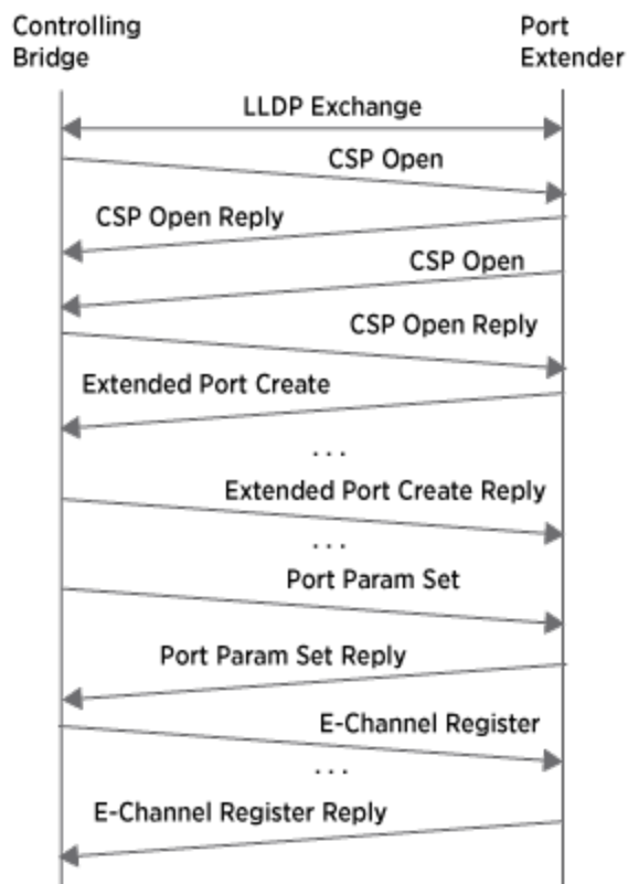
Figure 79: Example PE-CSP Protocol Exchange
