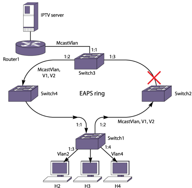
Figure 160: MVR on an EAPS Ring
