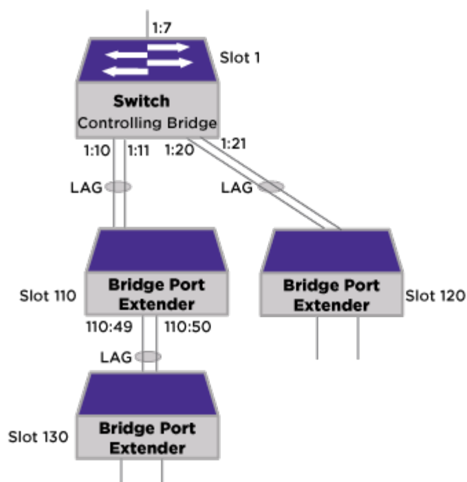
Figure 87: CB with Two-Tier BPEs Topology
