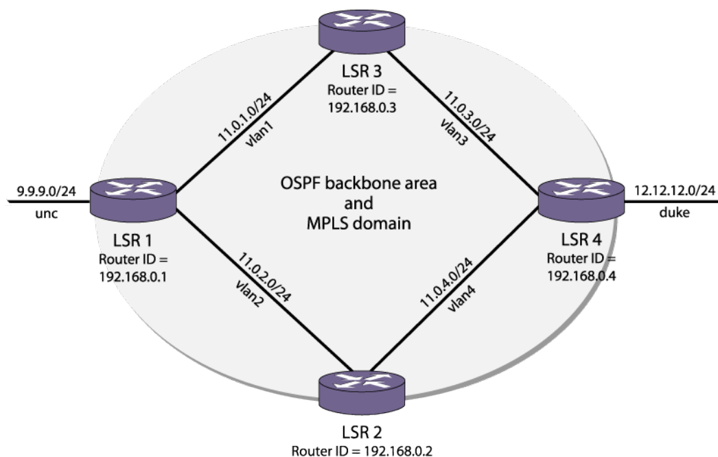
Figure 145: MPLS Configuration Example
