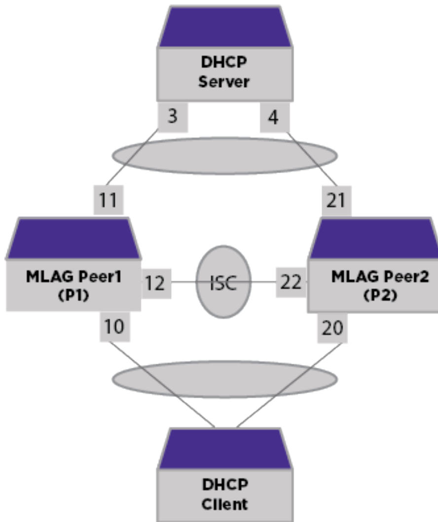
Figure 202: MLAG Topology
