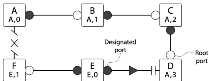
Figure 227: Communicating New Root Bridge Status to Neighbors
