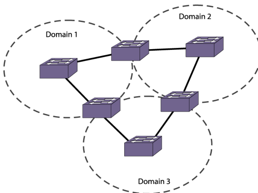
Figure 222: Looped VLAN Topology
