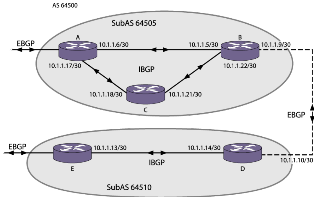
Figure 35: Routing Confederation
