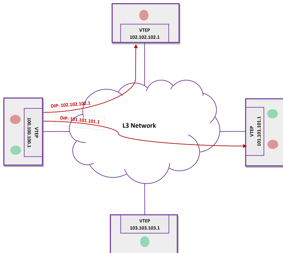
Figure 277: Head-end Replication
