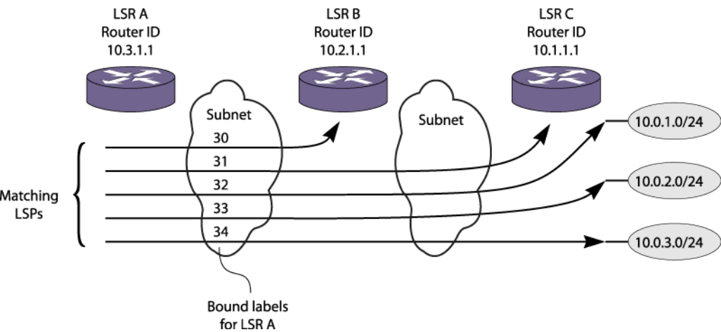
Figure 132: Matching and Calculated LSP Next Hops
