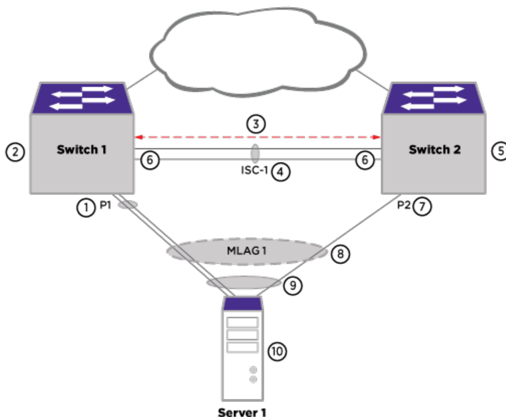
Figure 14: MLAG Elements
