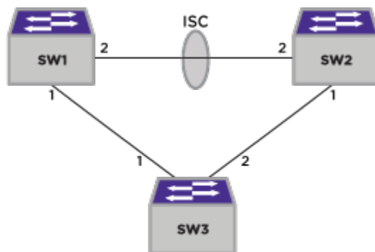
Figure 241: ELRP Egress Port Disable (1)
