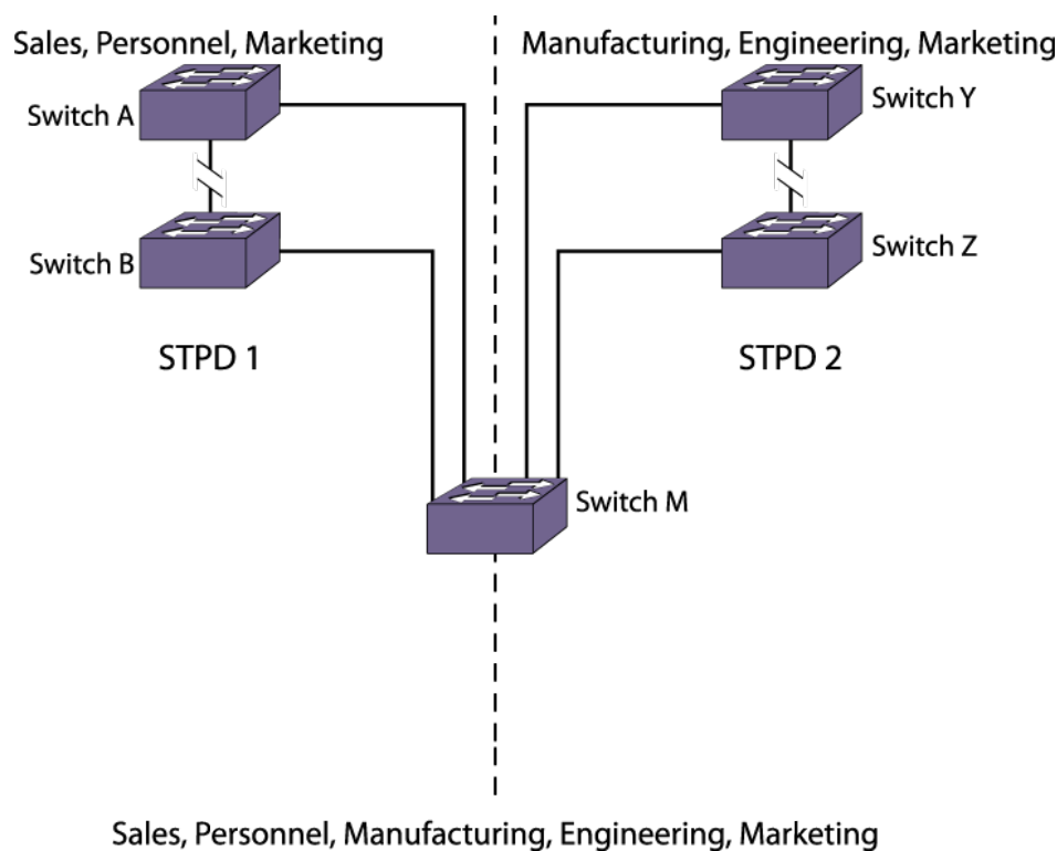
Figure 217: Multiple STPDs
