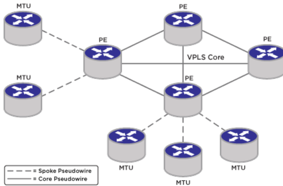
Figure 133: Example H-VPLS Network
