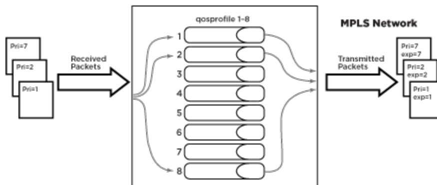
Figure 144: Mapping Dot1p to EXP Bits
