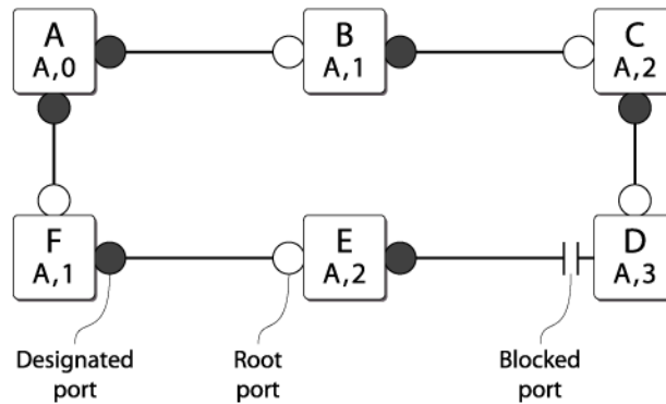
Figure 224: Initial Network Configuration
