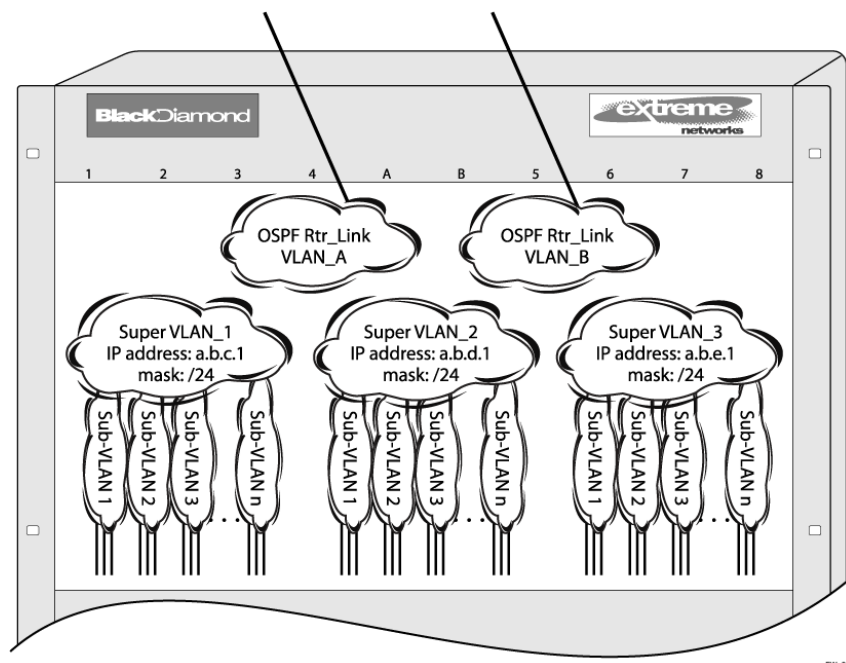
Figure 107: VLAN Aggregation
