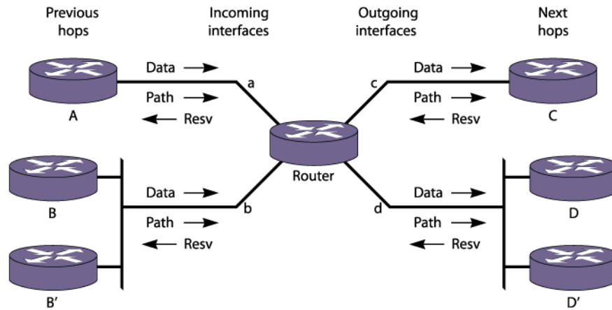
Figure 141: RSVP Messages
