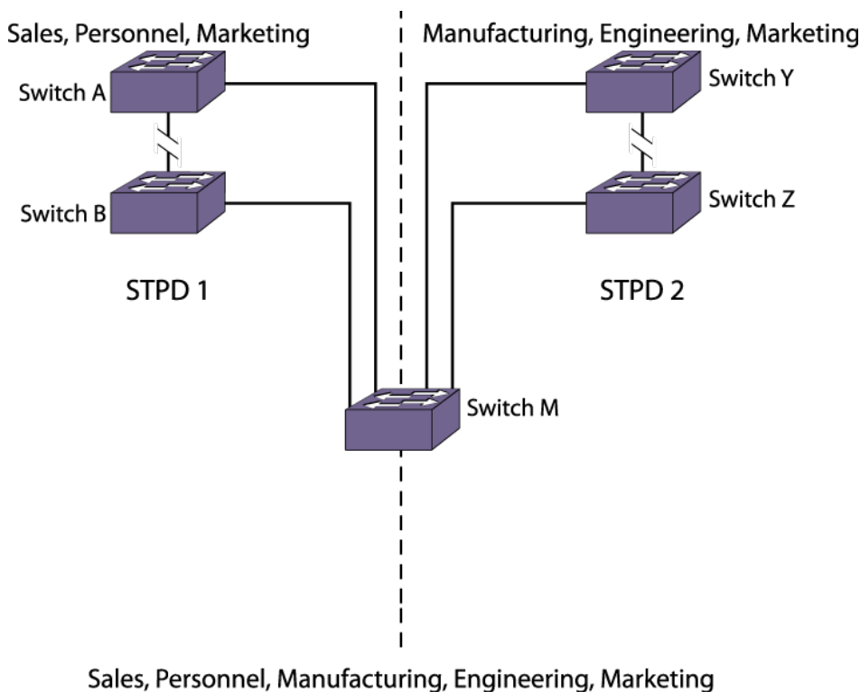
Figure 239: RSTP Example
