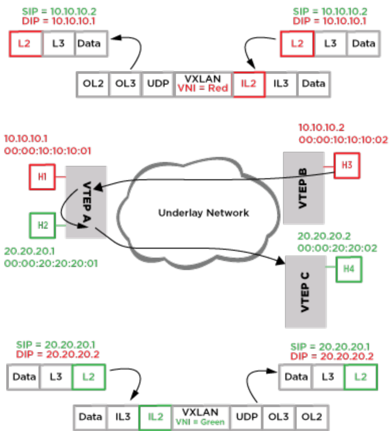
Figure 276: Routing in and out of a Tunnel
