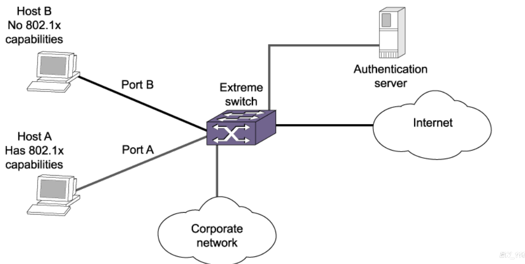
Figure 163: Guest VLAN for Network Login
