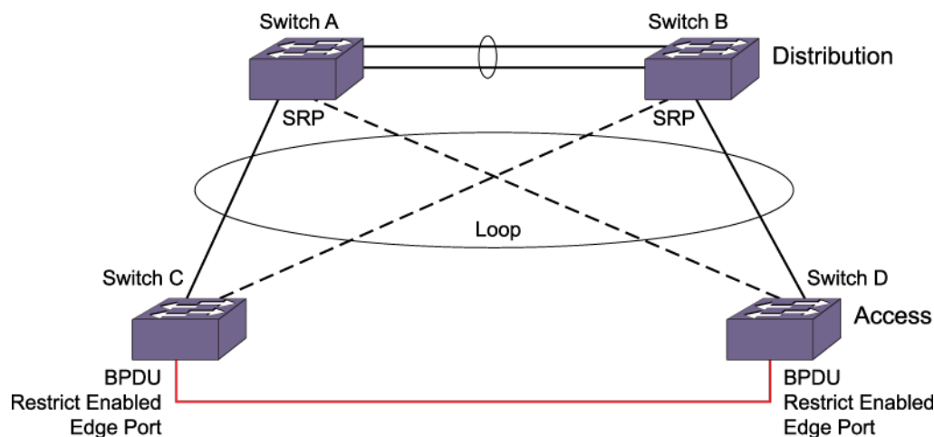
Figure 216: BPDU Restrict
