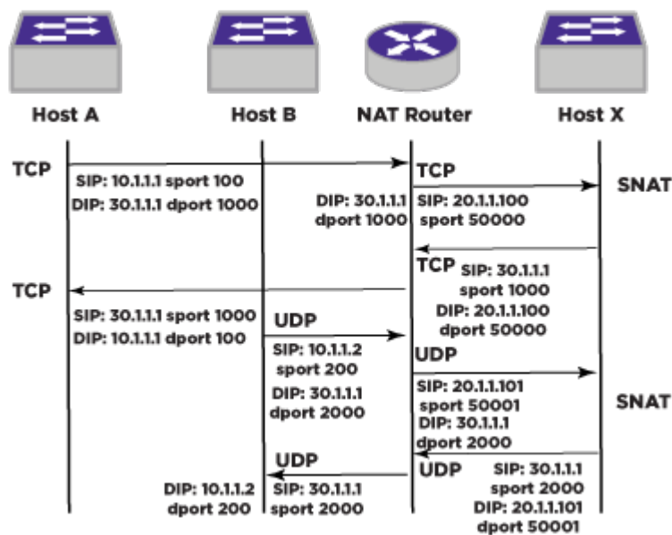
Figure 110: NAPT Example
