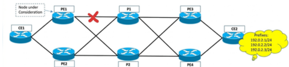
Figure 8: BGP PIC core node failure
