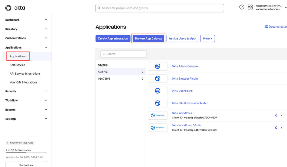
Figure 12: Applications Menu
