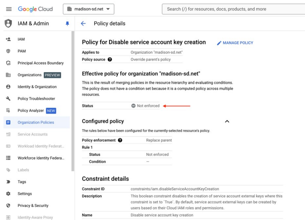
Figure 9: Successful Configuration
