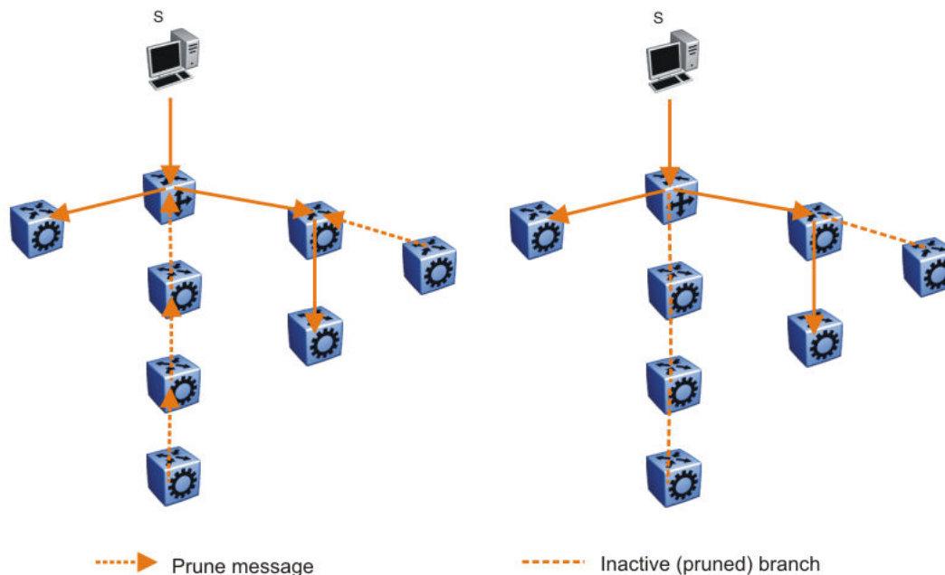
Figure 119: Pruning routers from a distribution tree
