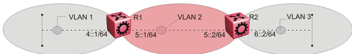
Figure 157: IPv6 routing between VLANs
