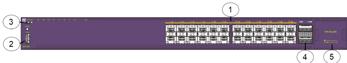
Figure 281: 5520-24X
