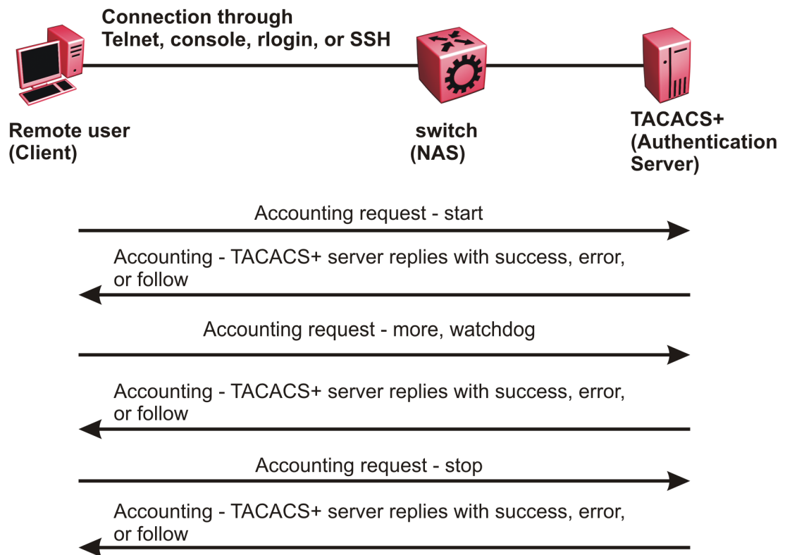
Figure 234: Accounting process
