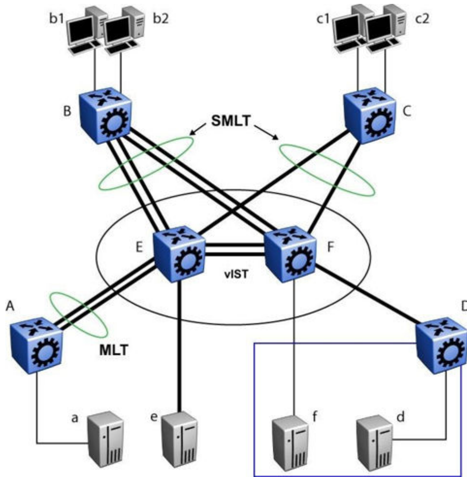
Figure 176: SMLT aggregation switches and operations
