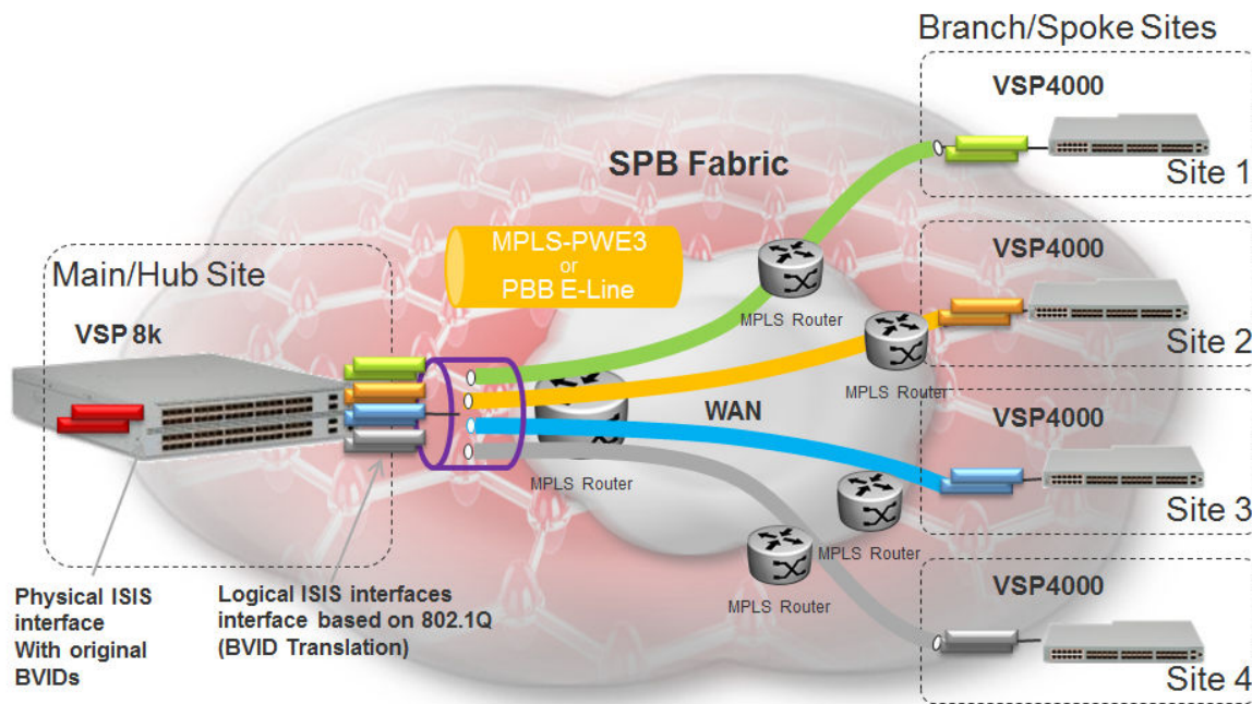
Figure 65: Fabric Extend Pseudowire Deployment Option
