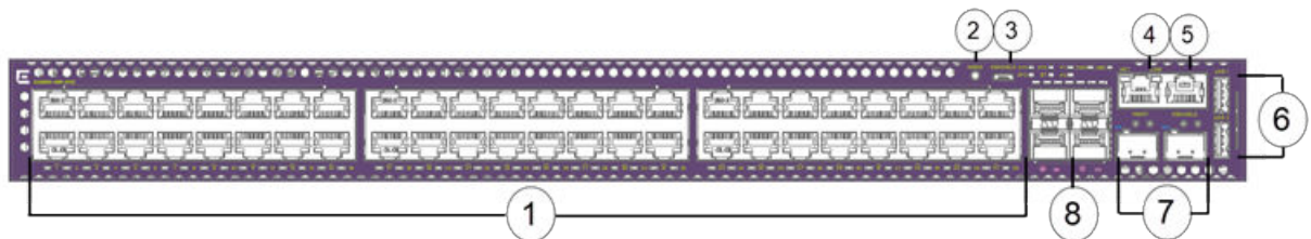
Figure 275: 5420M-48W-4YE Front Panel
