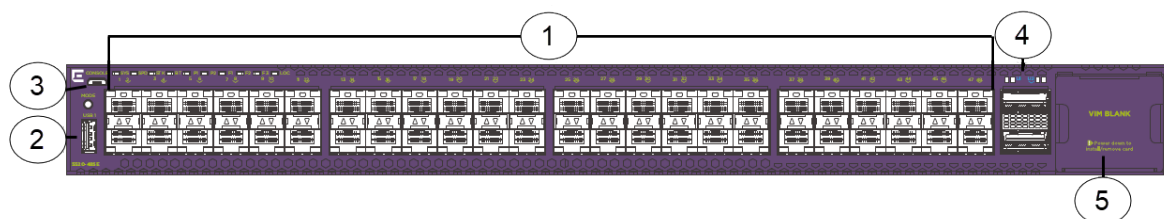
Figure 282: 5520-48SE
