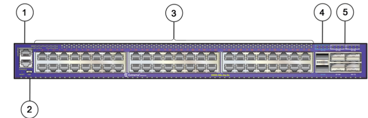
Figure 1 X690 Series Switch: Front Panel
