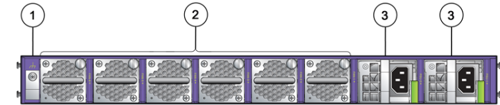
Figure 2 X690 Series Switch: Rear Panel
