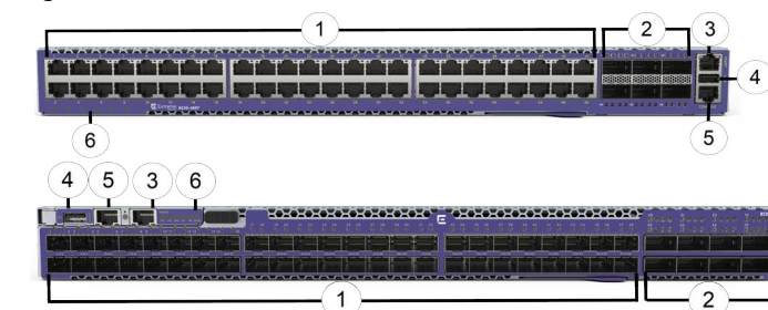
Figure 1 8520 Series Switches: Front Panels
