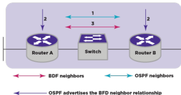
Figure 175: Basic Operational Flow of OSPFv3 BFD
