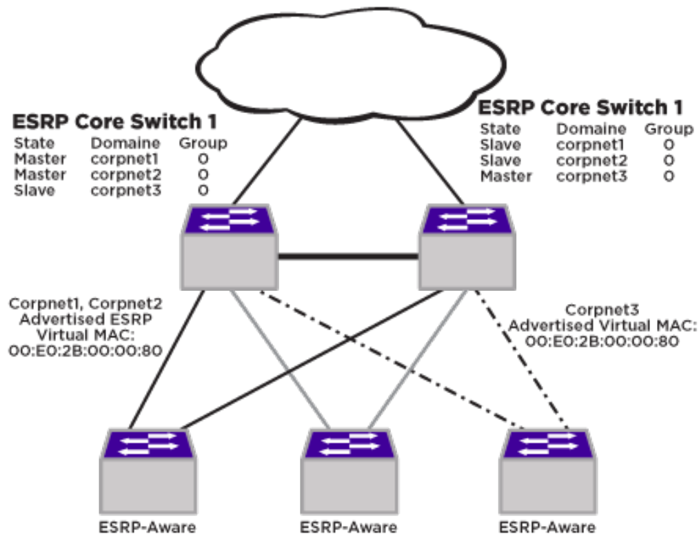
Figure 63: Example of a Basic ESRP Topology
