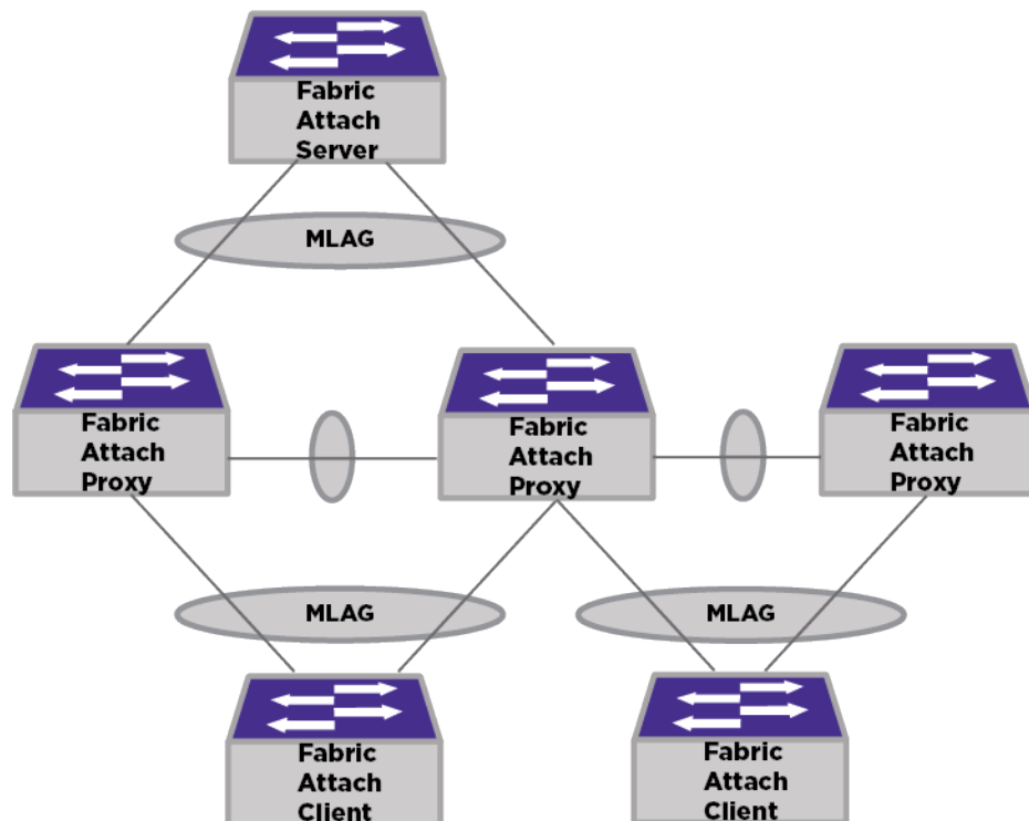
Figure 85: Fabric Attach with W-MLAG
