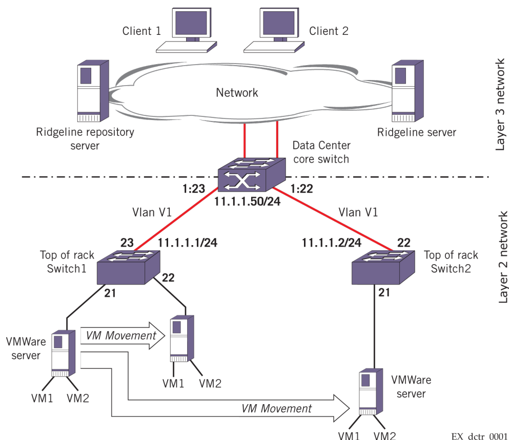
Figure 38: Sample XNV Topology
