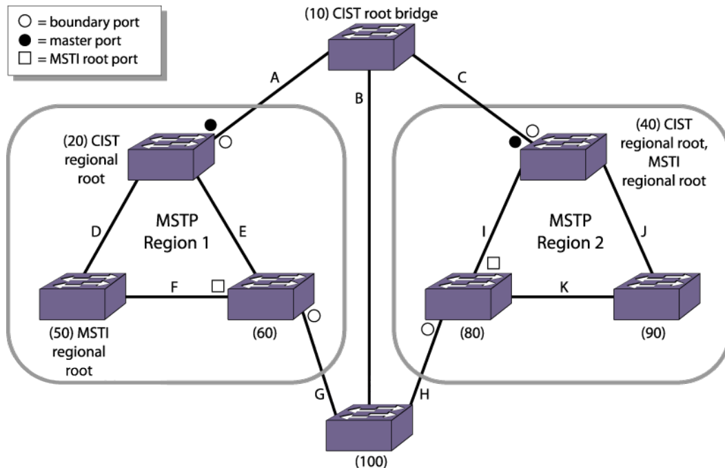
Figure 225: Sample MSTP Topology with Two MSTP Regions
