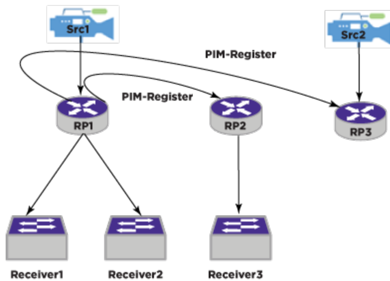
Figure 144: Anycast RP Operation
