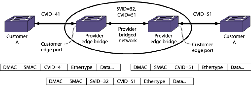
Figure 256: CVID Translation
