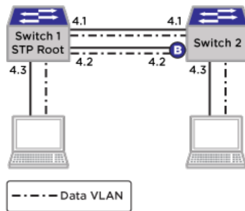
Figure 54: Sample STP Network for Migration to EAPS
