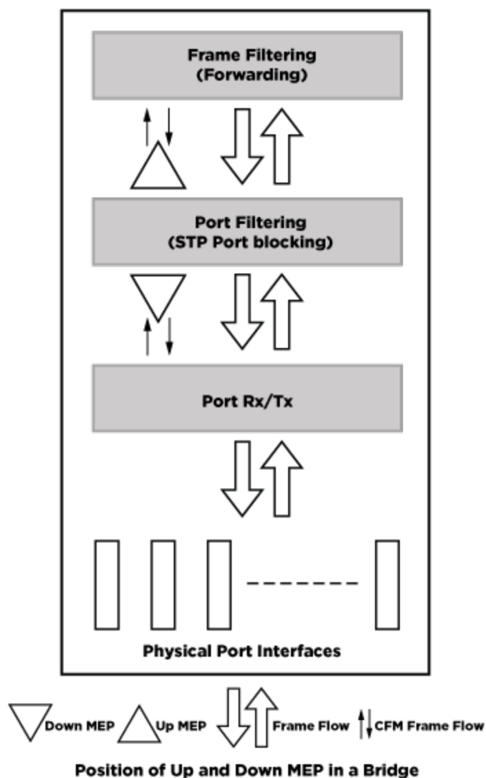
Figure 158: CFM UP and DOWN MEP at the Logical Level
