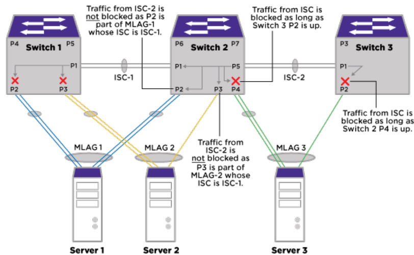
Figure 15: Traffic Flow (Unknown Traffic Switch-3 to Switch-2)
