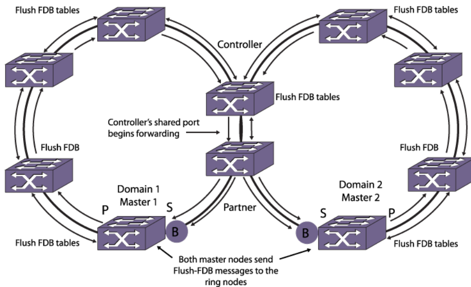
Figure 47: Common-Link Restored
