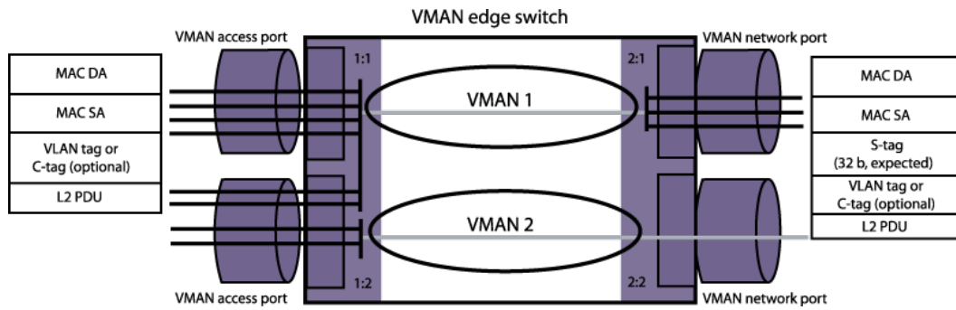
Figure 254: Tag Usage at the VMAN Access Switch
