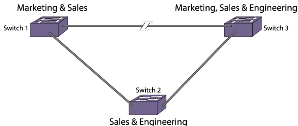
Figure 210: Incorrect Tag-Based STPD Configuration
