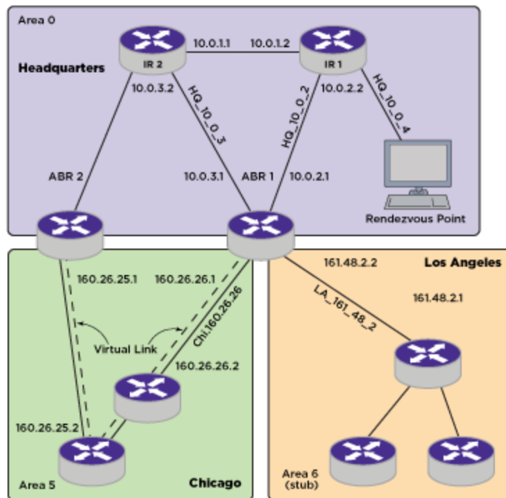
Figure 146: IP Multicast Routing Using PIM-SM Configuration Example
