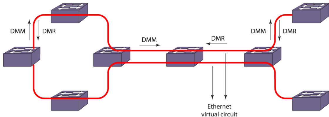
Figure 160: Two-Way Frame Delay and Frame Delay Variance Measurement
