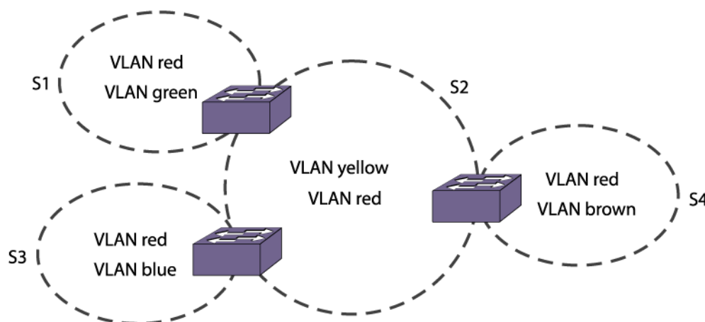
Figure 230: EMISTP Configuration Example
