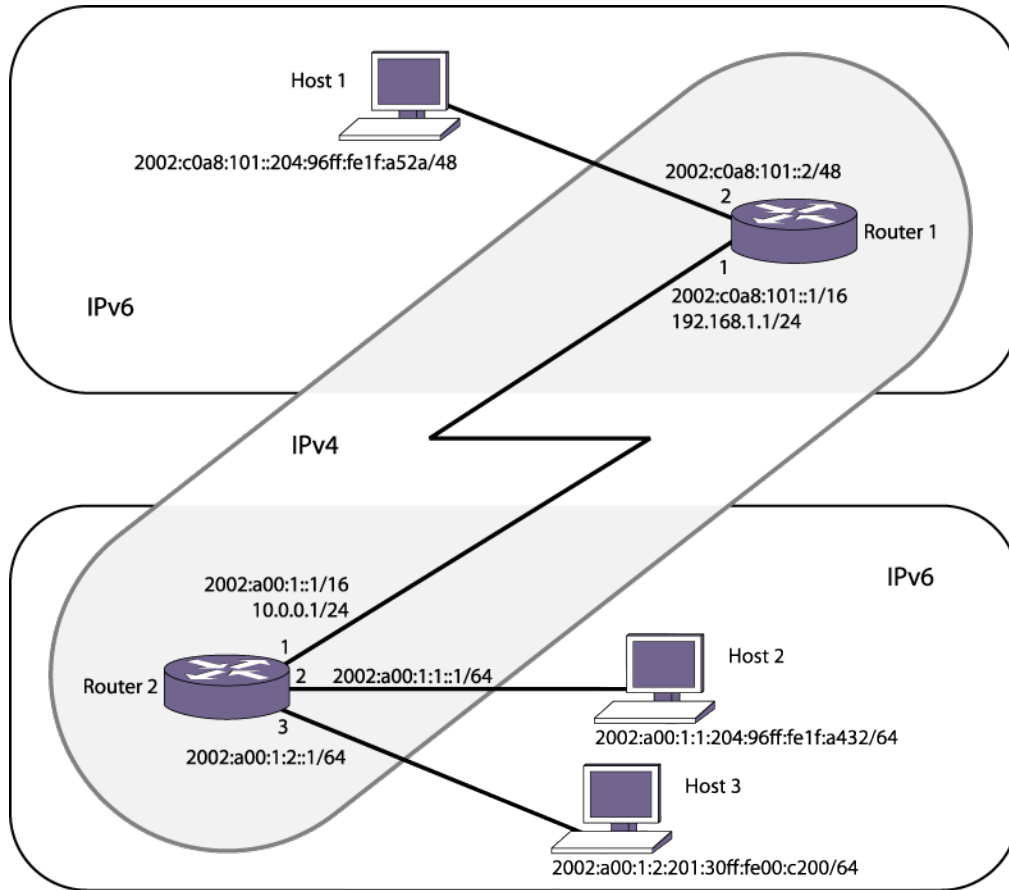
Figure 108: 6to4 Tunnel Configuration Example
