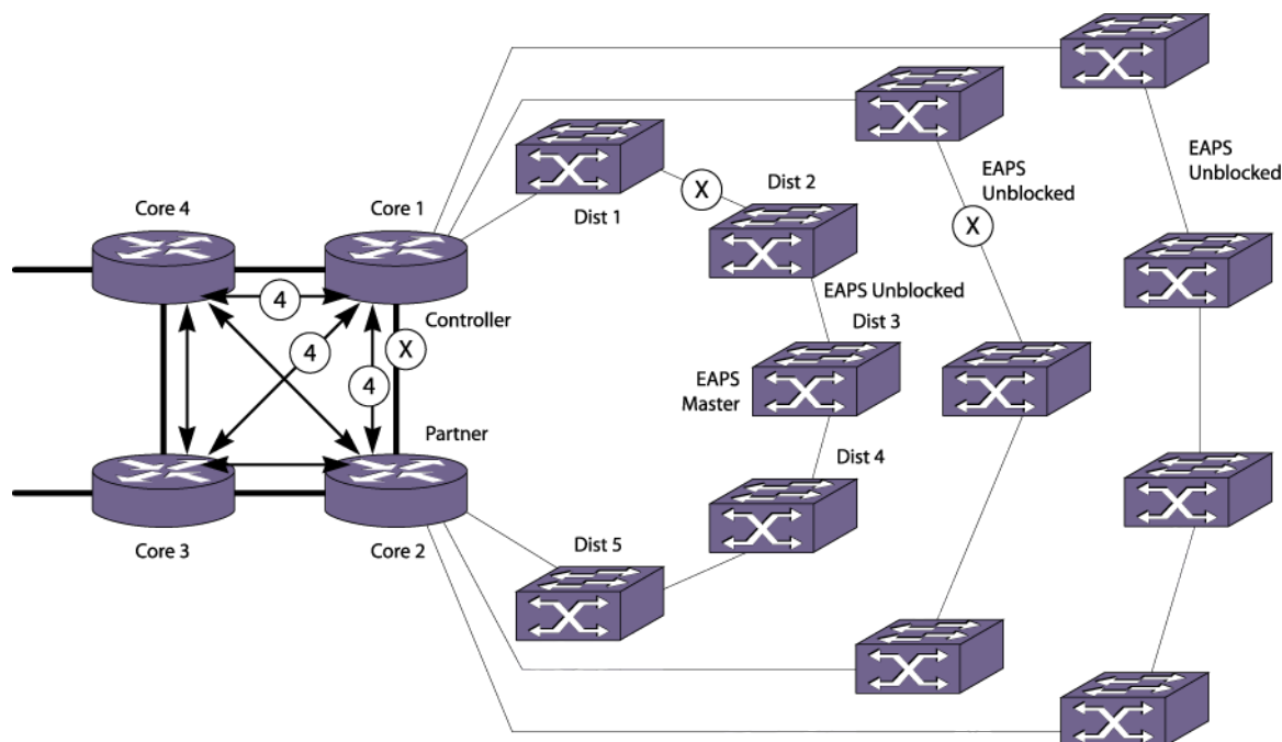
Figure 132: VPLS with Parallel Redundant EAPS Rings Configuration Example
