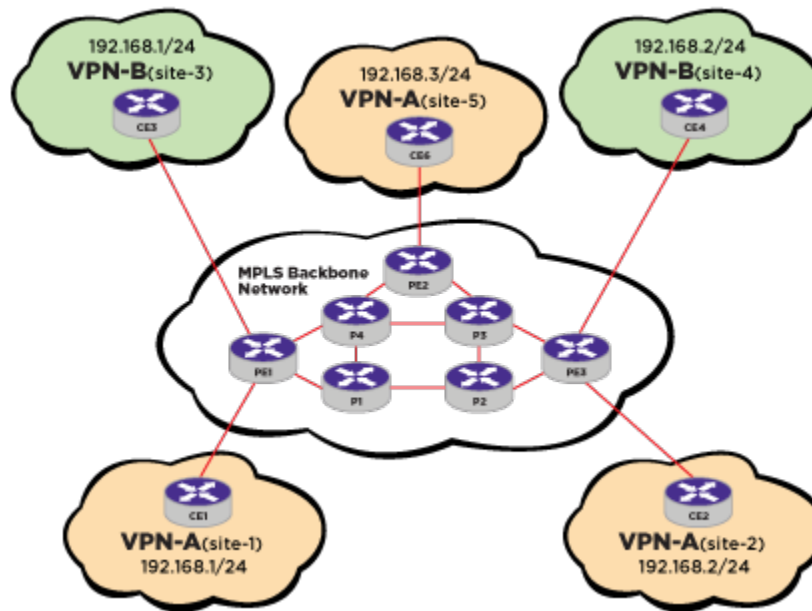
Figure 115: BGP/MPLS VPN Example
