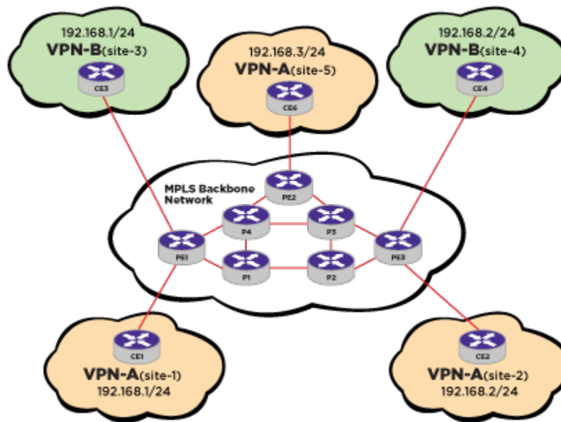
Figure 114: Different Router Roles in L3 VPN
