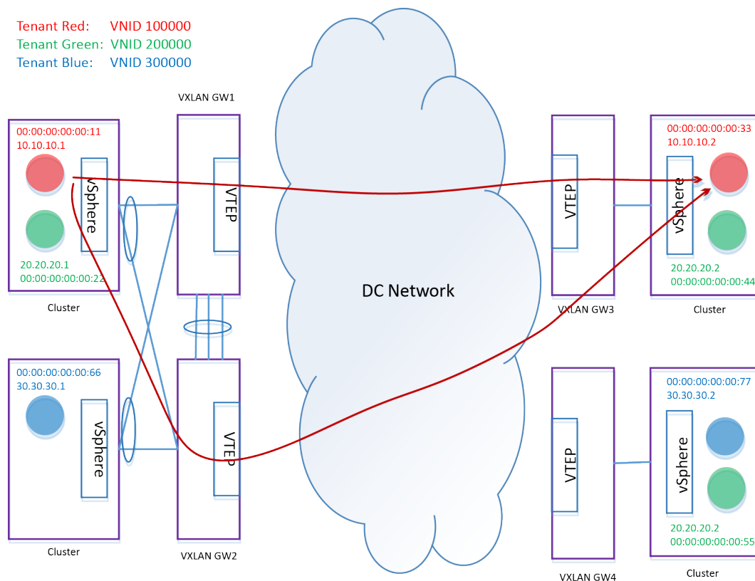
Figure 275: VXLAN Gateways with Three Tenants
