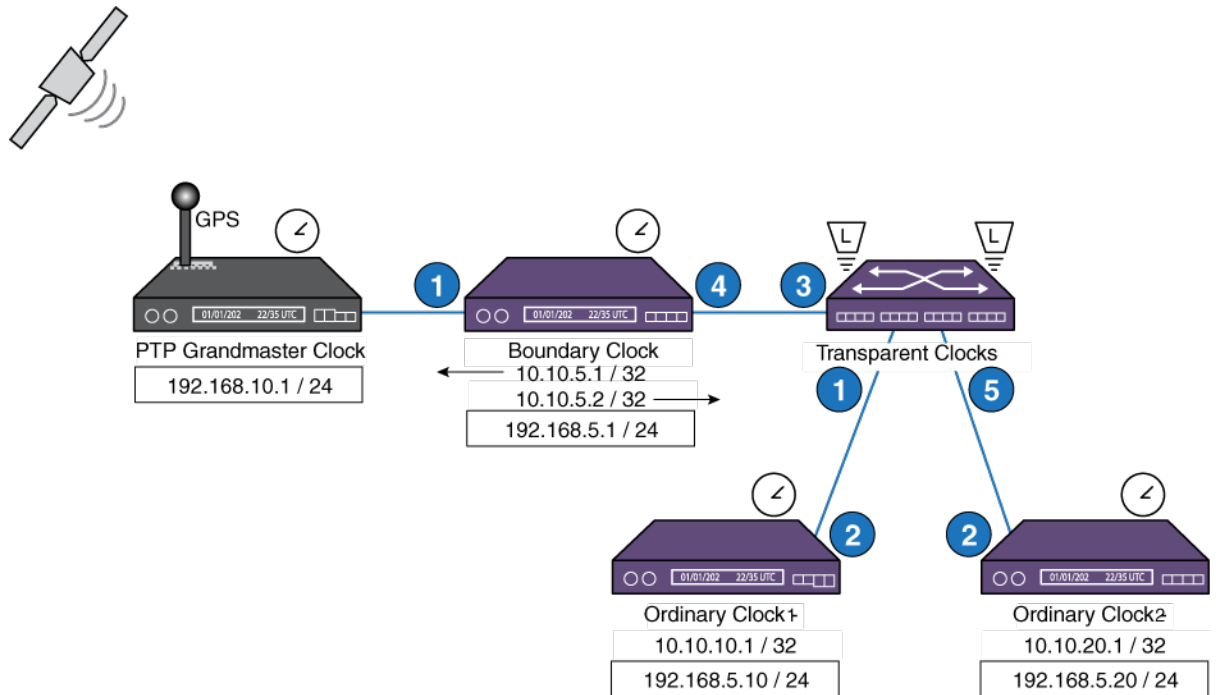
Figure 8: PTP 1588v2 Configuration Example
