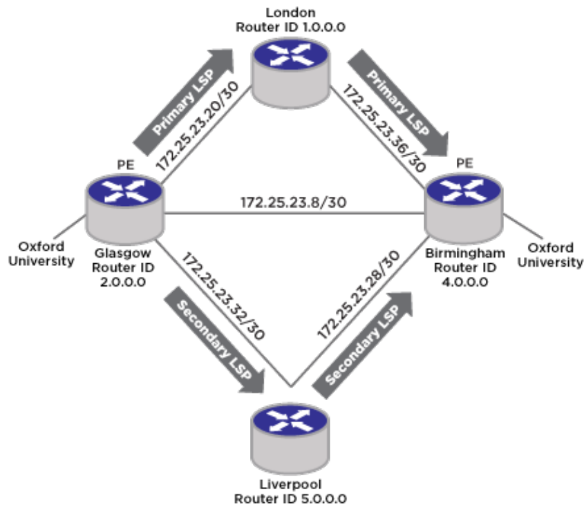
Figure 140: RSVP-TE Configuration Example
