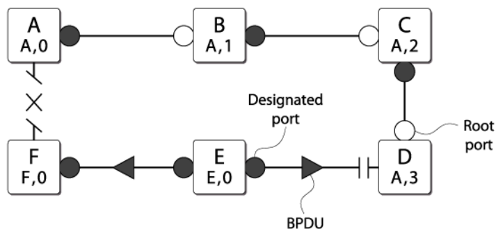
Figure 218: New Root Bridge Selected
