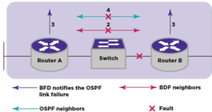
Figure 170: OSPF Neighbor Relationship Eliminated by BFD Fault Detection
