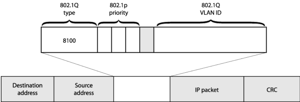
Figure 181: 802.1p Priority Bits
