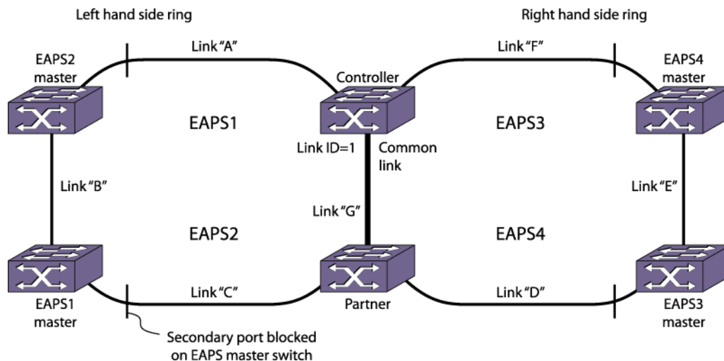
Figure 48: EAPS Common Link Topology with Spatial Reuse
