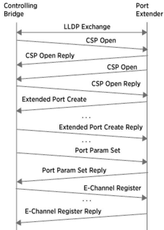
Figure 72: Example PE-CSP Protocol Exchange
