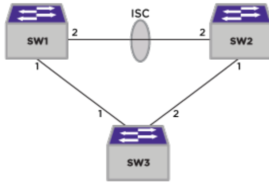
Figure 234: ELRP Egress Port Disable (2)
