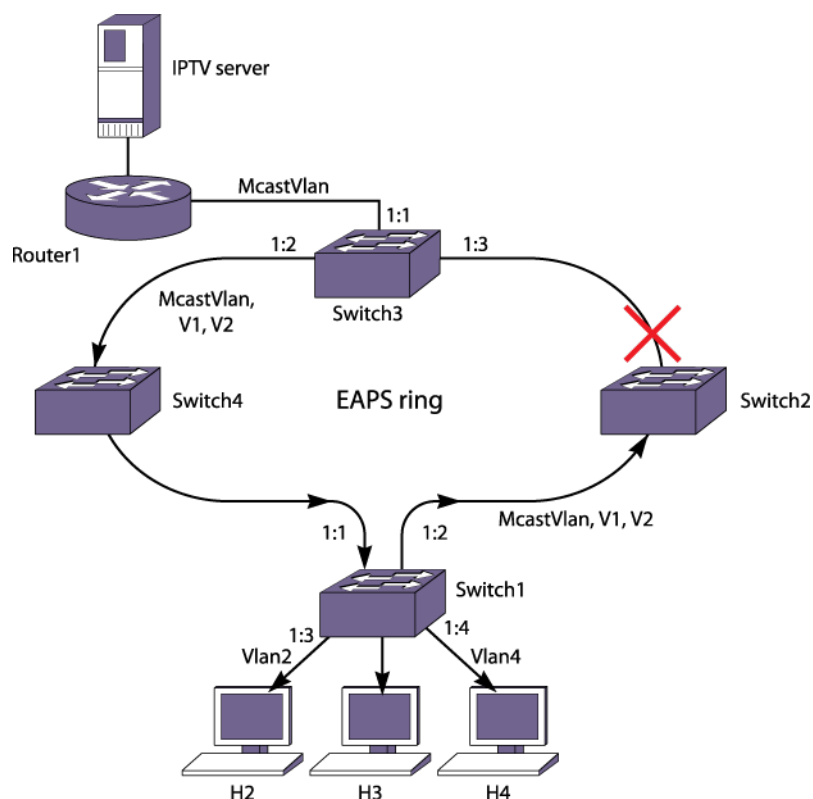
Figure 152: MVR on an EAPS Ring
