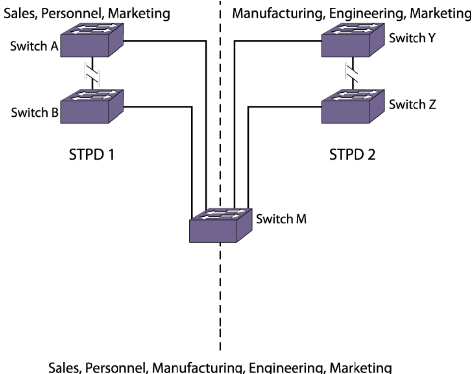
Figure 231: RSTP Example
