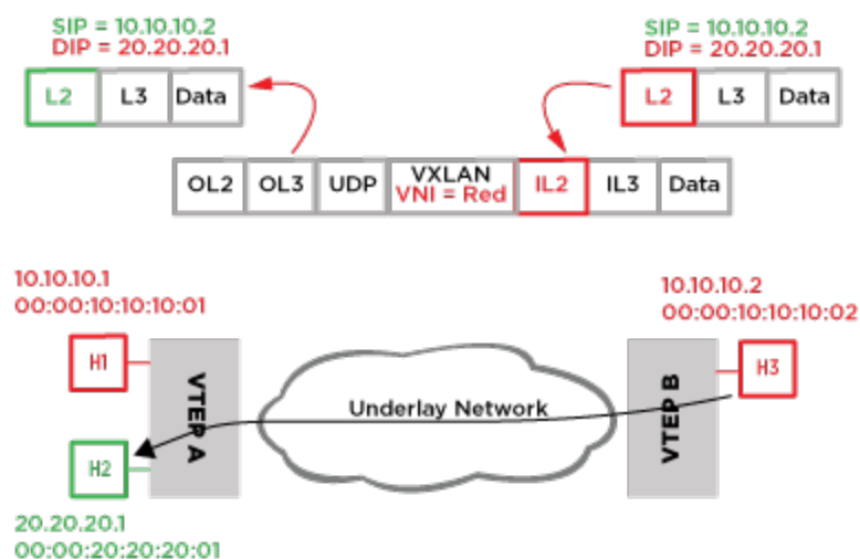
Figure 266: Routing from a Tunnel
