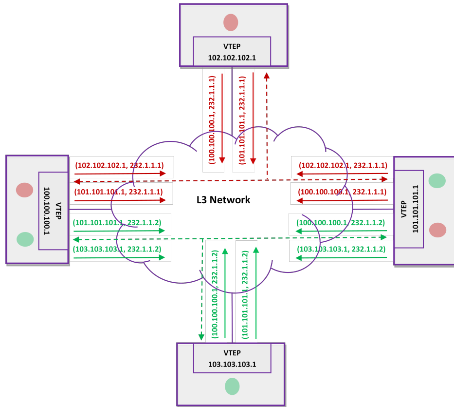
Figure 269: Underlay Multicast Distribution Tree
