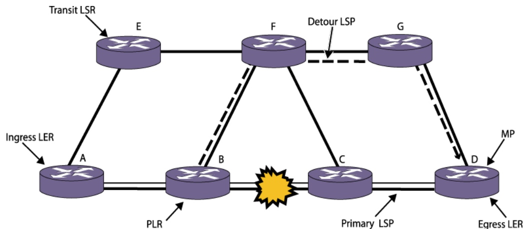
Figure 134: Fast-Reroute Terminology
