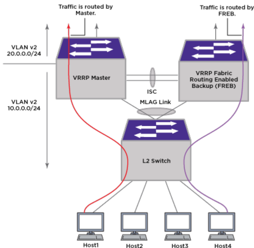
Figure 261: VRRP Fabric Routing
