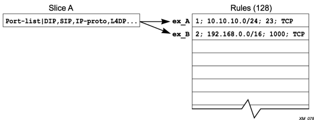
Figure 25: ACL Entry ex_A and ex_B
