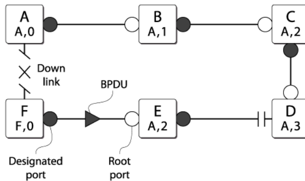
Figure 217: Down Link Detected
