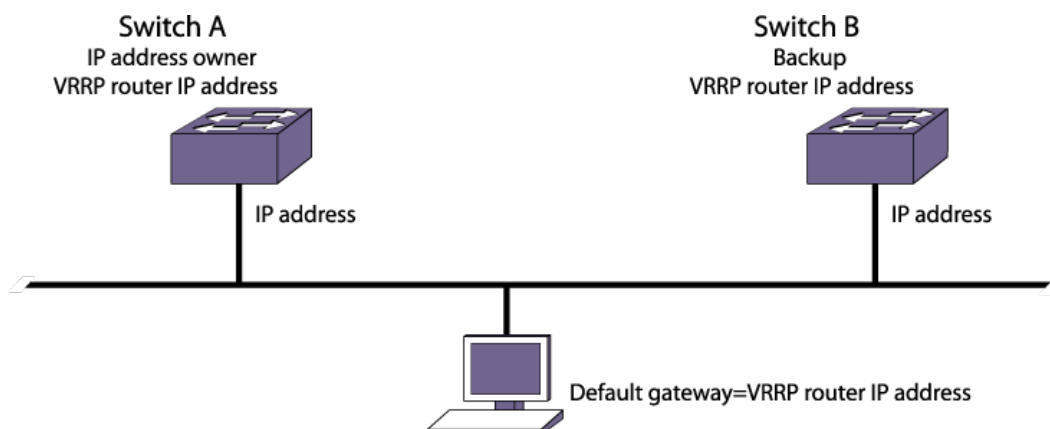
Figure 259: Simple VRRP Network
