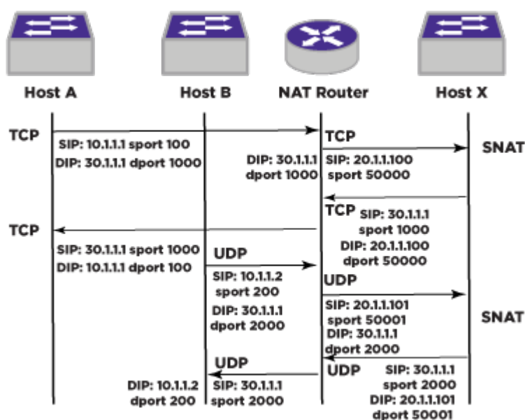
Figure 102: NAPT Example
