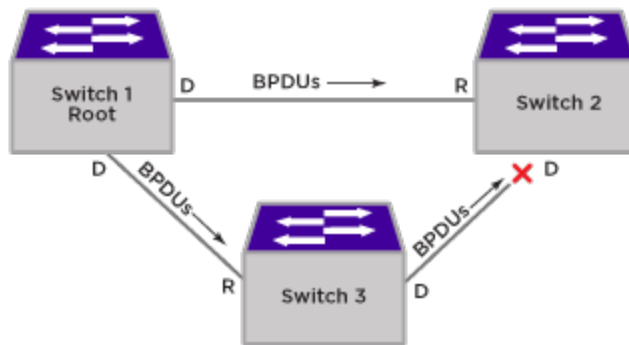
Figure 205: STP Disabled on Switch 2
