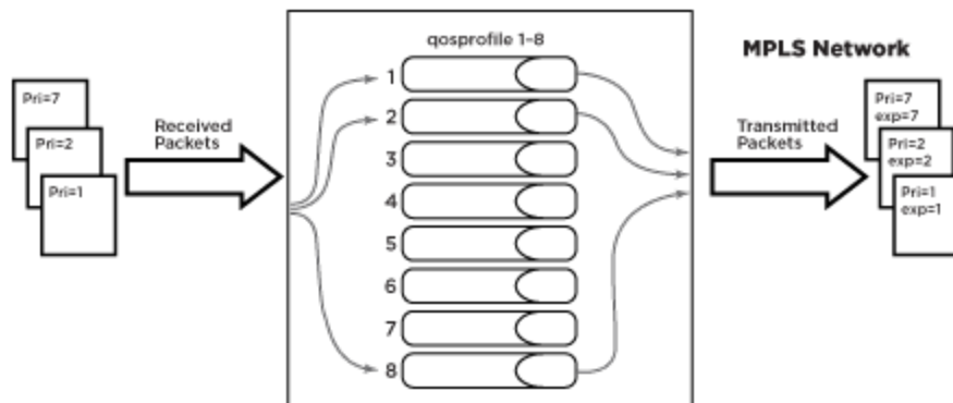
Figure 136: Mapping Dot1p to EXP Bits
