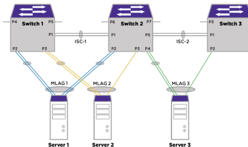
Figure 13: Two MLAG Peer Topology
