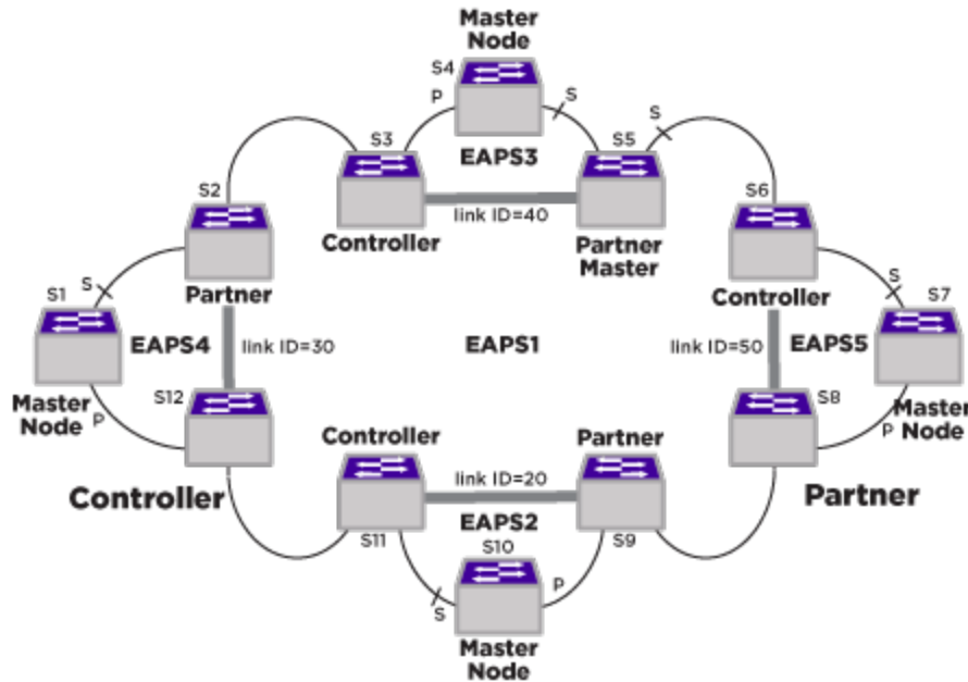
Figure 53: Large Core and Access Ring Topology
