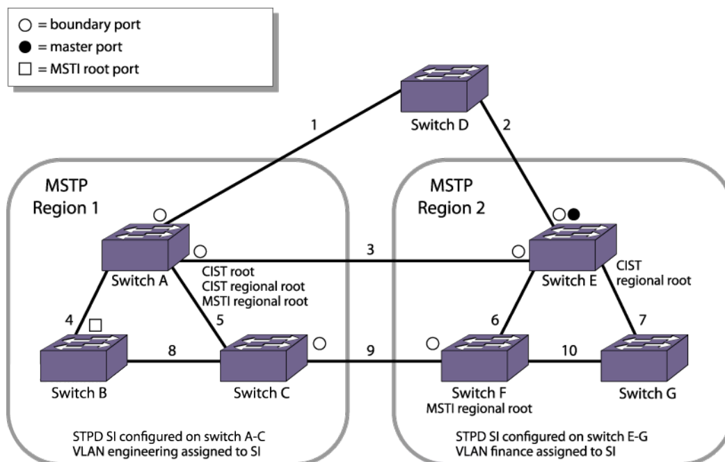
Figure 226: MSTP Topology with the CIST Root Bridge Contained within a Region
