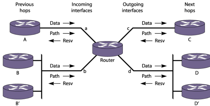
Figure 133: RSVP Messages
