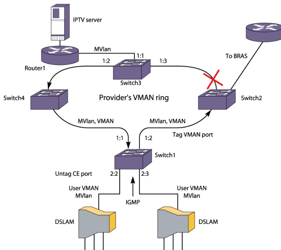
Figure 154: MVR in a VMAN Environment
