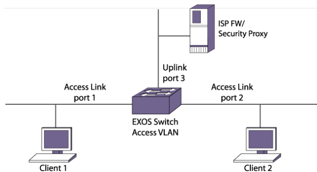
Figure 90: Upstream Forwarding or Disabling Egress Flooding Example
