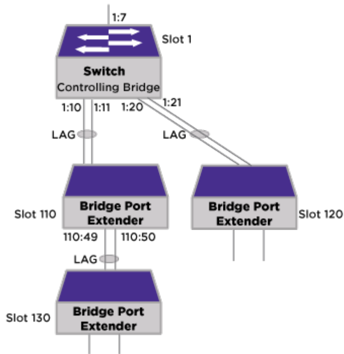
Figure 78: CB with Two-Tier BPEs Topology
