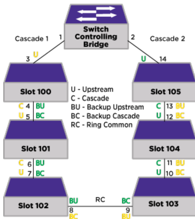
Figure 75: Counter-directional Cascades on Completed Ring
