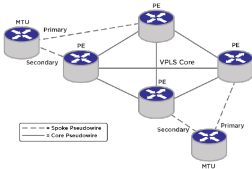
Figure 126: Example H-VPLS Network with Redundant Spokes
