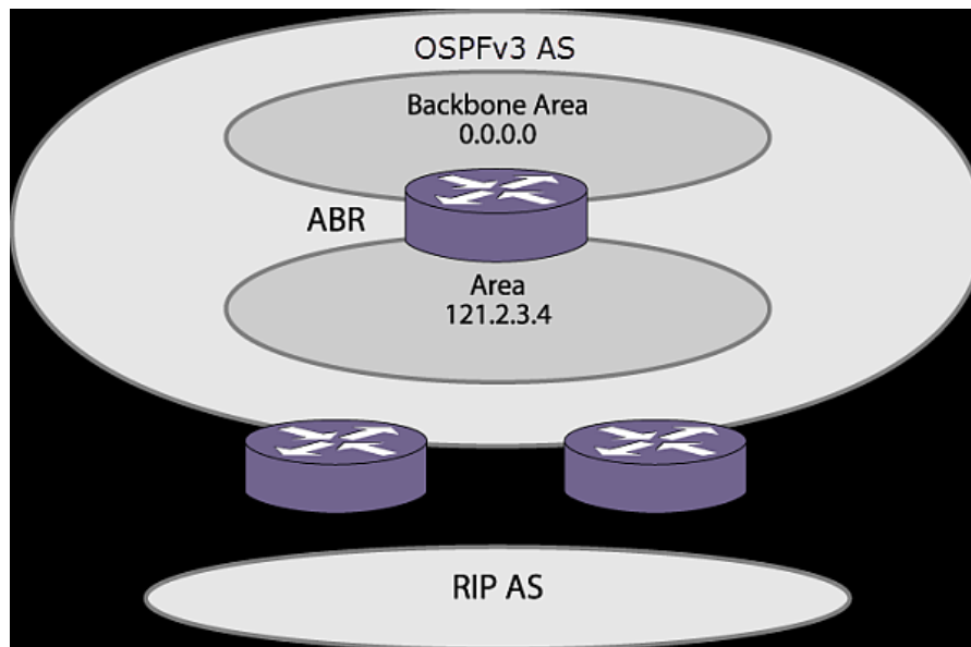
Figure 29: OSPF Route Redistribution
