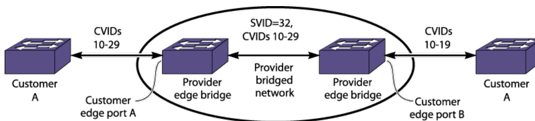
Figure 257: CVID Egress Filtering
