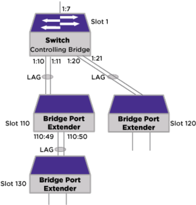
Figure 80: CB with Two-Tier BPEs Topology
