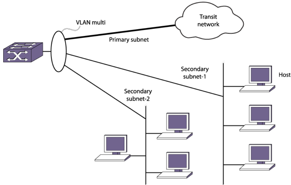
Figure 98: Multinetted Network Topology
