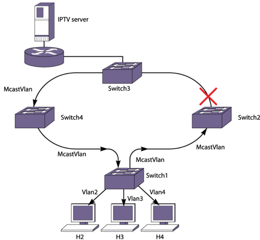
Figure 149: Basic MVR Deployment
