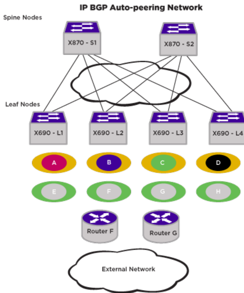
Figure 37: EVPN and Asymmetric VRF Routing in BGP Auto-peering with Routers
