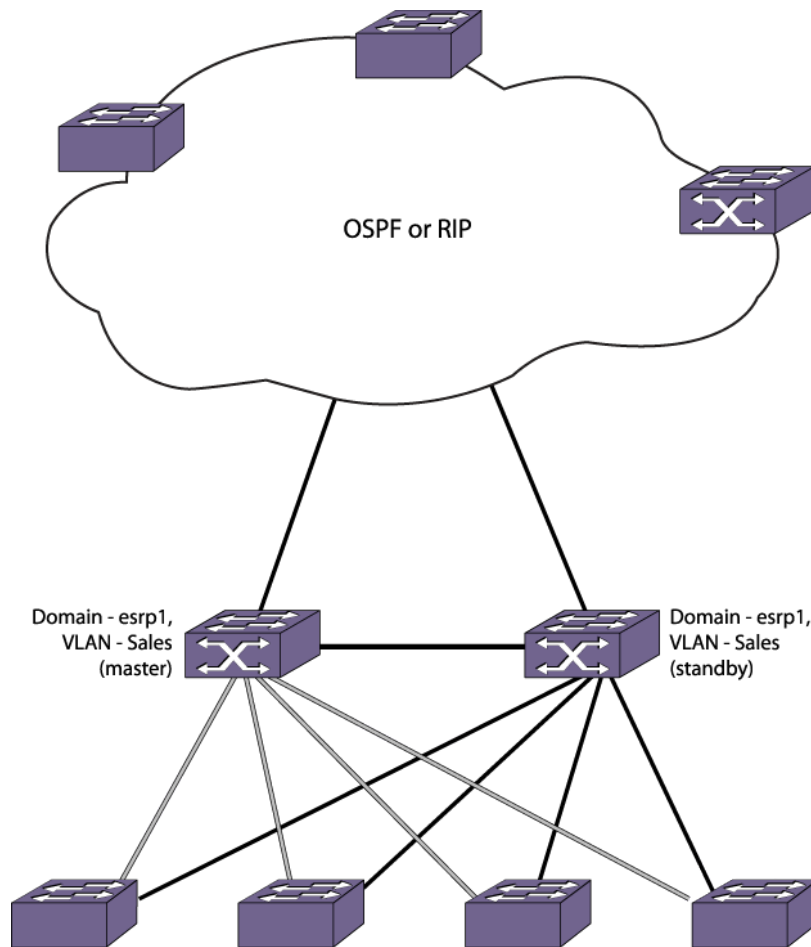
Figure 67: Single ESRP Domain Using Layer 2 and Layer 3 Redundancy
