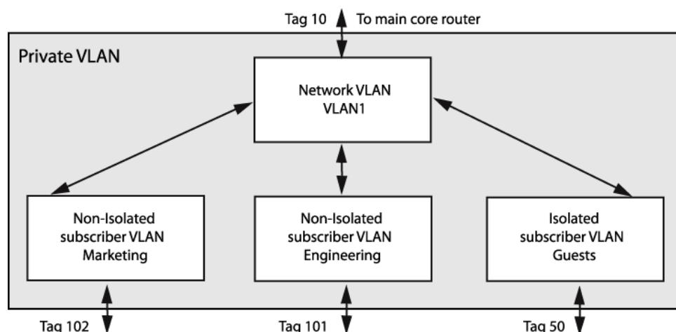
Figure 244: Private VLAN Switch Components
