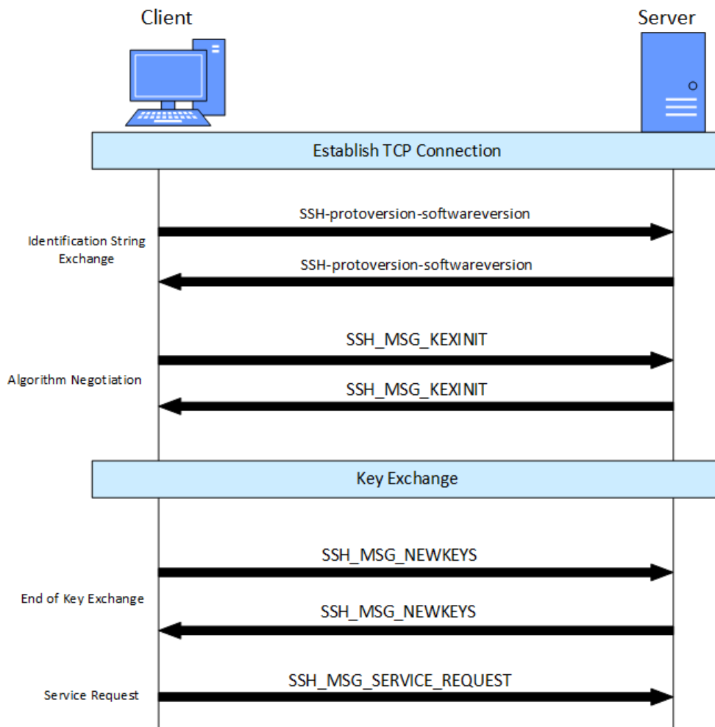
Figure 198: SSH Client /Server Connection Steps
