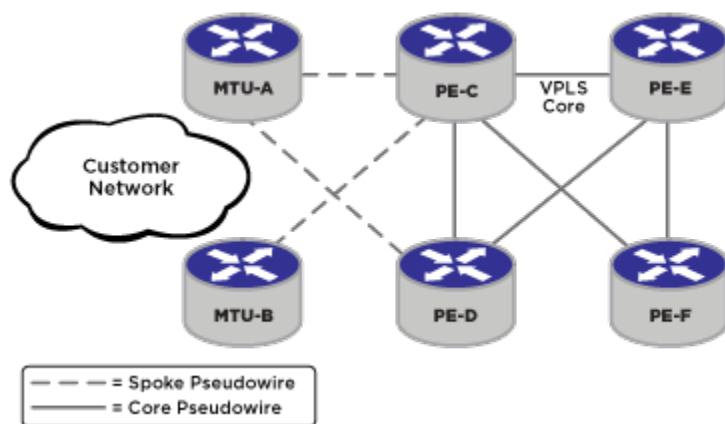
Figure 129: Example Redundant Edge H-VPLS Network
