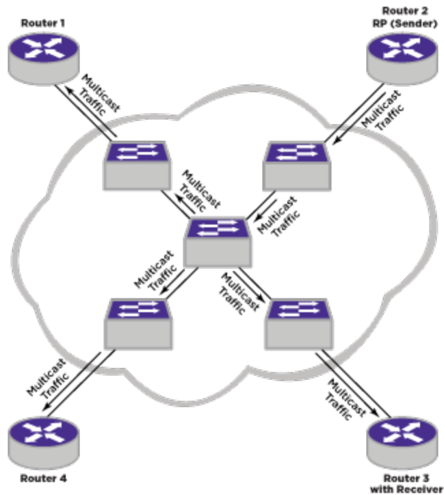
Figure 142: Multicast Without PIM Snooping
