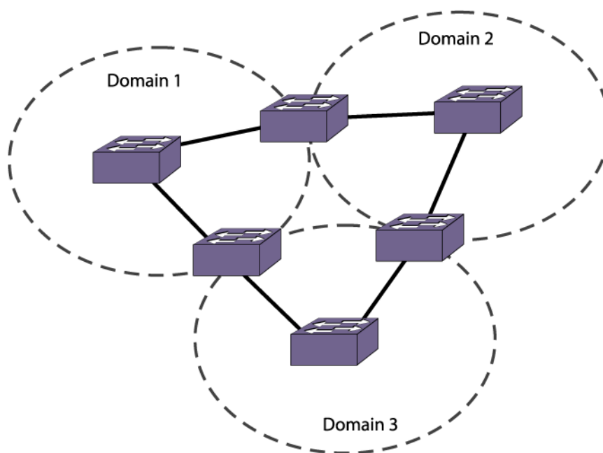
Figure 214: Looped VLAN Topology
