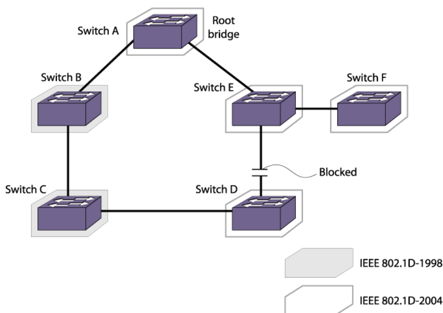
Figure 202: 802.1D-1998 and 802.1D-2004 Mixed Bridge Topology
