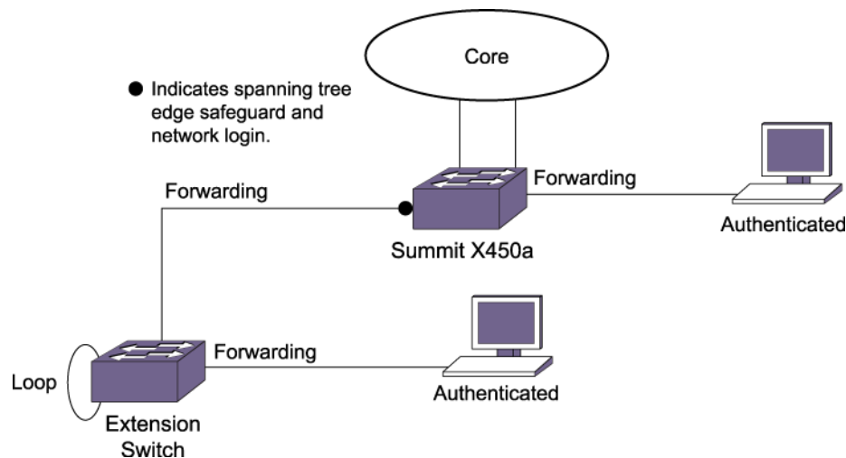
Figure 228: Traffic Monitoring on the Edge Side
