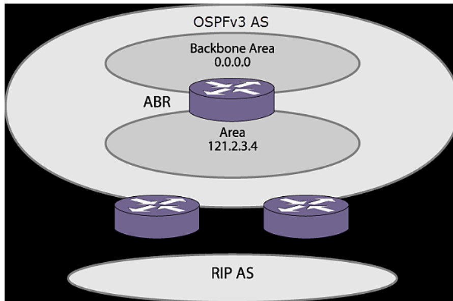
Figure 179: OSPF Route Redistribution
