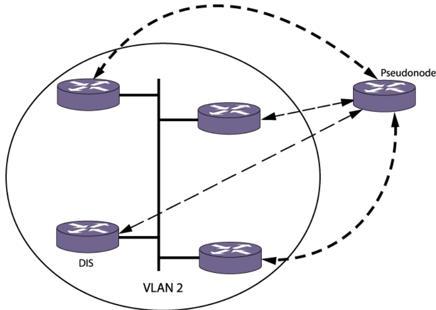
Figure 111: Broadcast Adjacencies in a Four-Router Network
