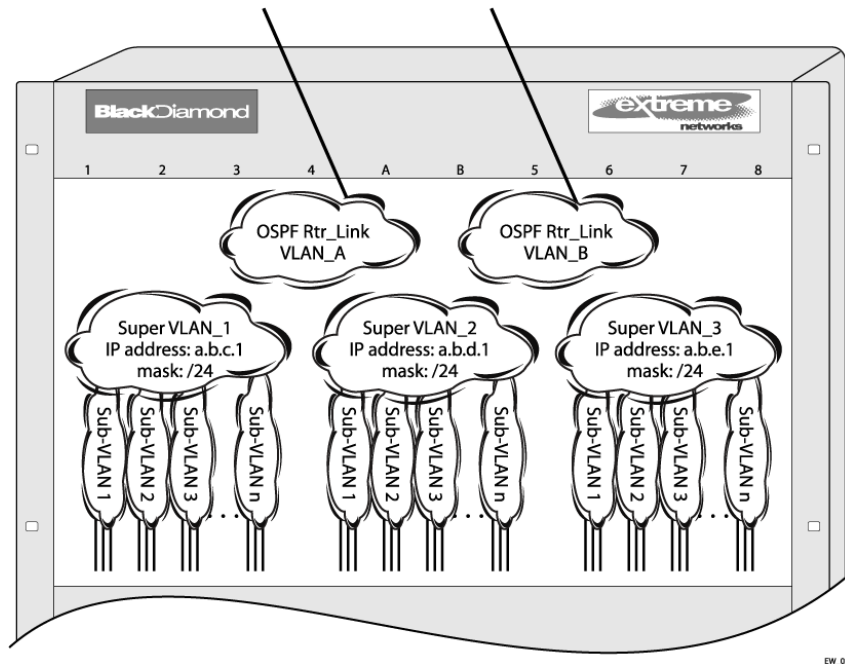
Figure 99: VLAN Aggregation
