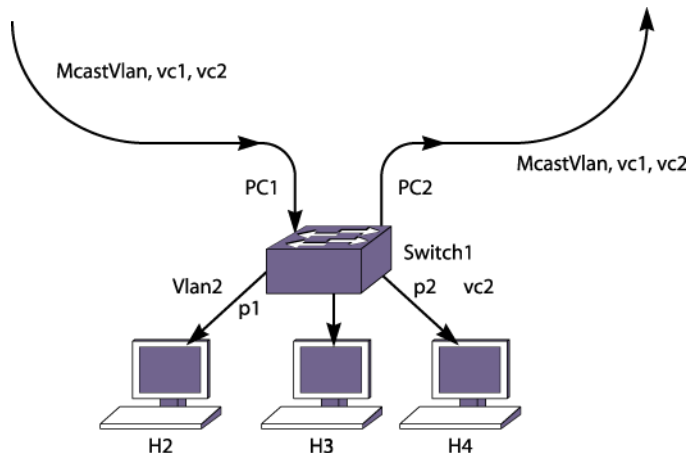
Figure 150: Multiple VLANs in the Core Network
