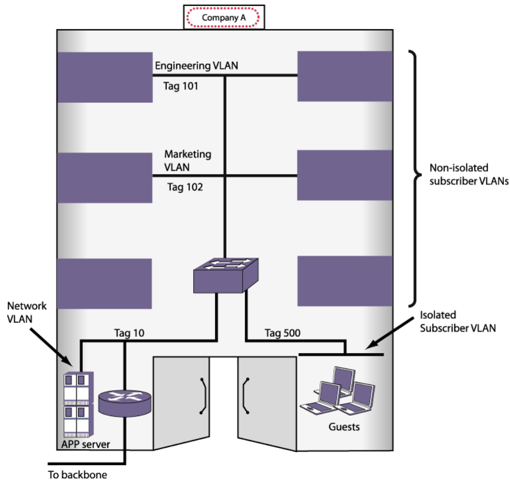
Figure 243: VLAN Isolation Application
