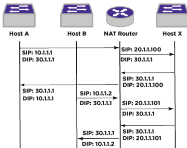
Figure 101: Address Translations During Basic NAT
