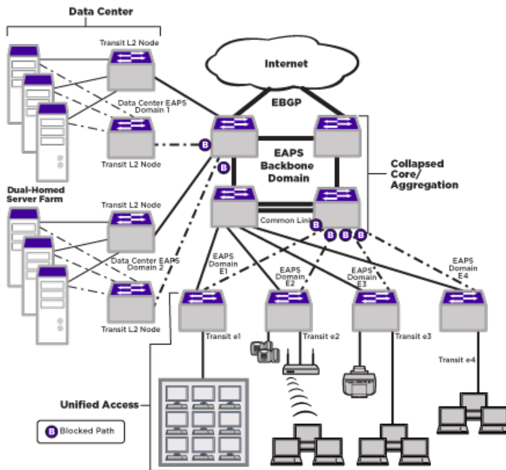
Figure 55: Extreme Networks EAPS Everywhere
