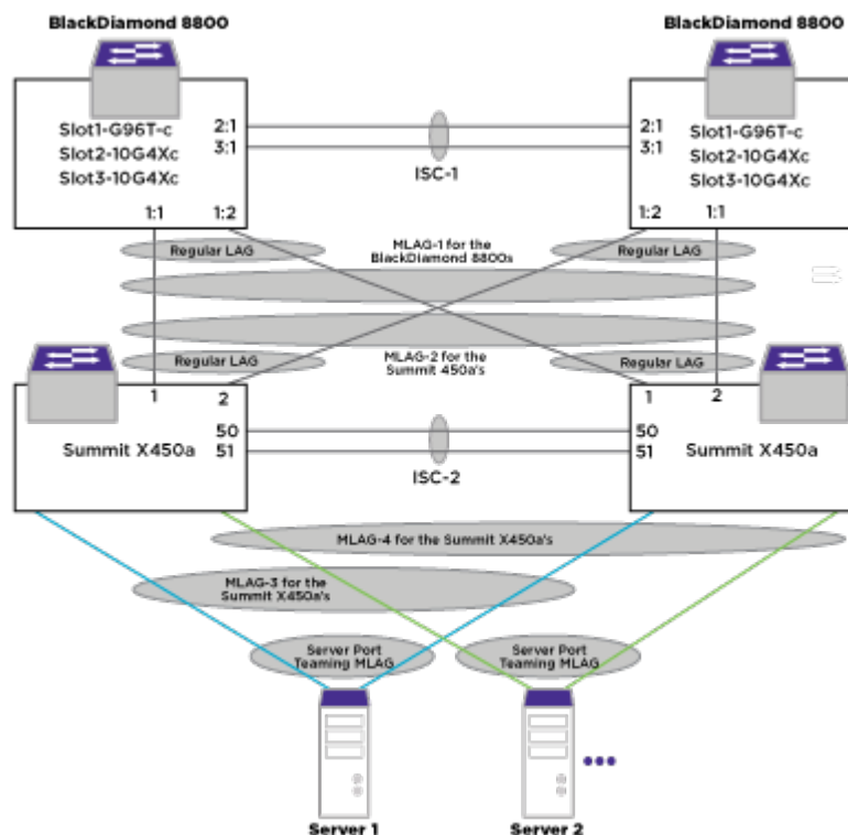
Figure 19: Two-tier MLAG Network
