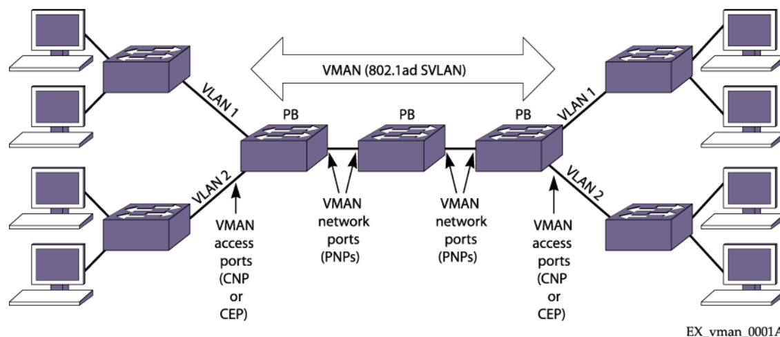
Figure 253: VMAN in PBN
