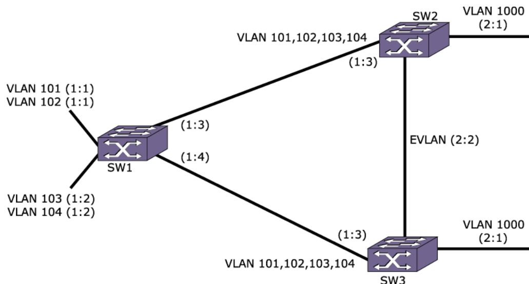
Figure 251: ESRP Redundancy Configuration Example
