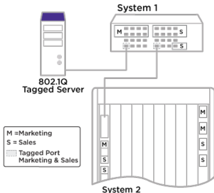
Figure 239: Physical Diagram of Tagged and Untagged Traffic
