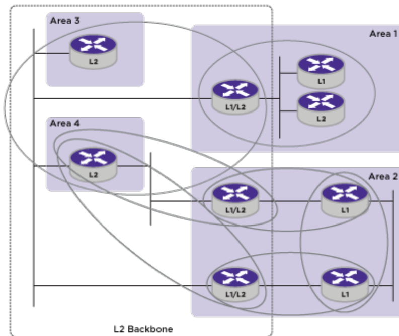
Figure 112: Basic Autonomous System
