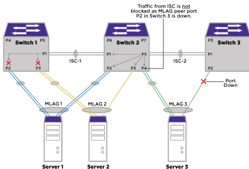
Figure 17: Peer Port Failure (cont.)
