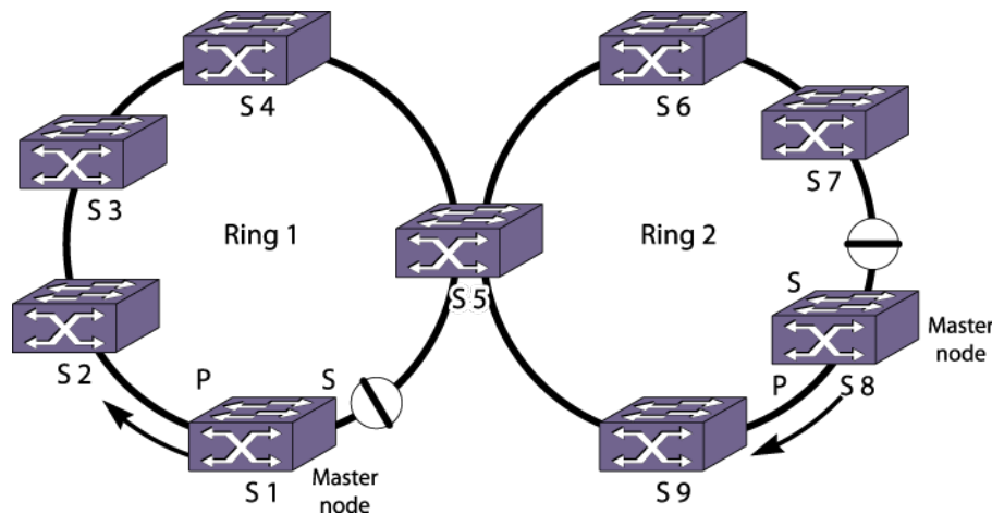
Figure 41: Two Rings Interconnected by One Switch
