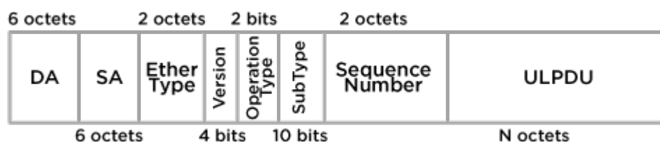
Figure 71: ECPDU Structure
