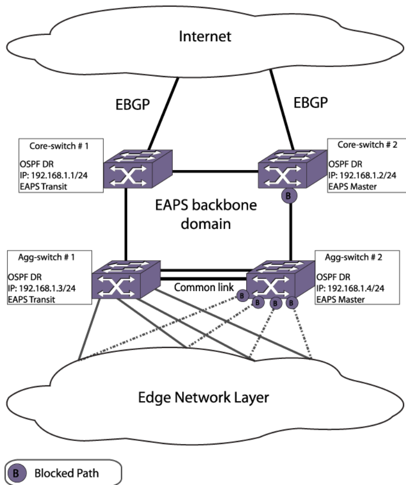
Figure 59: Core EAPS and OSPF Network Layer
