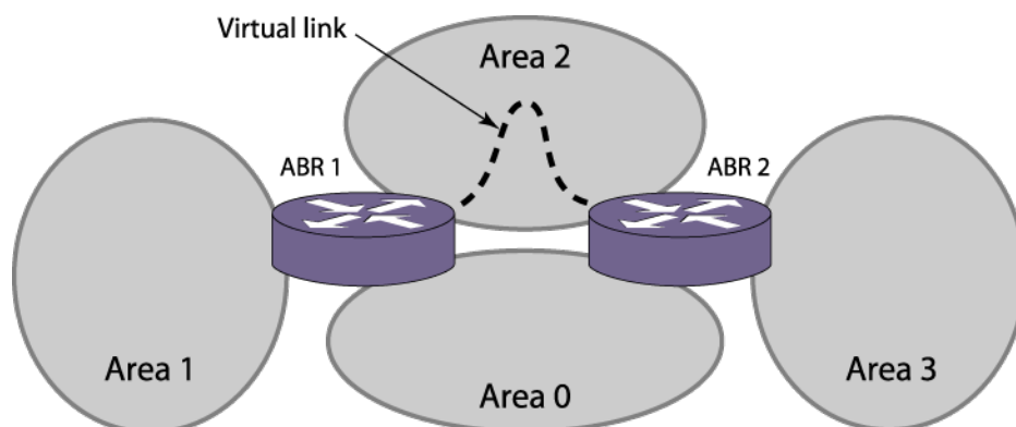
Figure 172: Virtual Link Providing Redundancy
