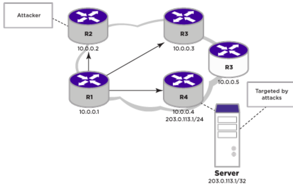
Figure 32: Black Hole Routing Using BGP
