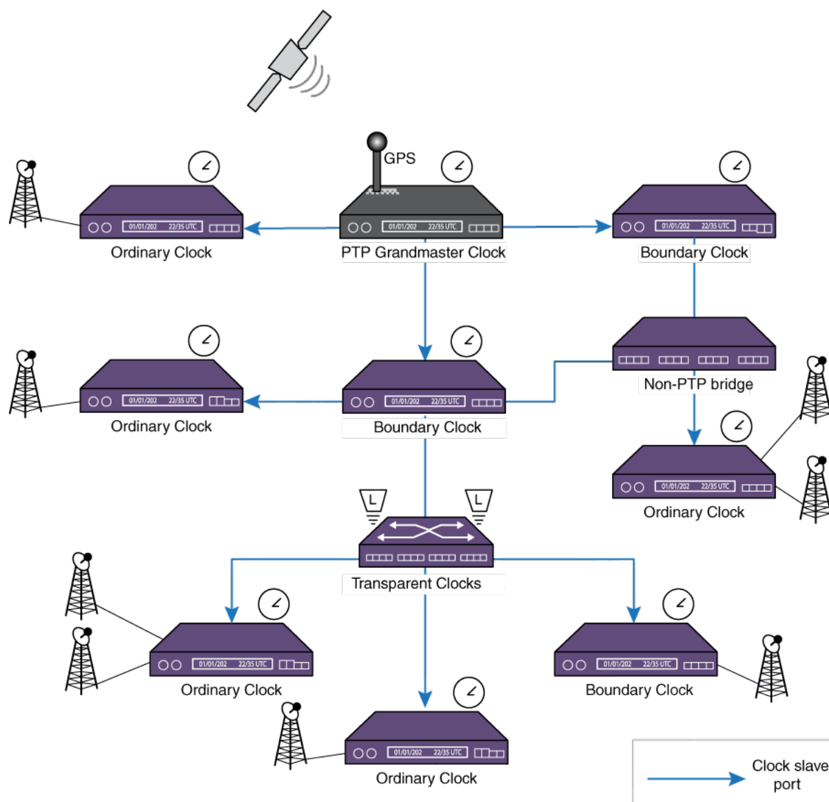
Figure 7: PTP Network Hierarchy
