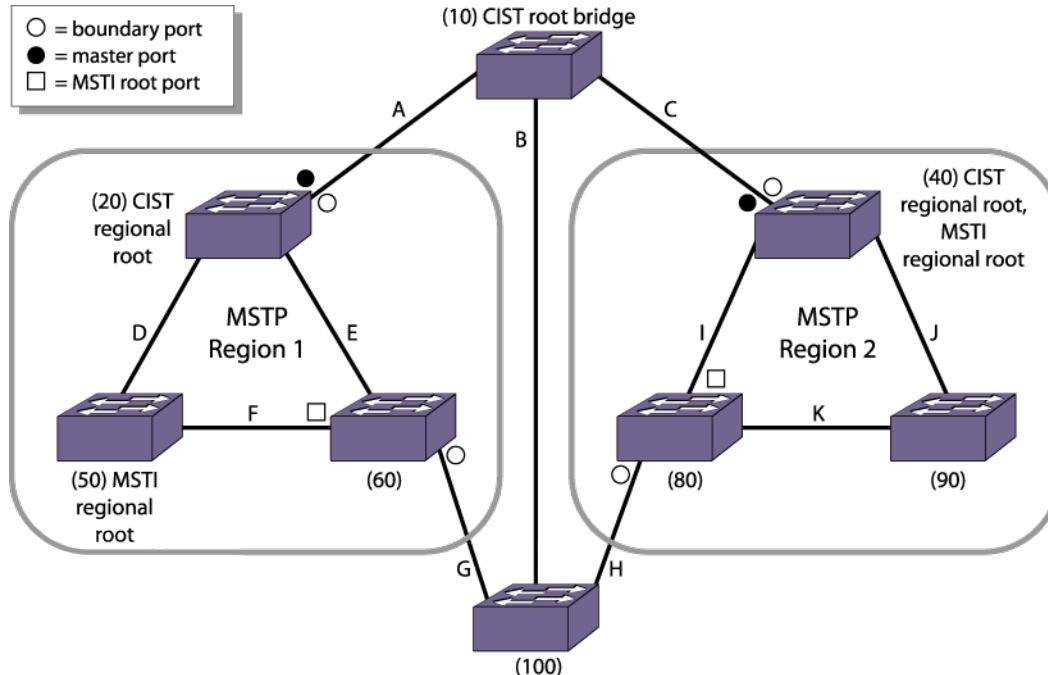
Figure 224: Sample MSTP Topology with Two MSTP Regions
