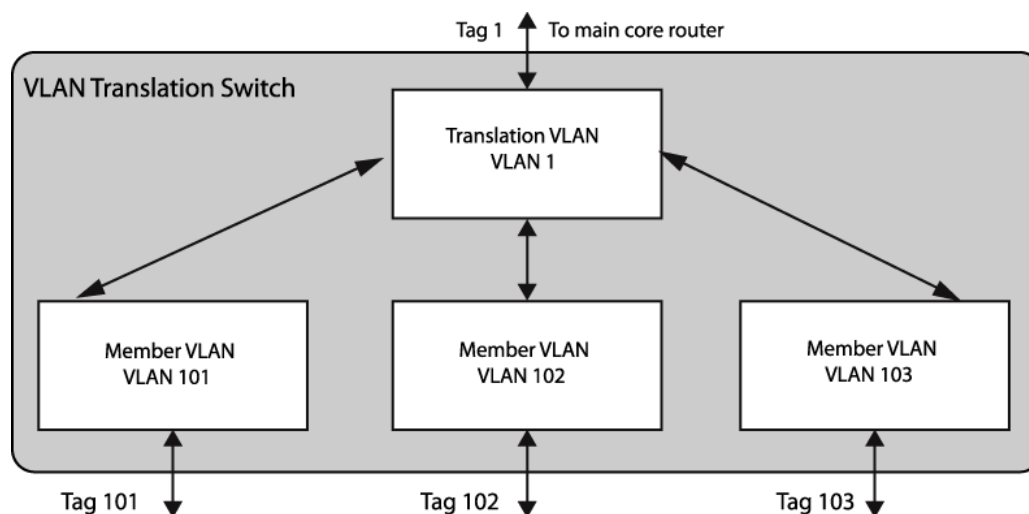
Figure 249: VLAN Translation Switch Configuration
