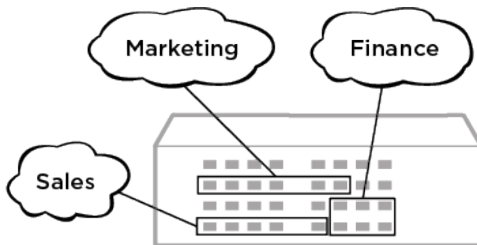
Figure 236: Example of a Port-Based VLAN on an Extreme Networks Switch
