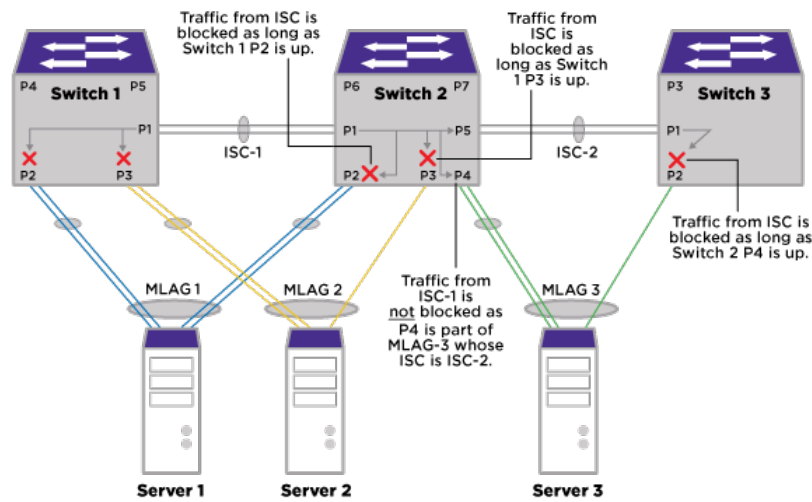
Figure 14: Traffic Flow
