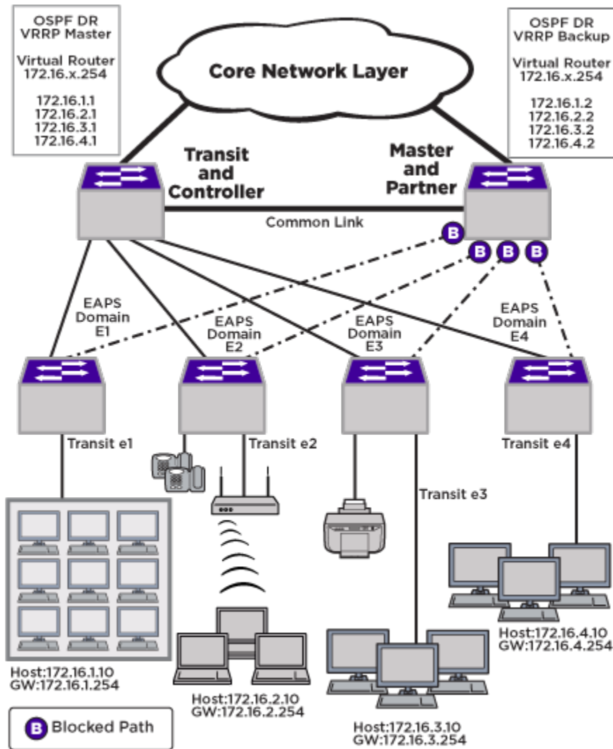
Figure 58: L2 and L3 Aggregation Network Layer
