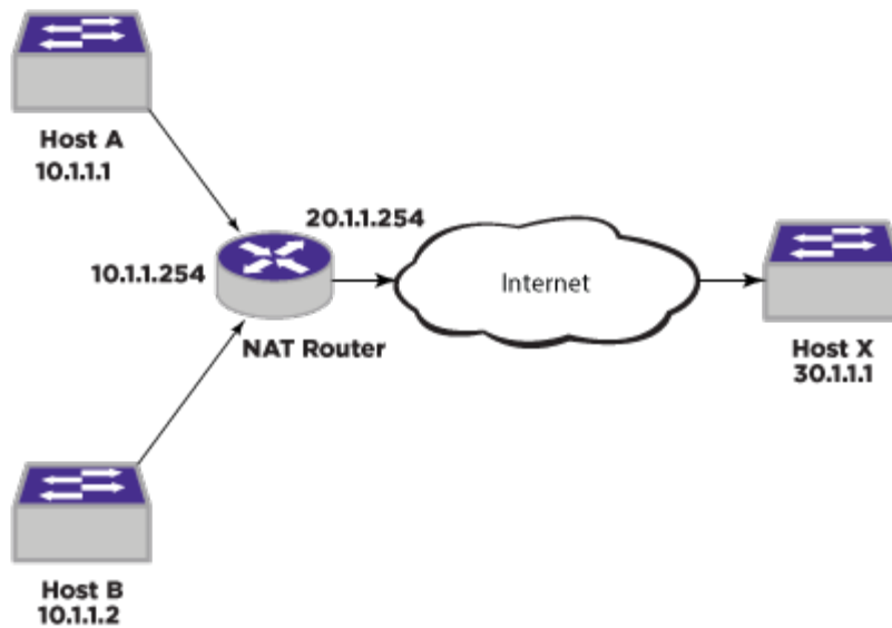
Figure 100: Example Network for NAT and NAT
