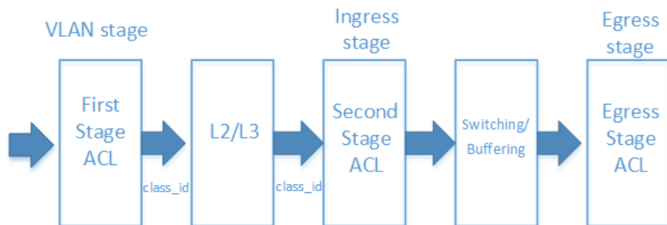
Figure 24: ACL Stages
