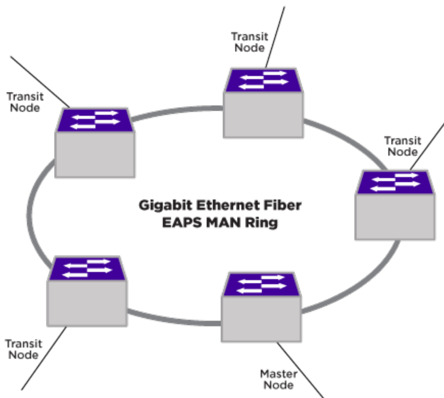
Figure 39: Gigabit Ethernet Fiber EAPS MAN Ring
