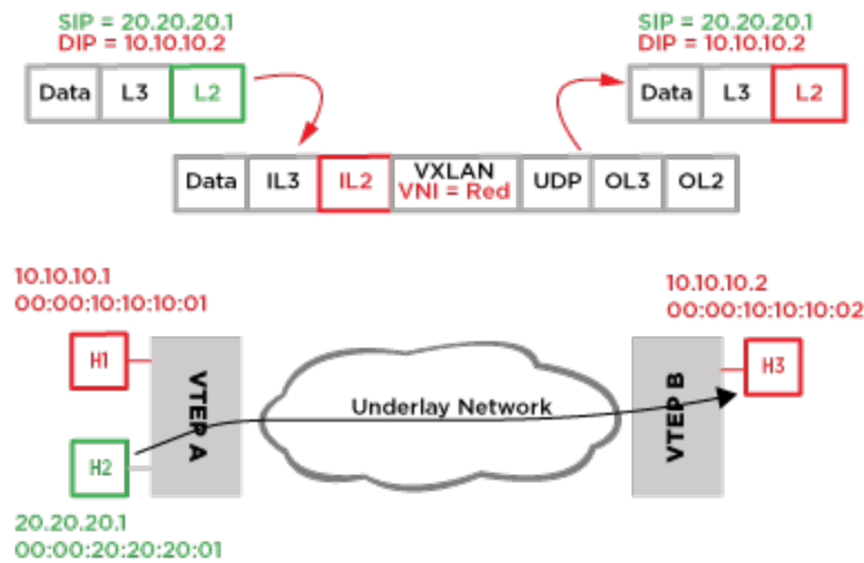
Figure 265: Routing into a Tunnel
