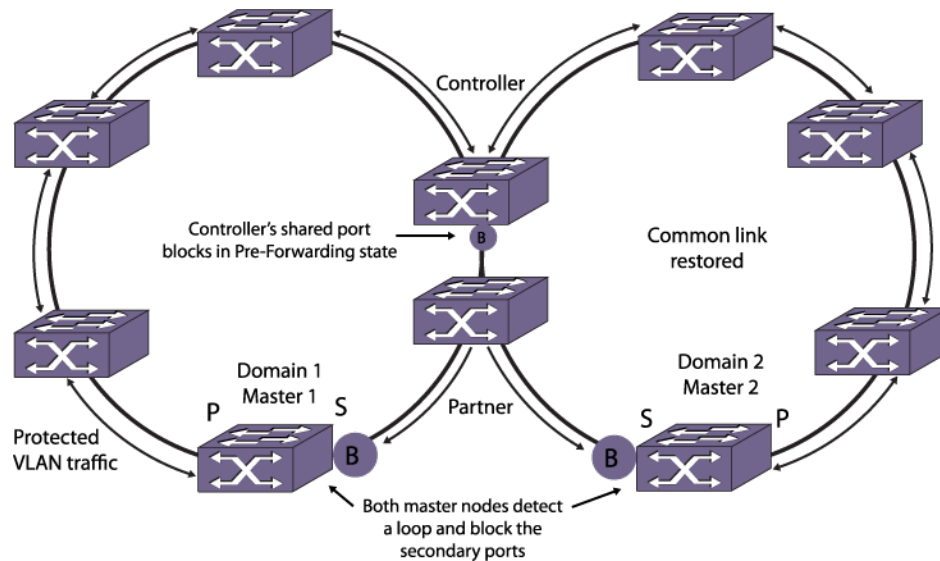
Figure 46: Common Link in Pre-Forwarding State
