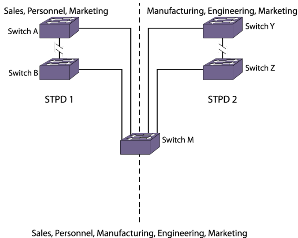
Figure 209: Multiple STPDs
