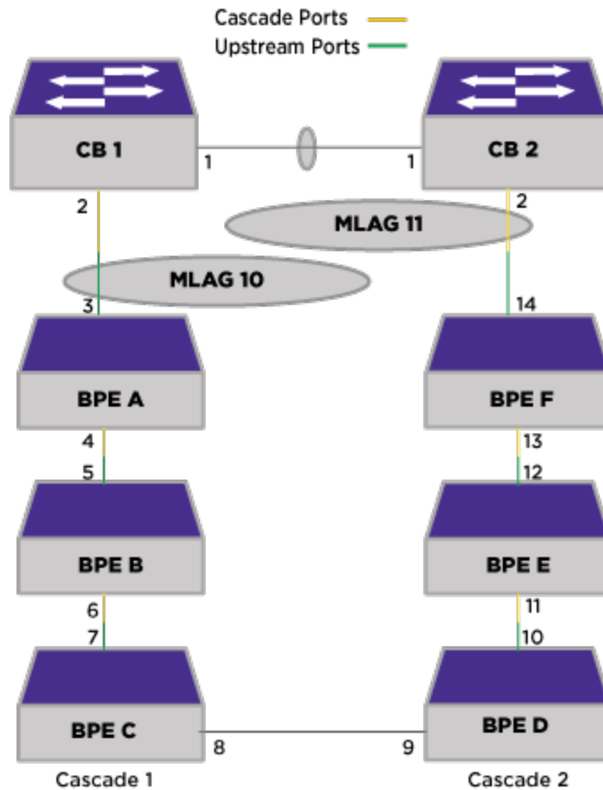
Figure 77: One-Arm MLAG
