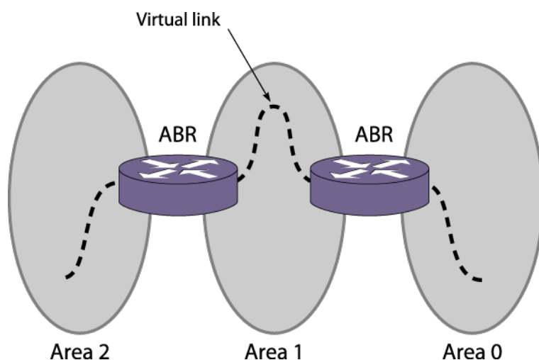
Figure 171: Virtual Link Using Area 1 as a Transit Area
