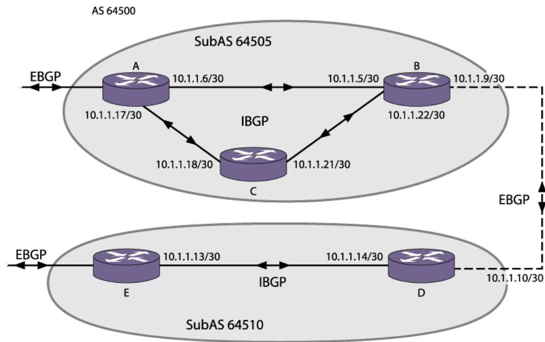
Figure 28: Routing Confederation
