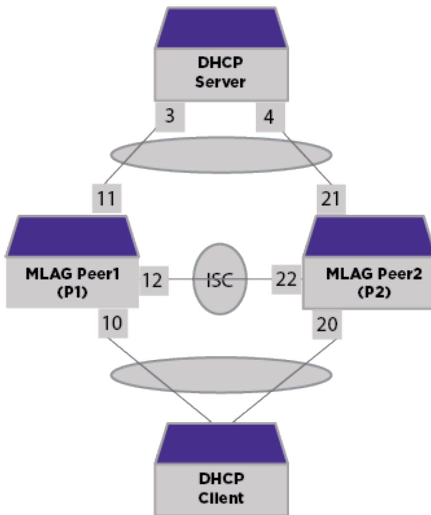
Figure 194: MLAG Topology
