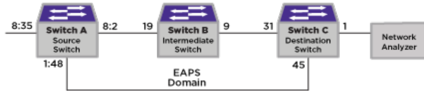
Figure 22: Remote Mirroring with EAPS
