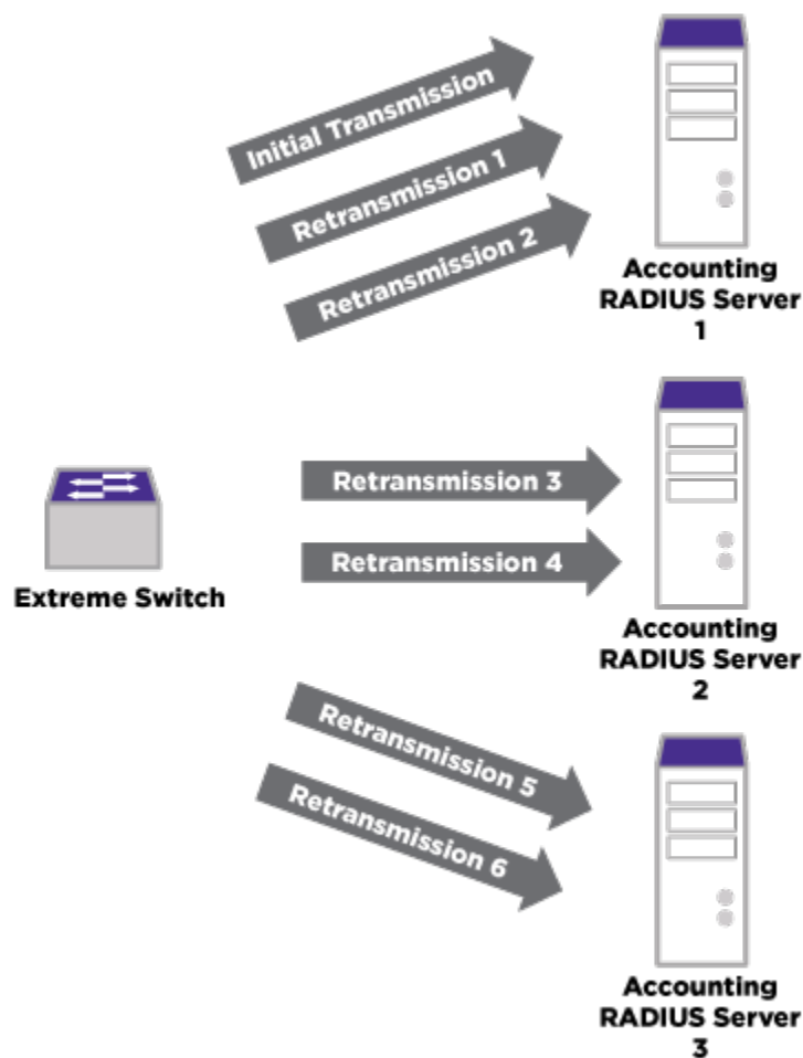
Figure 197: Accounting Retransmission Algorithm (No Servers Responding)
