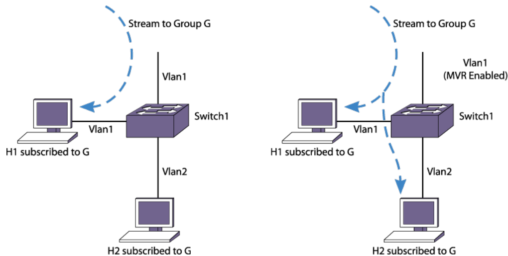
Figure 148: Standard VLAN Compared to an MVR VLAN
