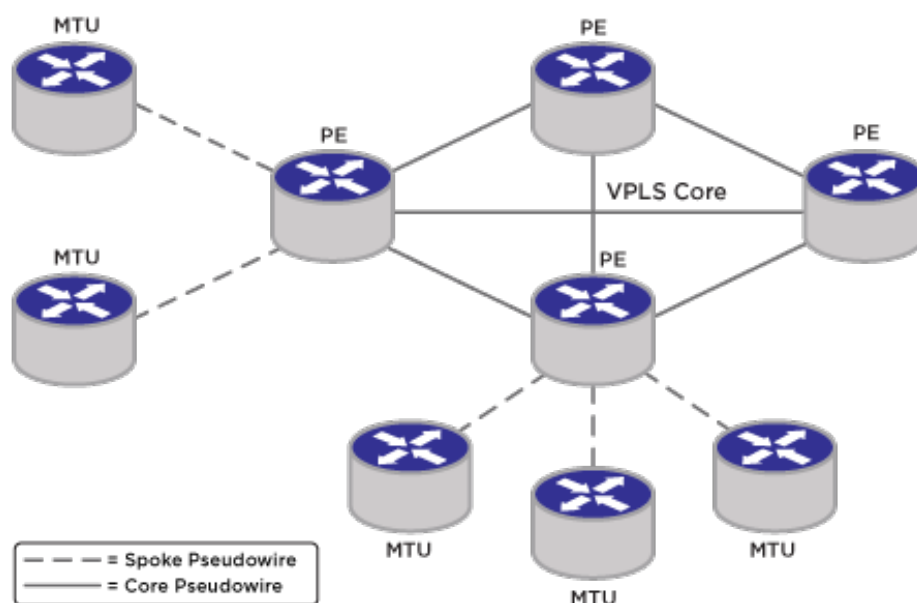
Figure 125: Example H-VPLS Network
