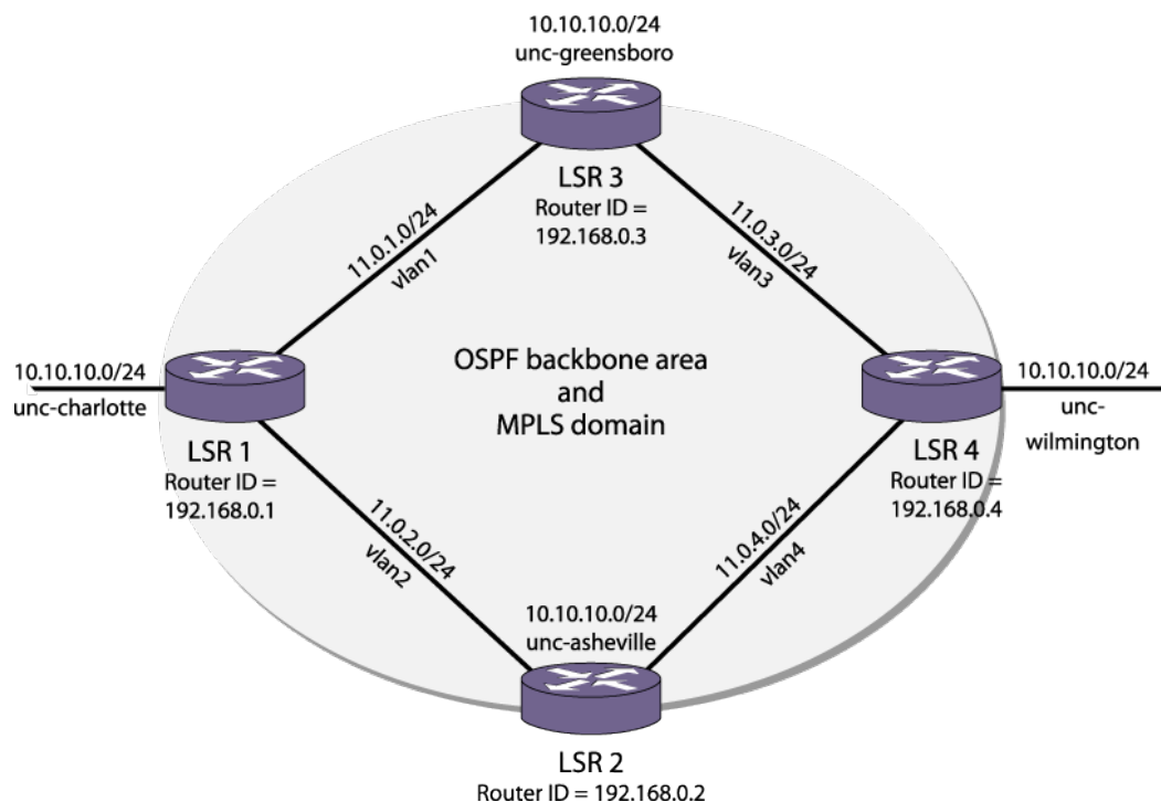
Figure 139: Full Mesh Configuration Example
