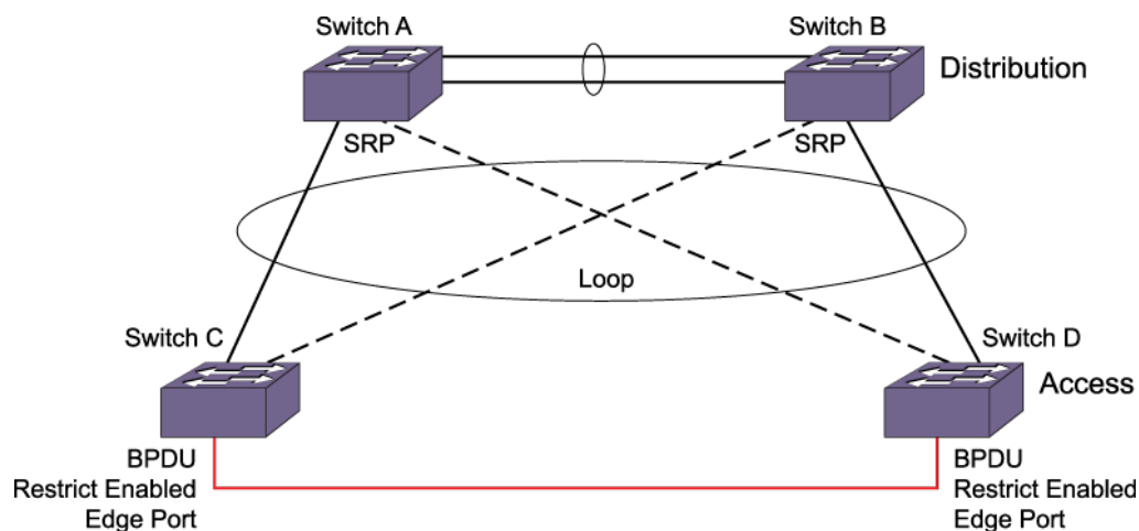
Figure 208: BPDU Restrict
