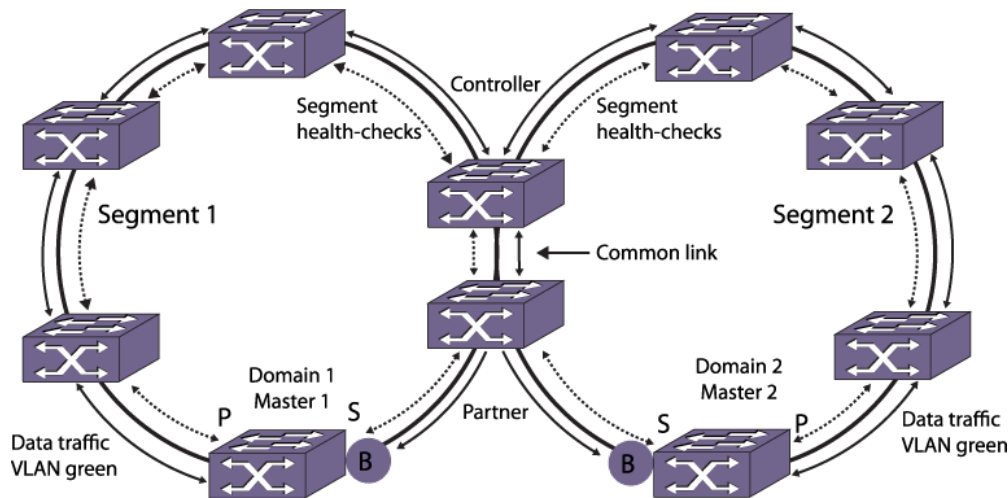
Figure 44: Segment Health-Check Messages
