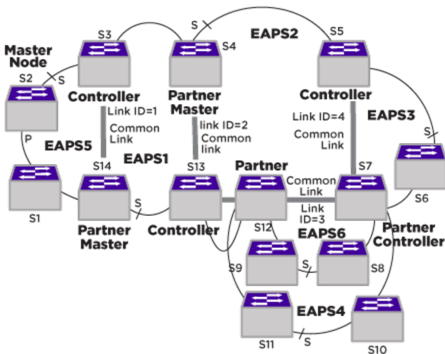
Figure 52: Advanced Basic Core and Right Angle Topology
