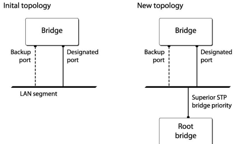
Figure 215: Example of Root Port Rapid Behavior
