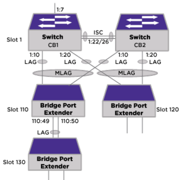
Figure 82: Redundant CBs with Two-Tier BPEs Topology
