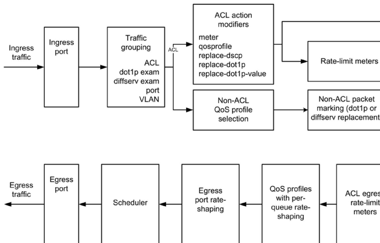
Figure 184: QoS on SummitStack and ExtremeSwitching Switches
