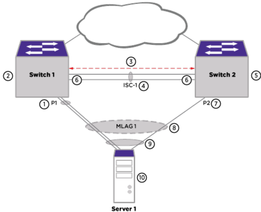
Figure 11: MLAG Elements
