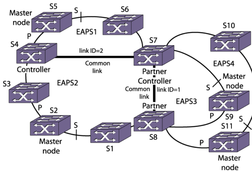
Figure 50: Right-Angle Topology
