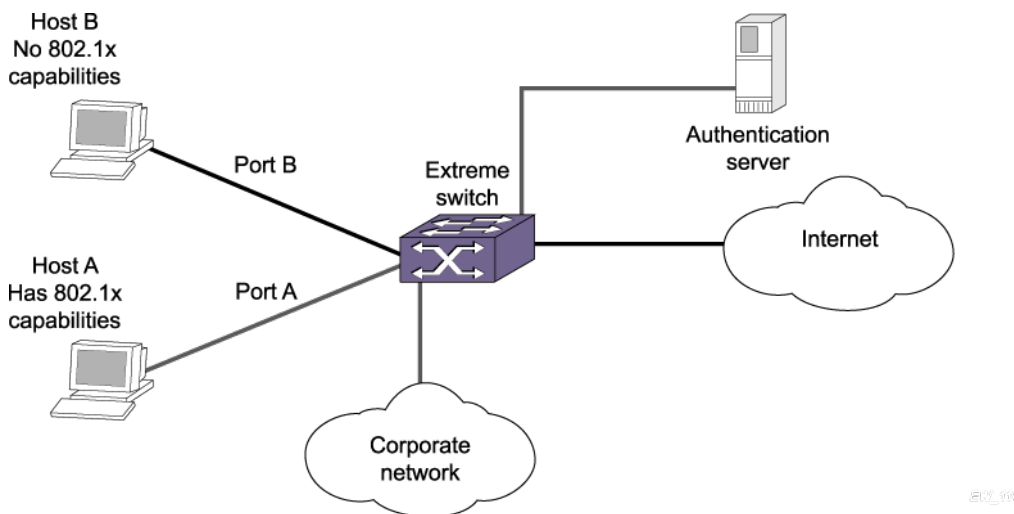
Figure 155: Guest VLAN for Network Login
