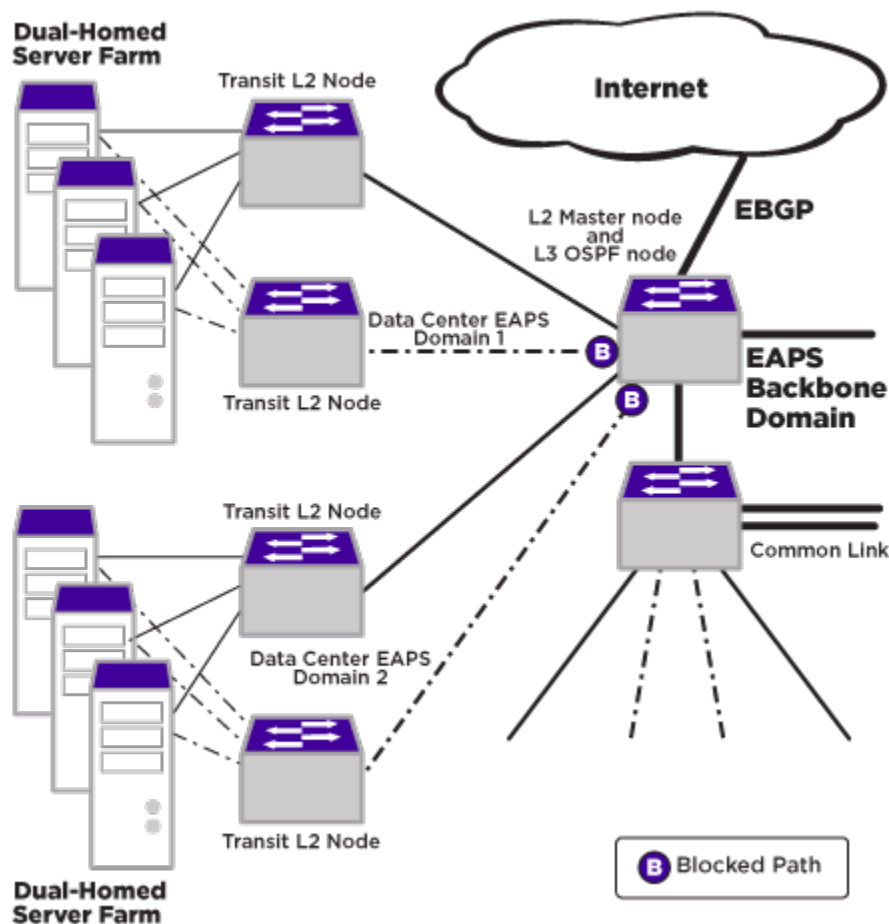
Figure 60: Data Center EAPS and OSPF Network Layer
