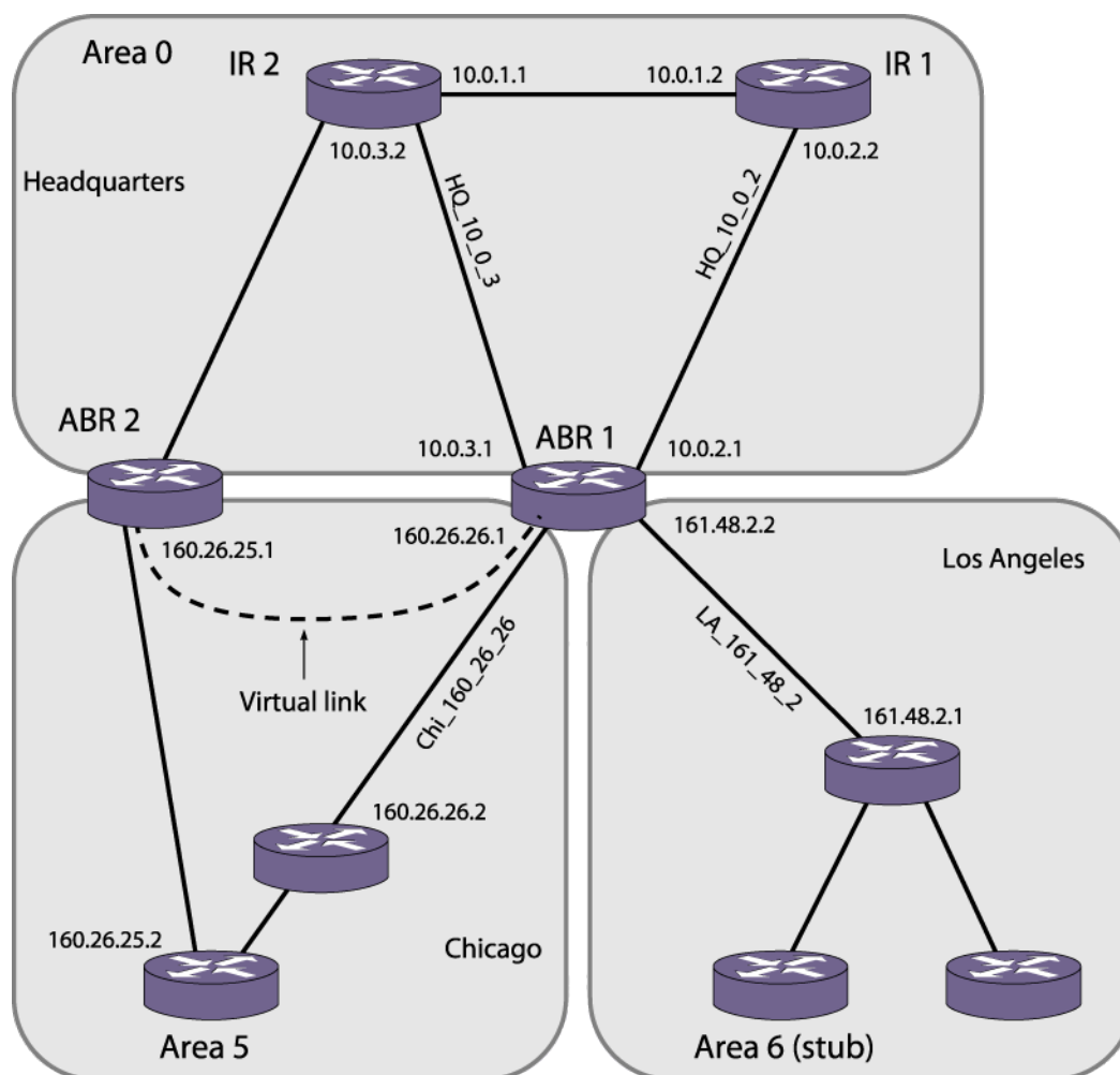
Figure 174: OSPF Configuration Example
