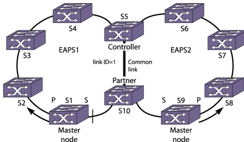
Figure 42: Multiple Rings Sharing a Common Link
