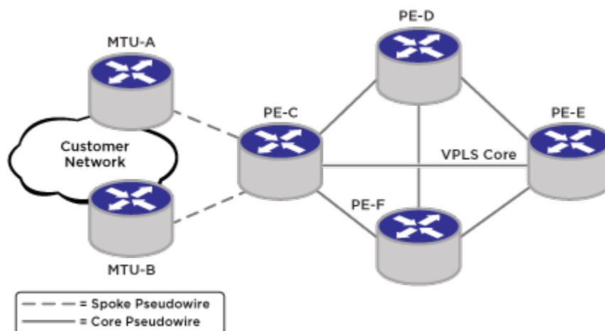
Figure 128: Example Protected Access H-VPLS Network
