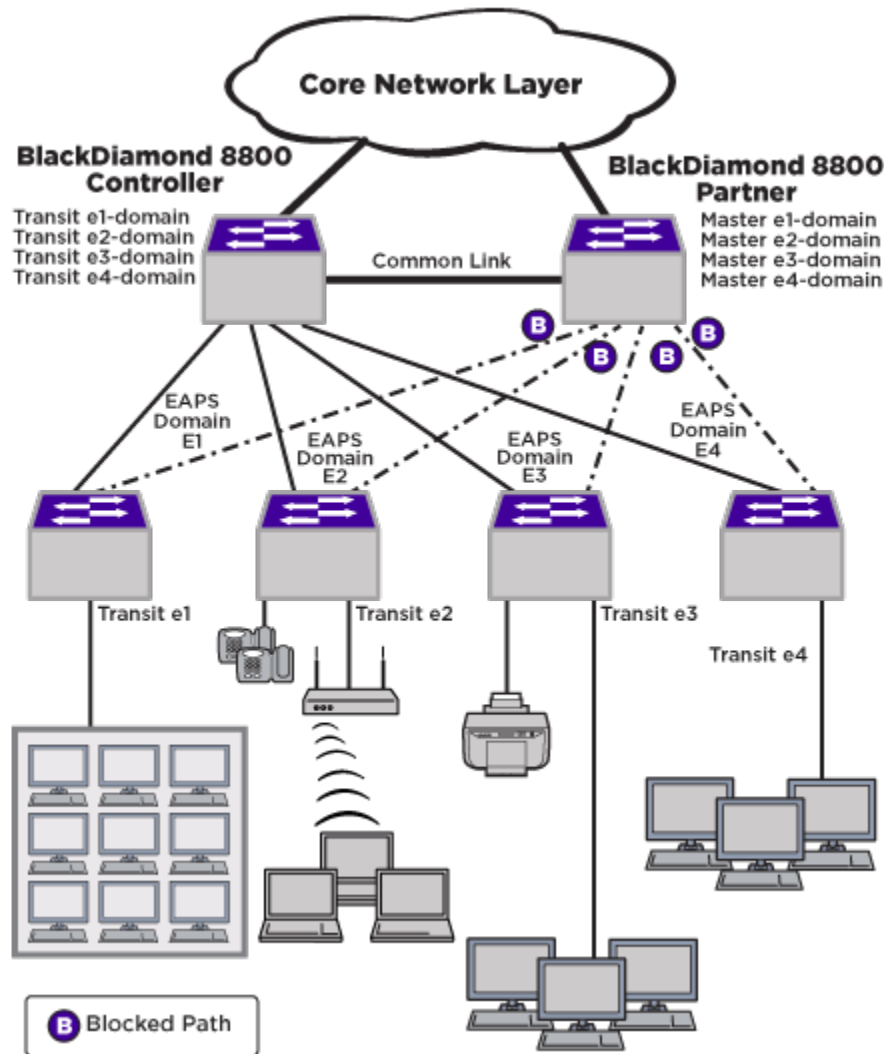
Figure 57: L2 Aggregation Network Layer
