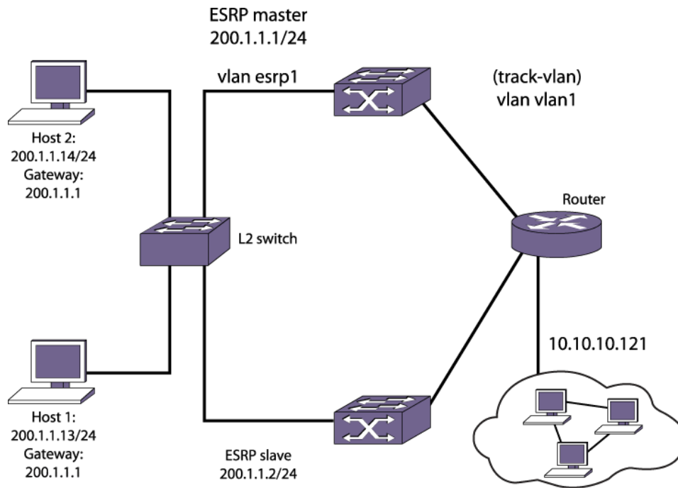
Figure 65: ESRP Tracking
