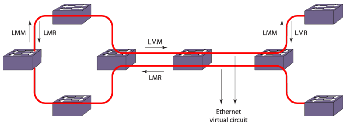
Figure 162: Two-Way Frame-Loss Measurement
