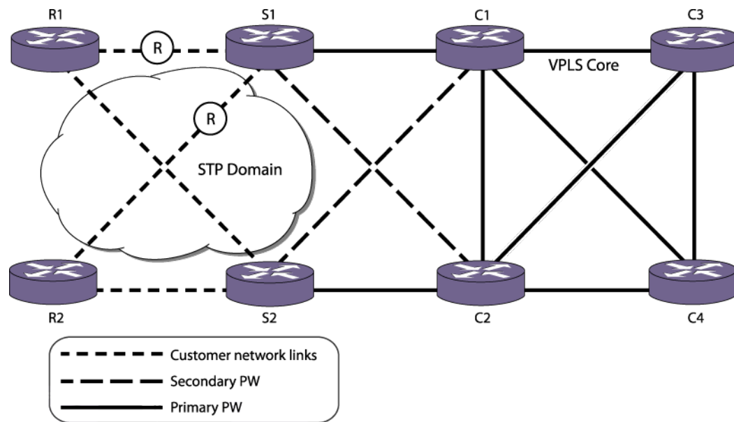
Figure 130: Redundant Edge H-VPLS Network with STP Example
