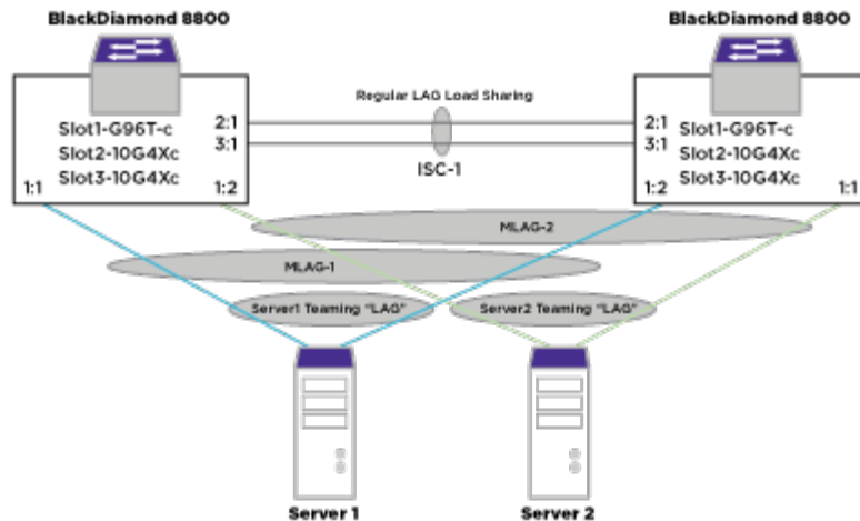
Figure 18: Simple MLAG Configuration
