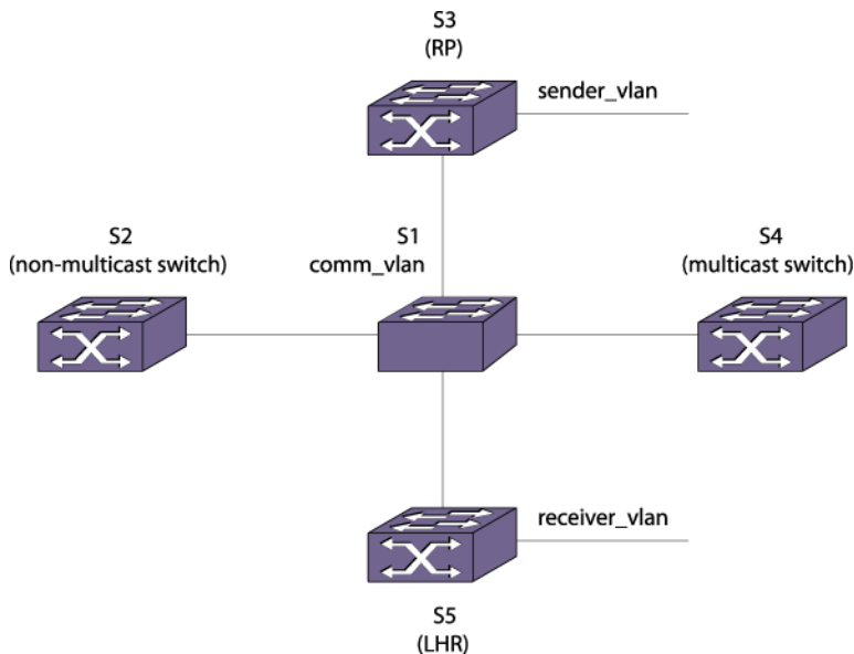
Figure 147: PIM Snooping Configuration Example
