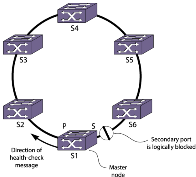
Figure 40: EAPS Operation
