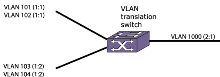
Figure 250: VLAN Translation Configuration Example
