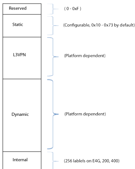
Figure 123: MPLS Label Space Partitions
