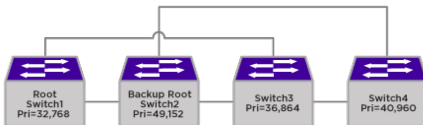
Figure 203: STP Root Bridge Loss Example
