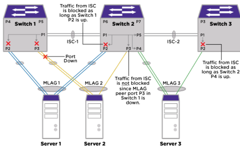
Figure 16: Peer Port Failure
