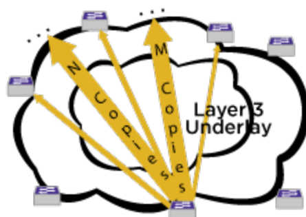
Figure 270: Example Head-End Replication Topology
