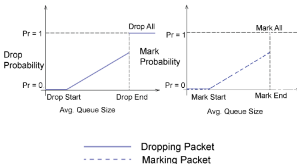
Figure 183: WRED Behavior with and without ECN
