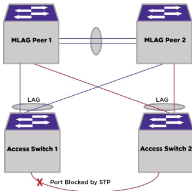
Figure 229: MLAG and MSTP/RSTP
