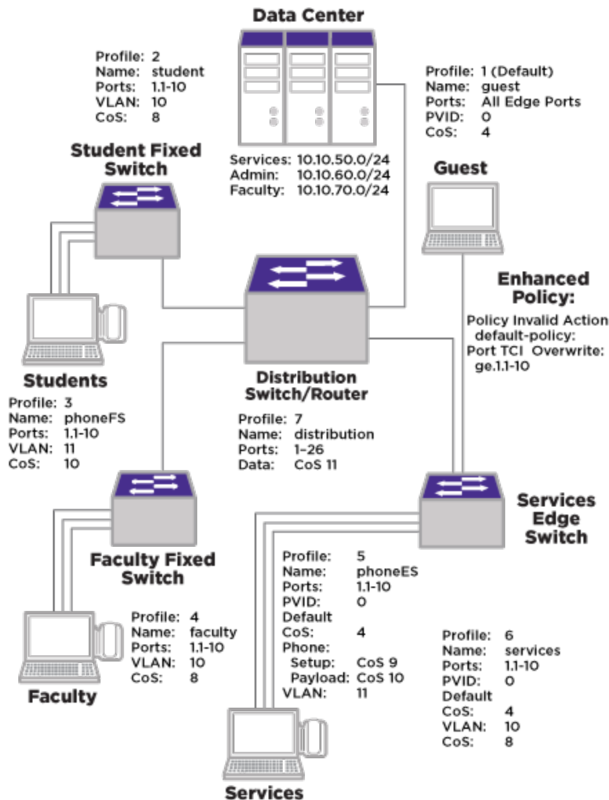
Figure 168: College-Based Policy Configuration
