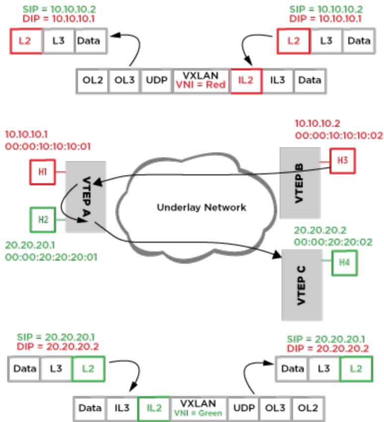
Figure 267: Routing in and out of a Tunnel
