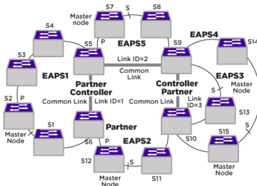
Figure 51: Basic Core and Right Angle Topology
