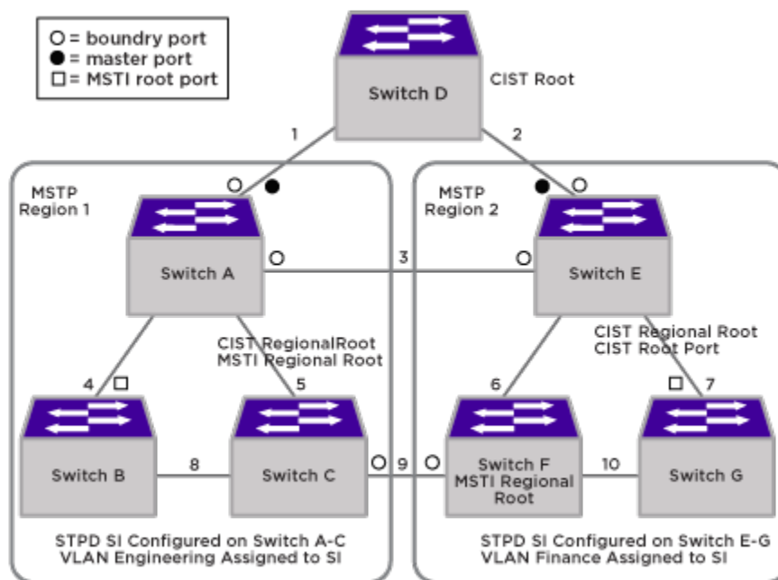
Figure 232: MSTP Configuration Example
