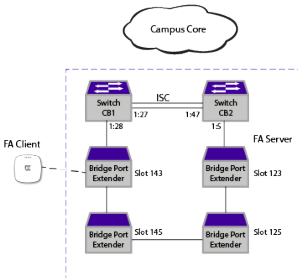
Figure 86: FA Clients Connect to BPE with Ring MLAG-Connected FA Server Peers
