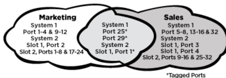
Figure 240: Logical Diagram of Tagged and Untagged Traffic
