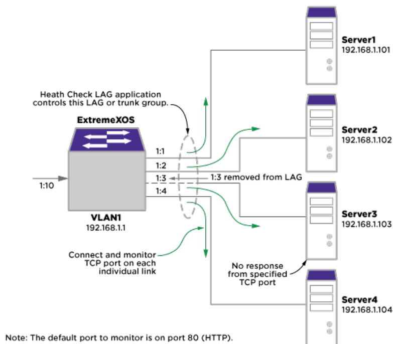
Figure 10: Health Check LAG Example
