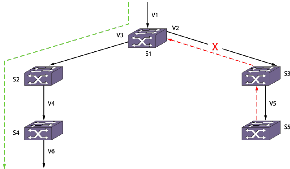
Figure 141: PIM-DM Operation
