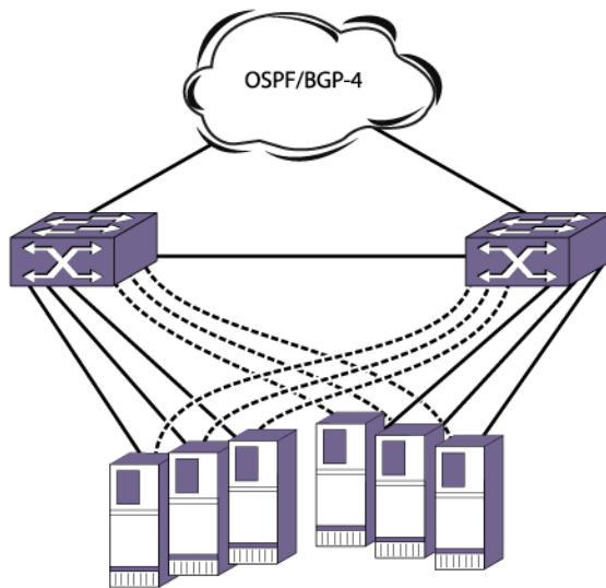
Figure 66: ESRP Host Attach
