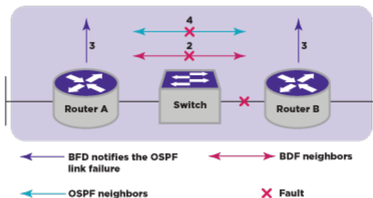
Figure 176: OSPFv3 Neighbor Relationship Eliminated by BFD Fault Detection
