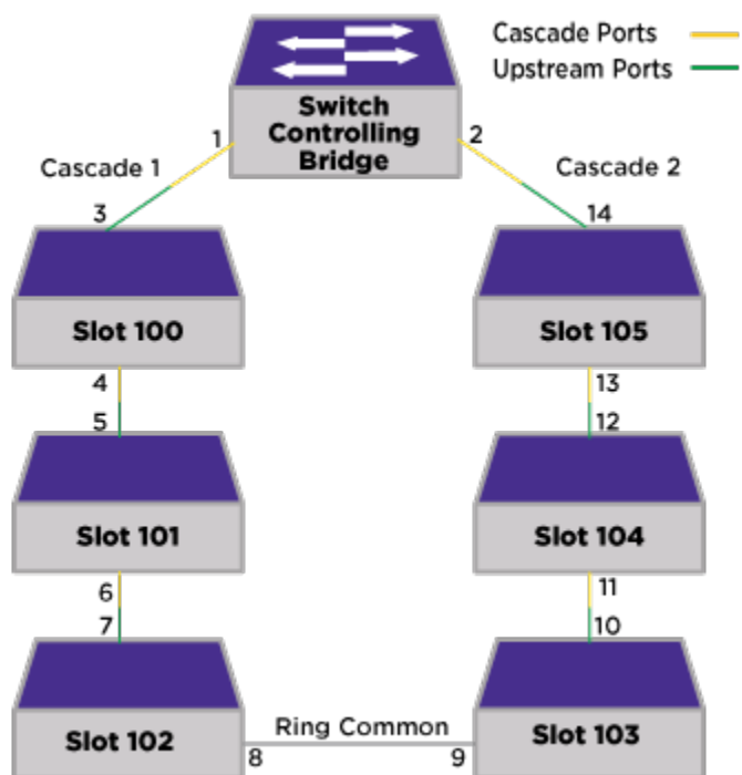
Figure 74: Simple Extended Edge Switching Ring
