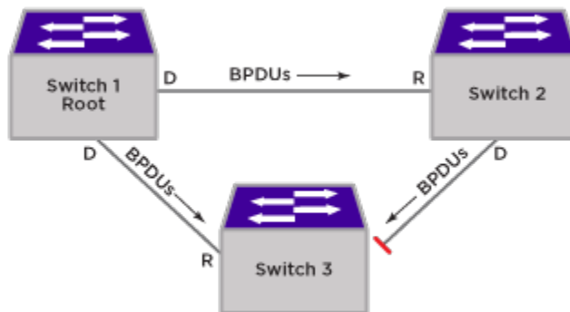
Figure 204: Switch 1 Elected as Root
