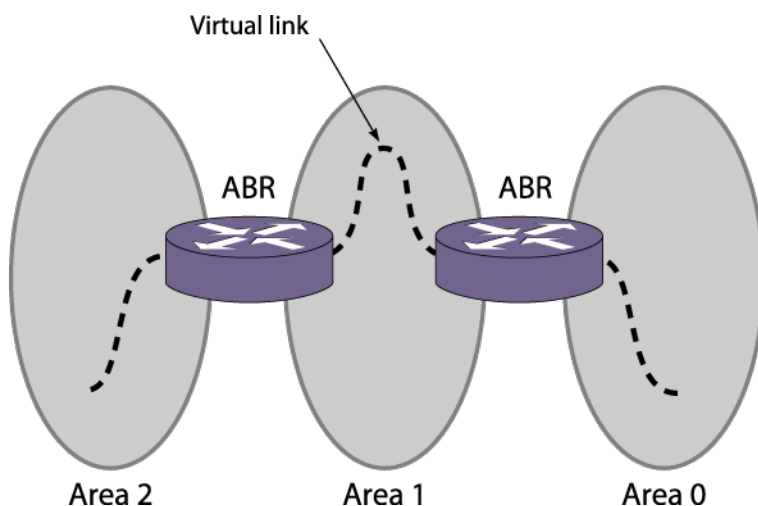
Figure 177: Virtual Link Using Area 1 as a Transit Area
