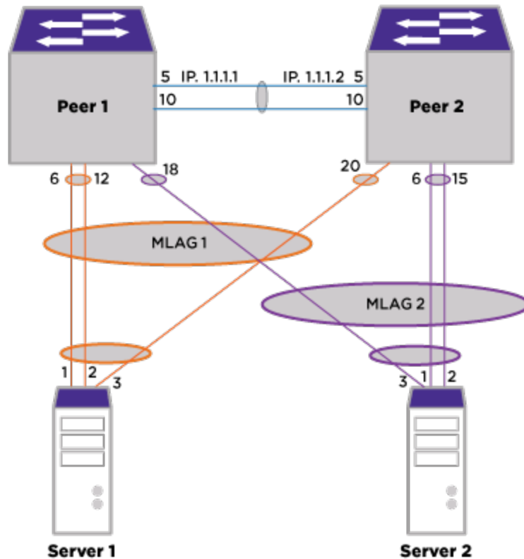
Figure 20: LACP Ports in MLAG Configuration
