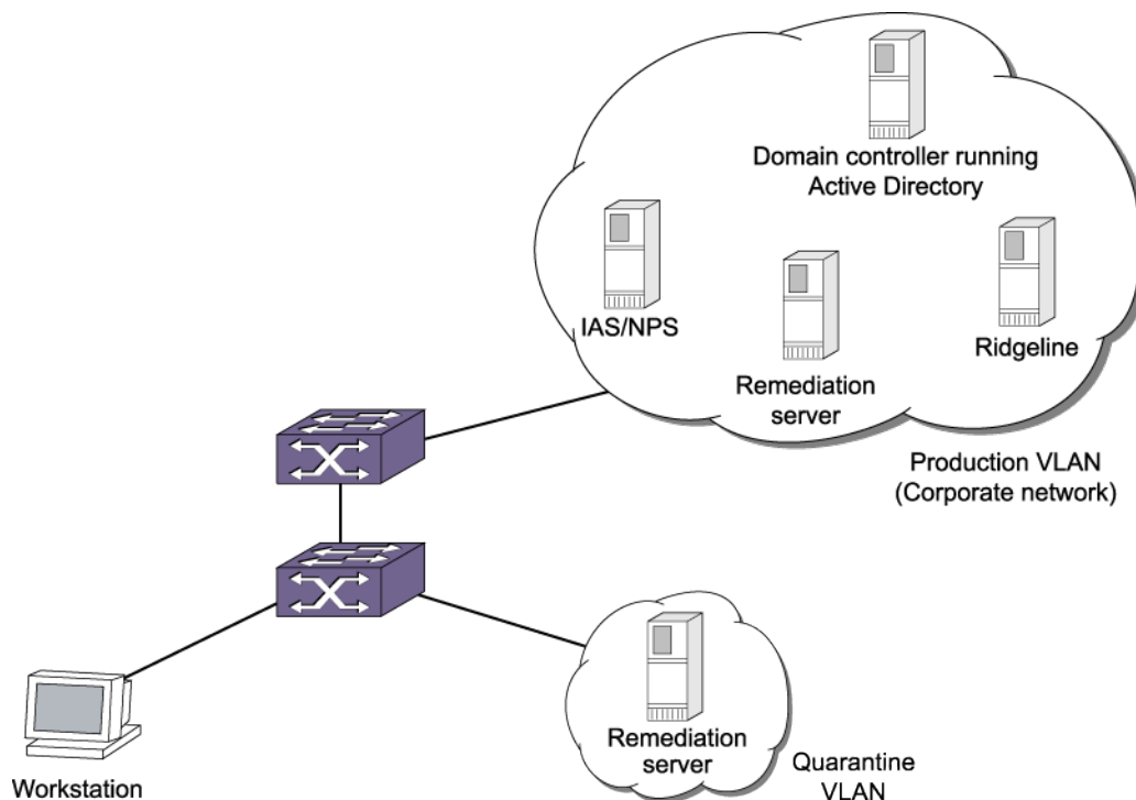
Figure 156: Sample Network Using NAP to Provide Enhanced Security
