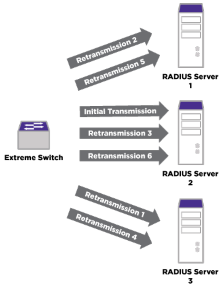
Figure 196: Authentication Retransmission Algorithm for a Single RADIUS Transaction (No Servers Responding 2)
