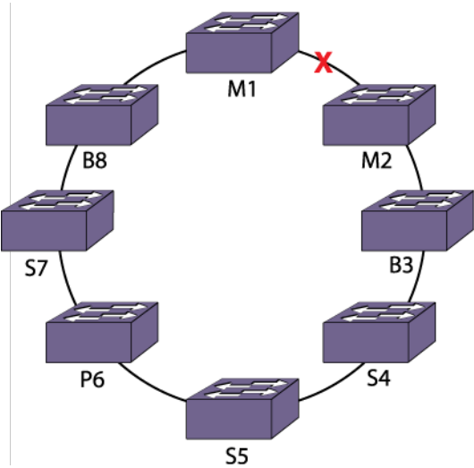
Figure 6: Example of a Split Stack that Results in a Dual Primary Situation
