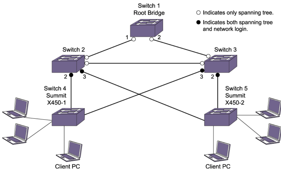
Figure 227: STP and Network Login Enabled
