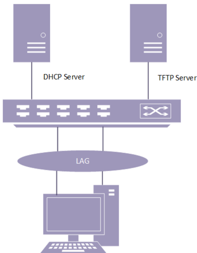
Figure 9: LACP Fallback
