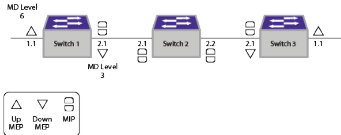
Figure 159: CFM Configuration Example
