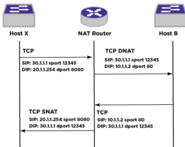
Figure 103: Destination Network Address Port Translation (NAPT)
