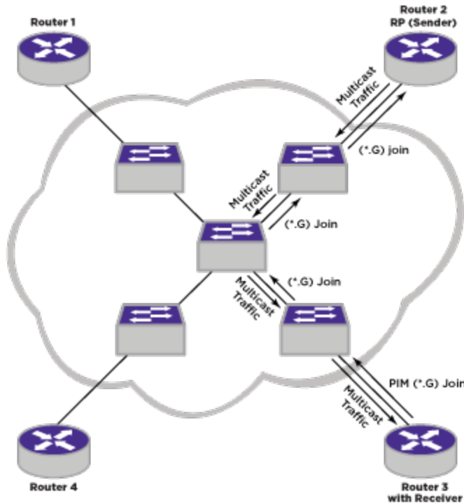
Figure 143: Multicast With PIM Snooping
