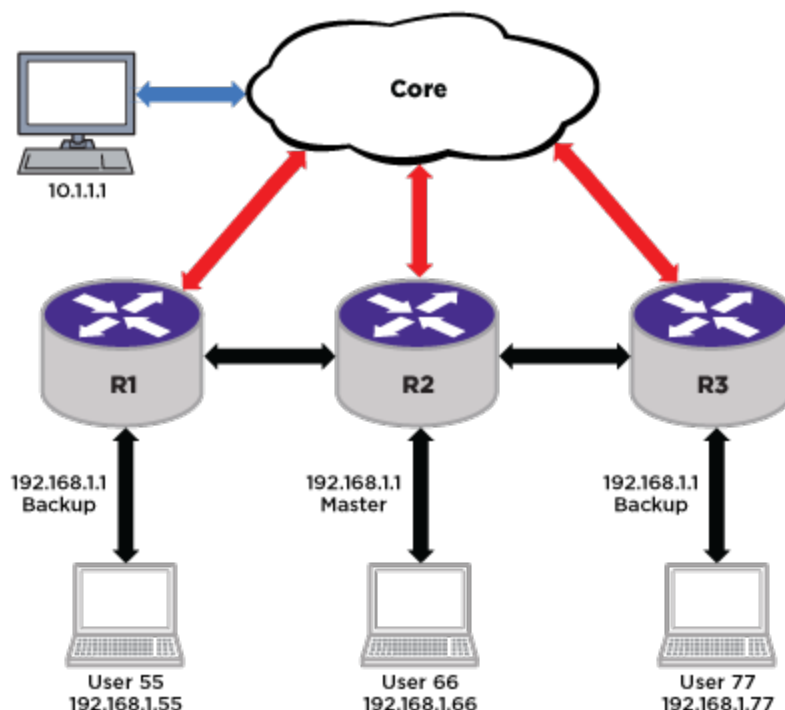
Figure 262: Asymmetric Routing and VRRP (1)
