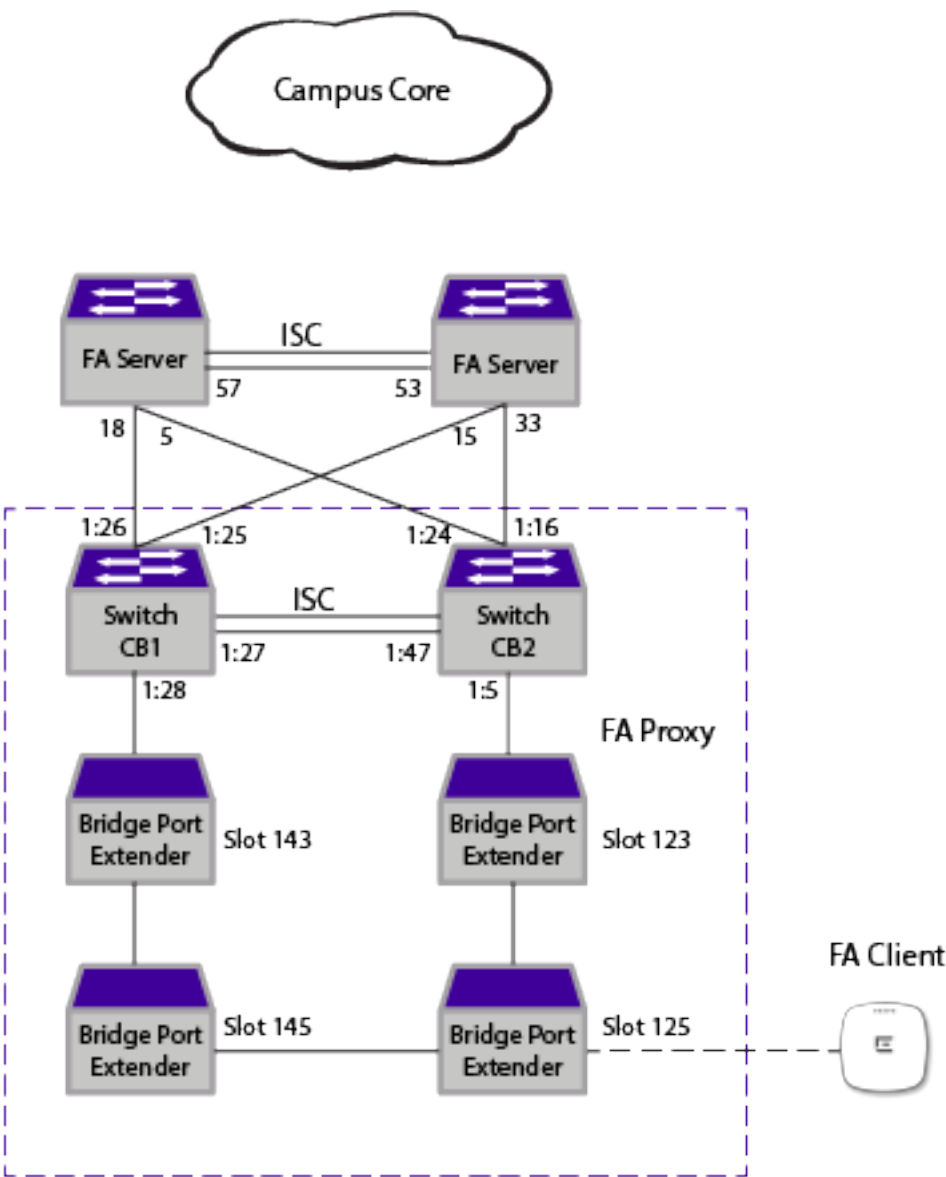
Figure 87: FA Clients Connect to BPE with Ring MLAG-Connected FA Proxy Peers
