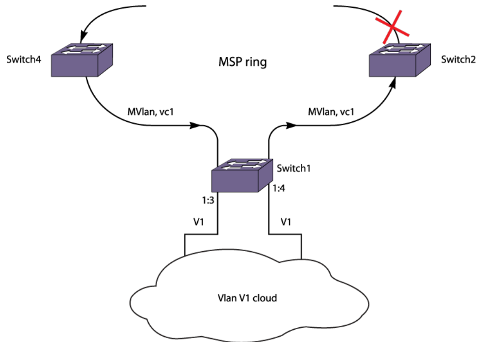
Figure 153: MVR with STP
