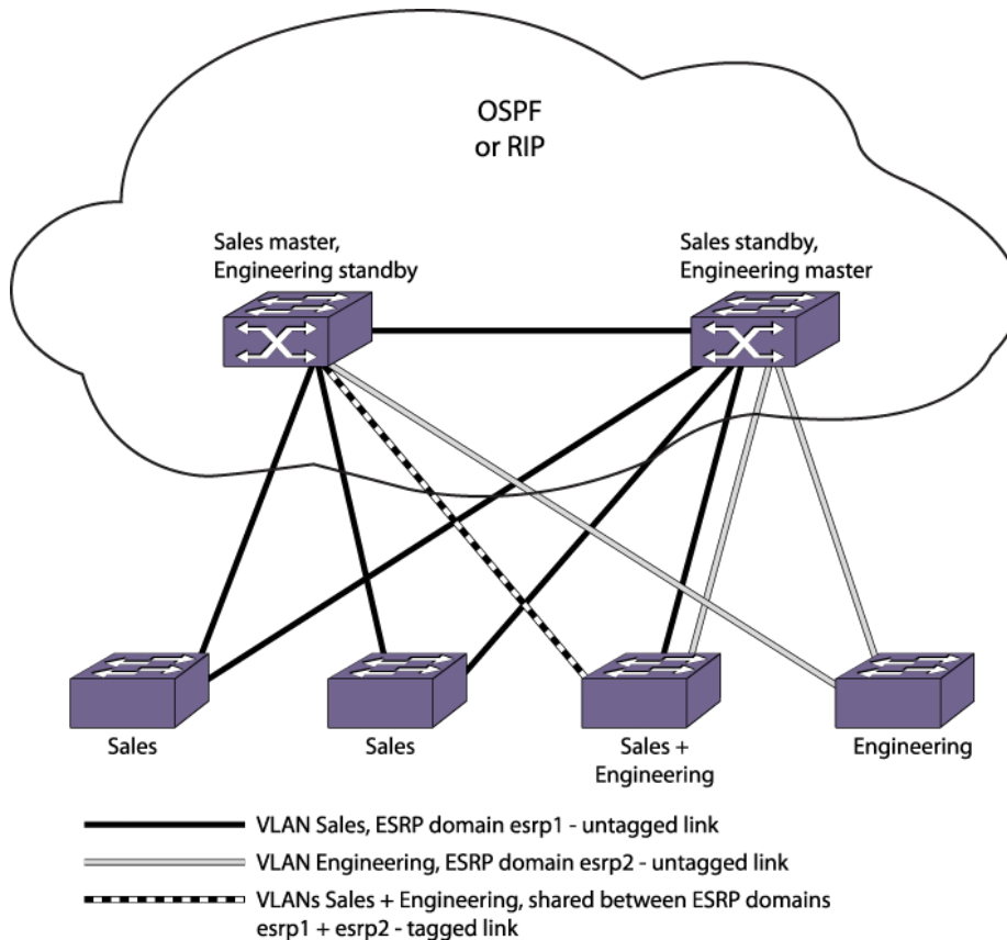
Figure 68: Multiple ESRP Domains Using Layer 2 and Layer 3 Redundancy
