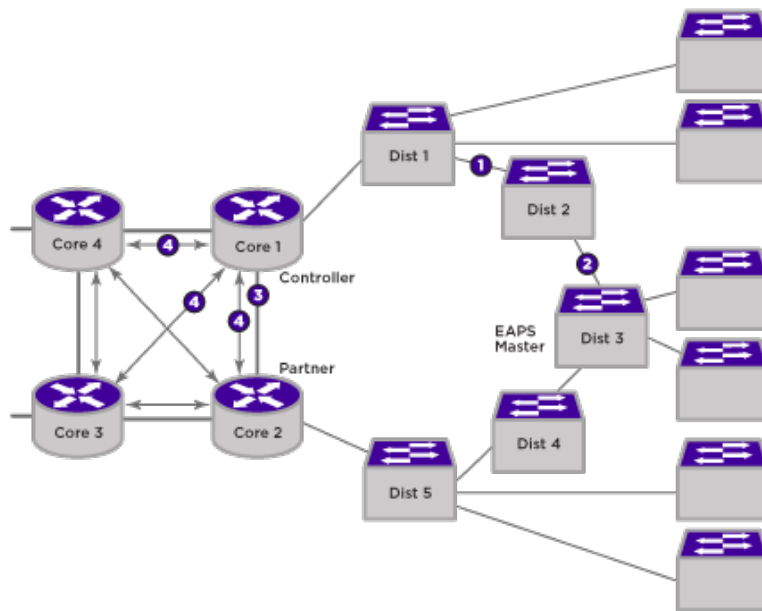
Figure 131: VPLS with Redundant EAPS Configuration Example
