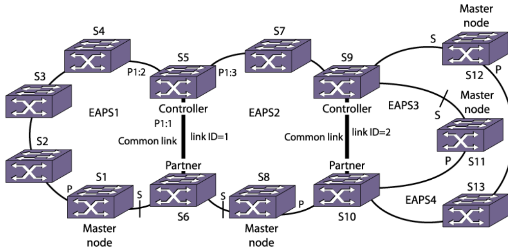
Figure 49: Basic Core Topology
