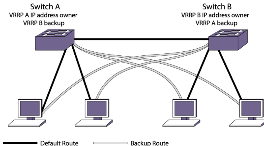
Figure 260: VRRP Load-sharing Configuration
