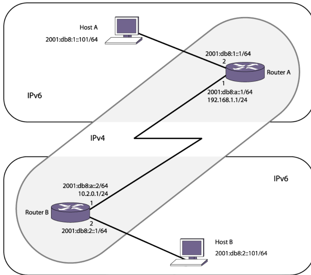
Figure 107: 6in4 Tunnel Example
