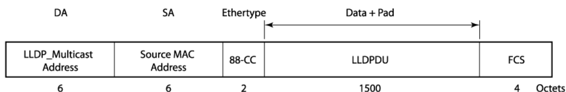
Figure 117: LLDP Packet Format
