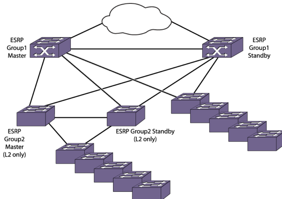
Figure 64: ESRP Groups
