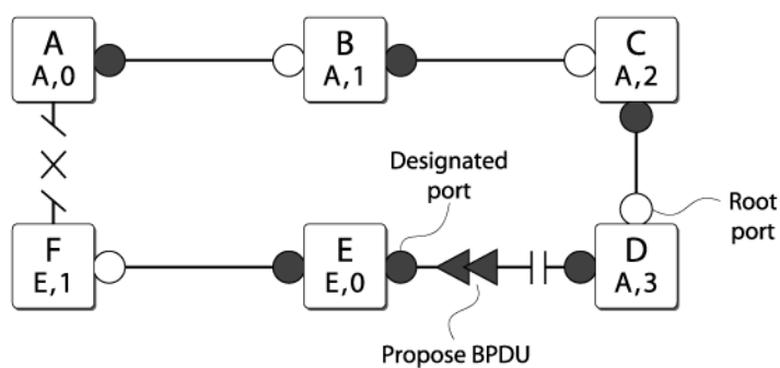
Figure 220: Sending a Propose Message to Confirm a Port Role
