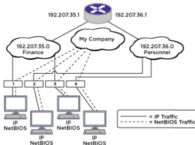
Figure 186: RIP Configuration Example
