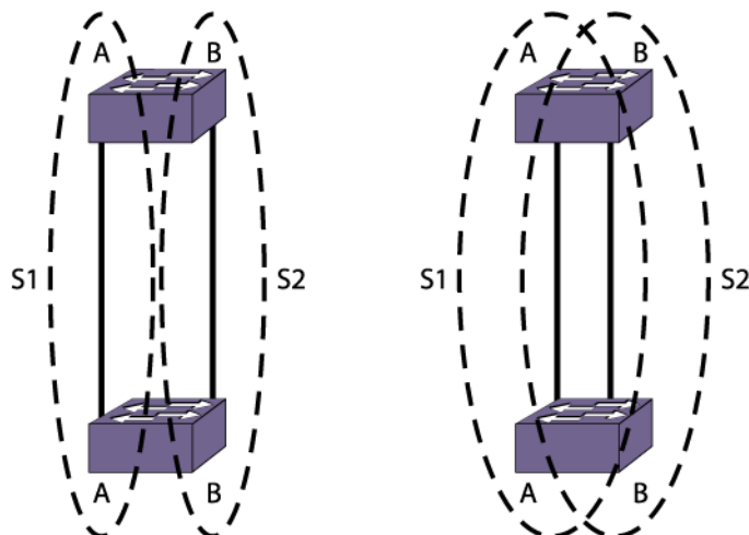
Figure 211: Limitations of Traditional STPD
