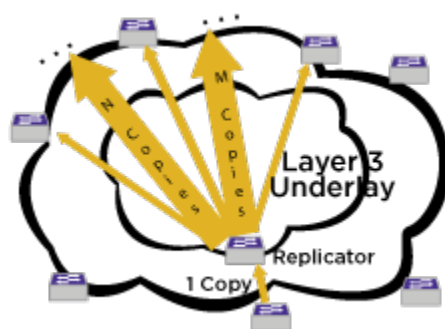
Figure 271: Example Assisted Replication Topology
