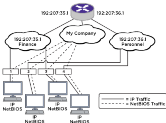
Figure 106: Unicast Routing Configuration Example
