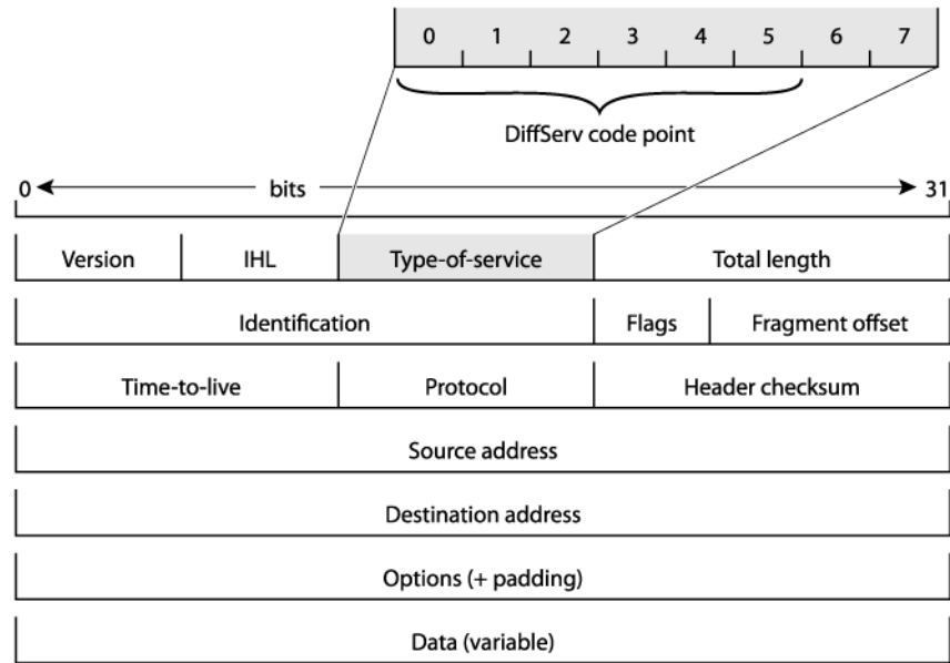
Figure 182: DiffServe Code Point
