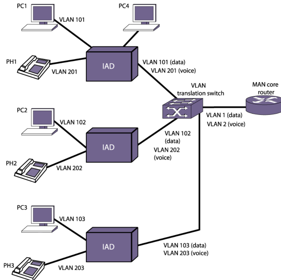
Figure 242: VLAN Translation Application
