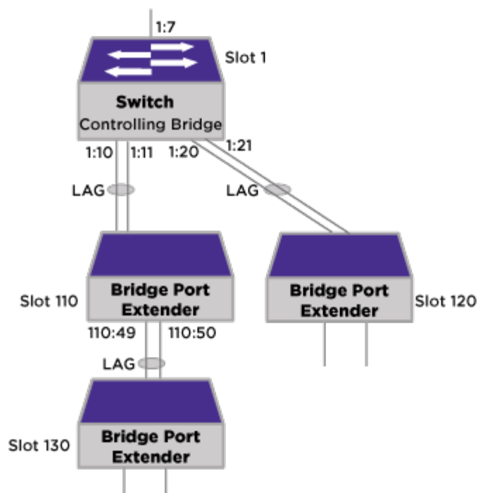
Figure 79: CB with Two-Tier BPEs Topology
