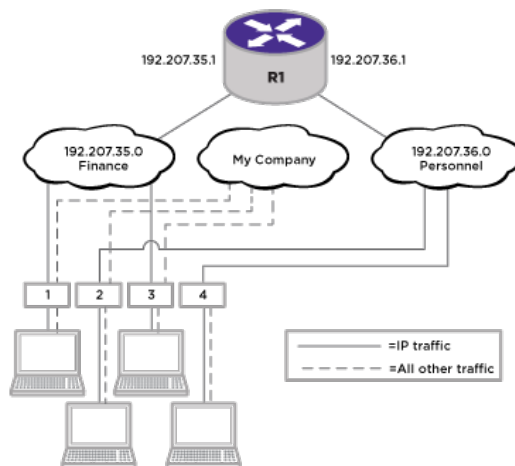
Figure 241: Protocol-Based VLANs
