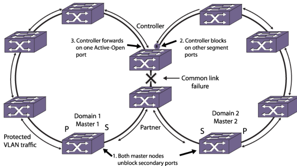
Figure 45: Common Link Failure
