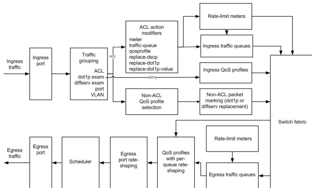
Figure 180: QoS on Extreme Networks Switches
