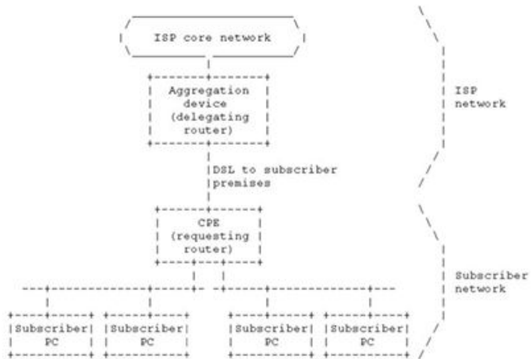
Figure 105: Prefix Delgation Example
