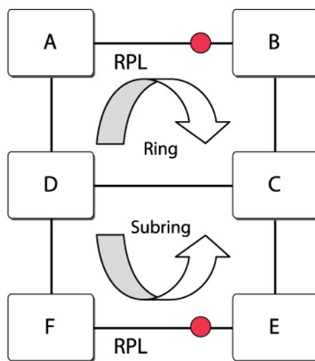
Figure 62: Ring and Sub-ring Network
