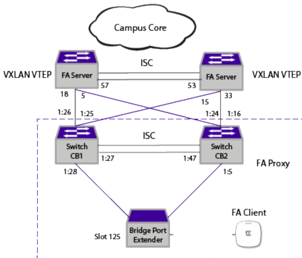
Figure 89: Cross-Connect MLAG Topology
