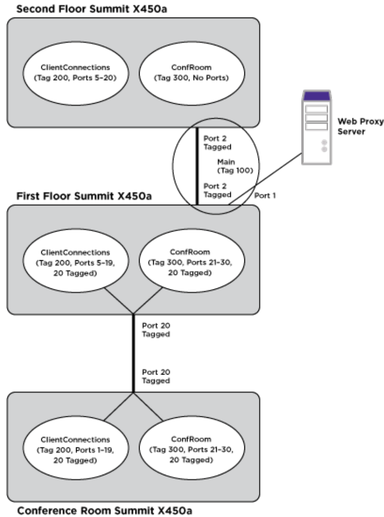
Figure 248: PVLAN Configuration Example 2
