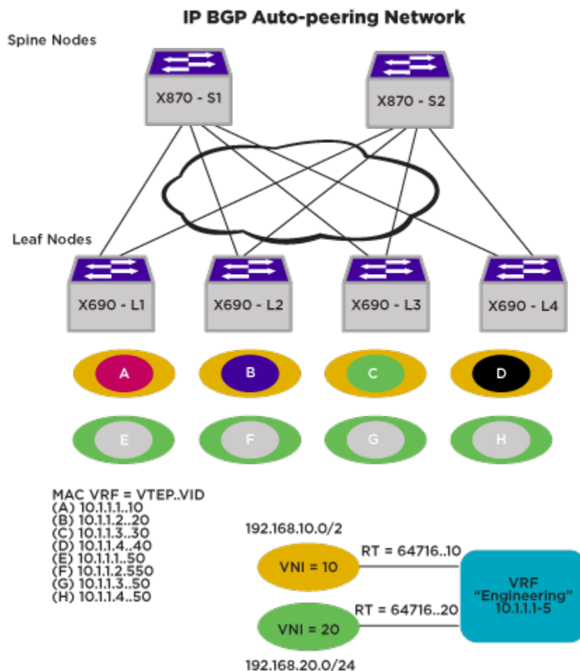
Figure 36: EVPN and Asymmetric VRF Routing in BGP Auto-peering
