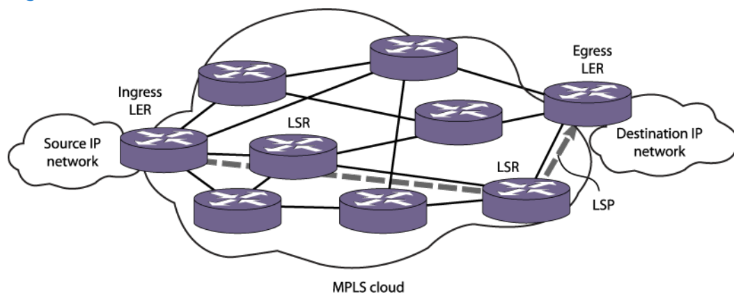
Figure 118: MPLS Network
