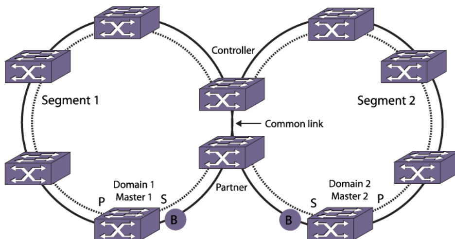
Figure 43: Master Node Operation in a Multiple Ring Topology
