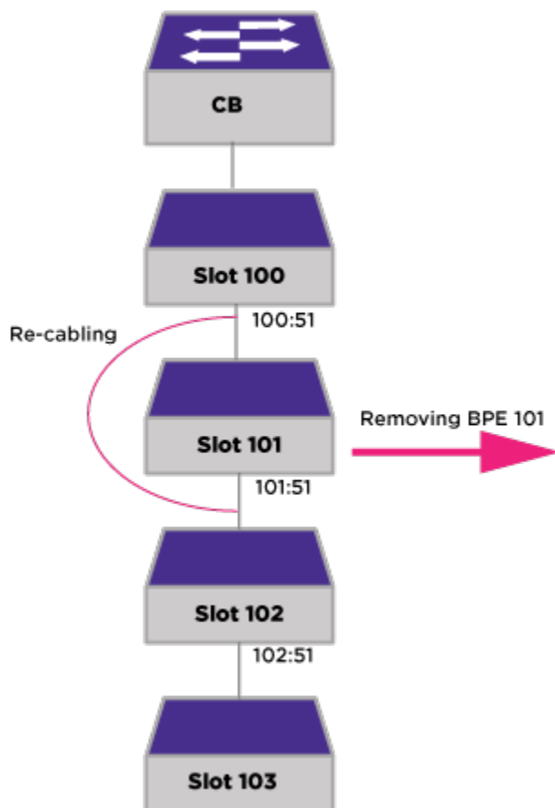
Figure 81: Removing BPE from Cascade
