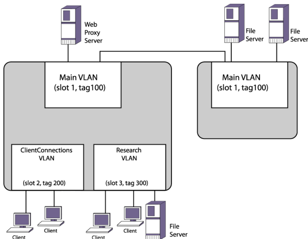
Figure 247: PVLAN Configuration Example 1
