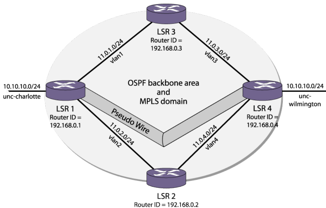
Figure 138: MPLS VPLS Configuration Example
