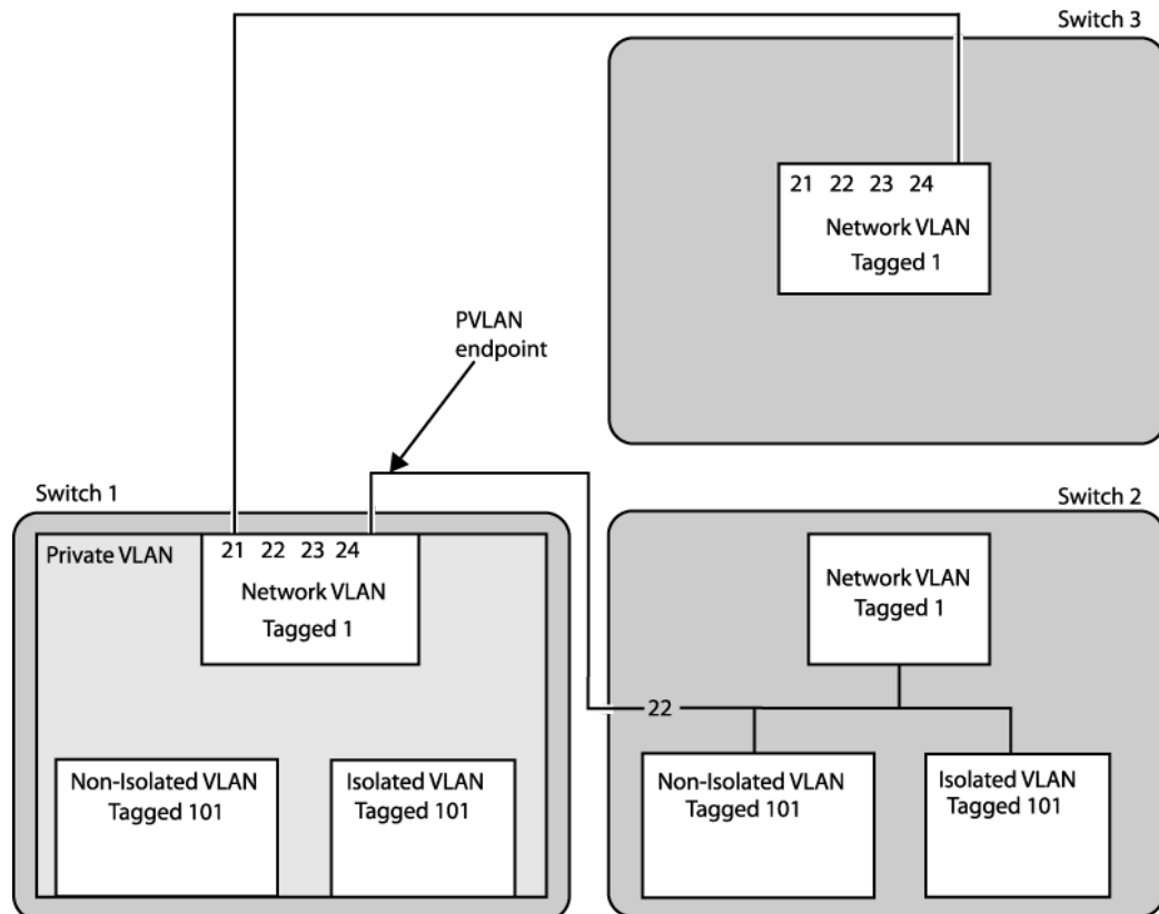
Figure 246: Private VLAN Connections to Switches Outside the PVLAN
