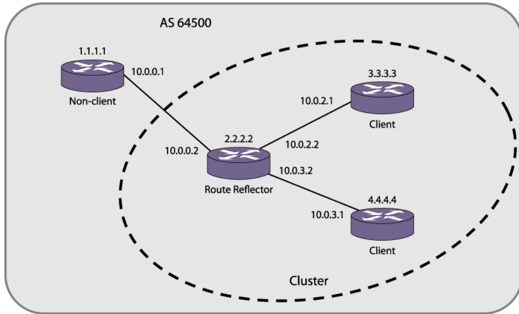
Figure 27: Route Reflectors
