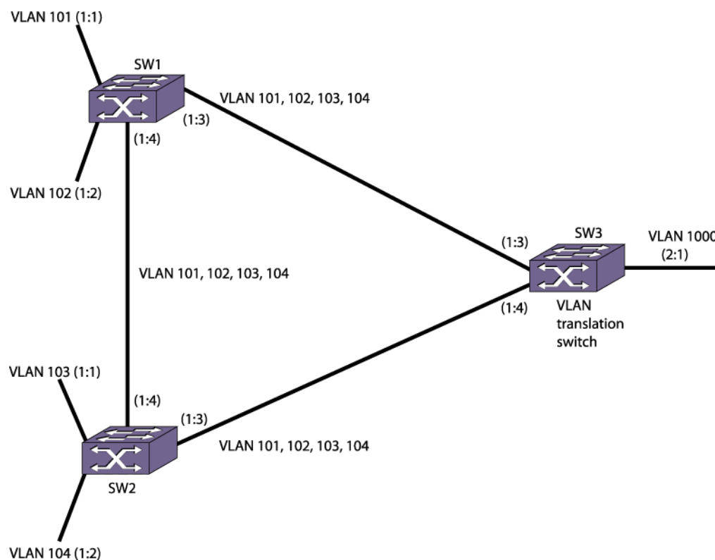
Figure 252: STP Redundancy Configuration Example
