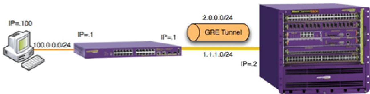
Figure 95: GRE Tunnel Configuration
