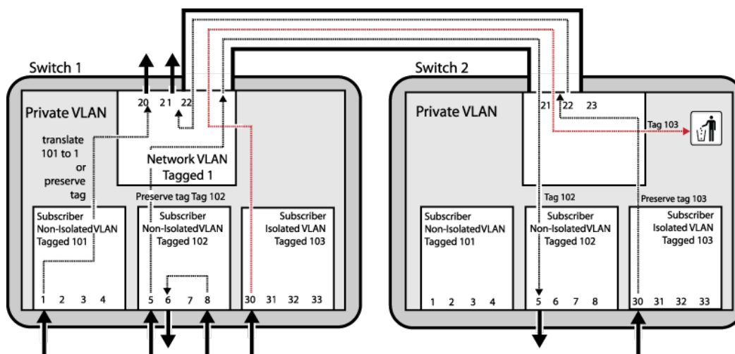
Figure 245: Private VLAN Support on Multiple Switches
