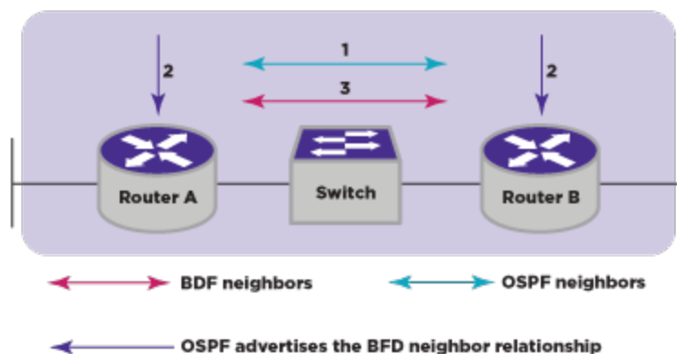
Figure 169: Basic Operational Flow of OSPF BFD
