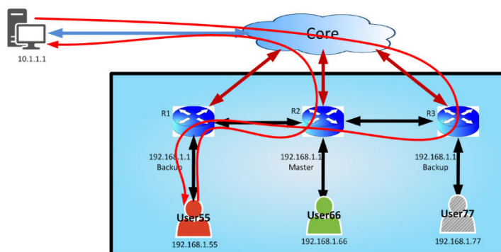
Figure 263: Asymmetric Routing and VRRP (2)
