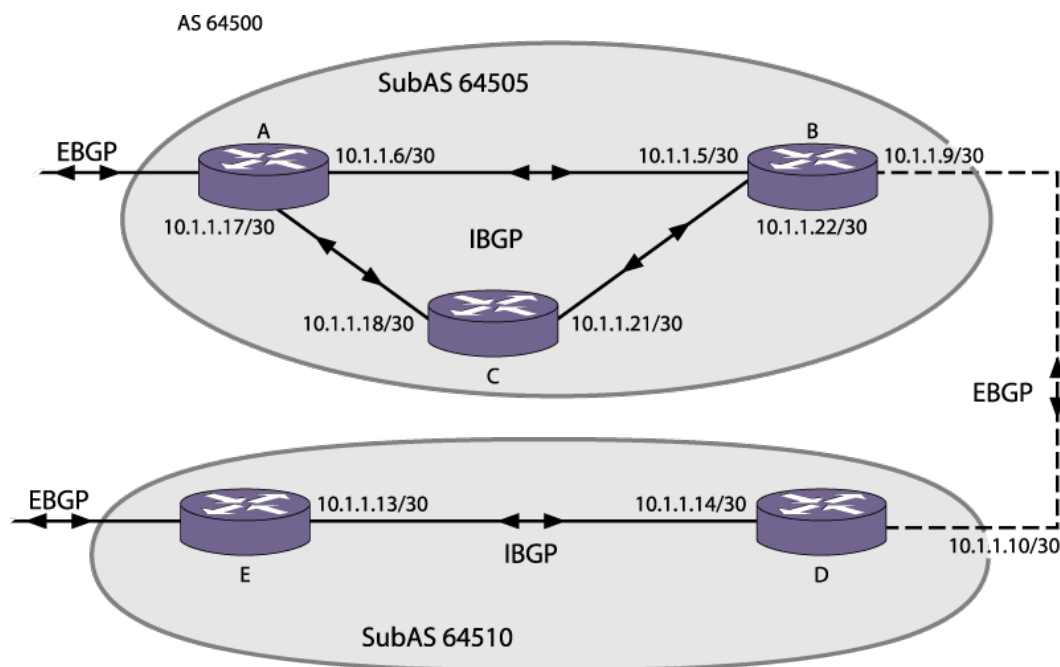
Figure 28: Routing Confederation
