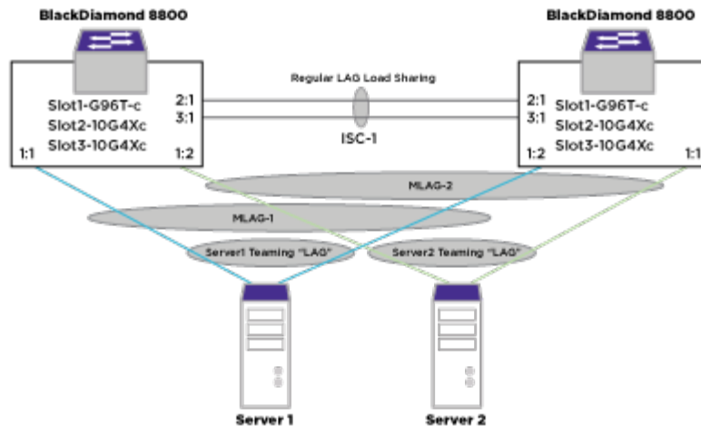
Figure 18: Simple MLAG Configuration
