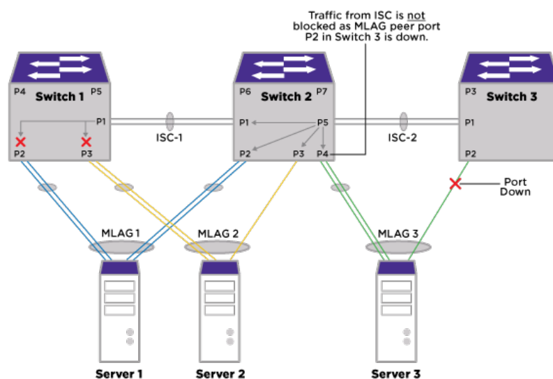
Figure 17: Peer Port Failure (cont.)
