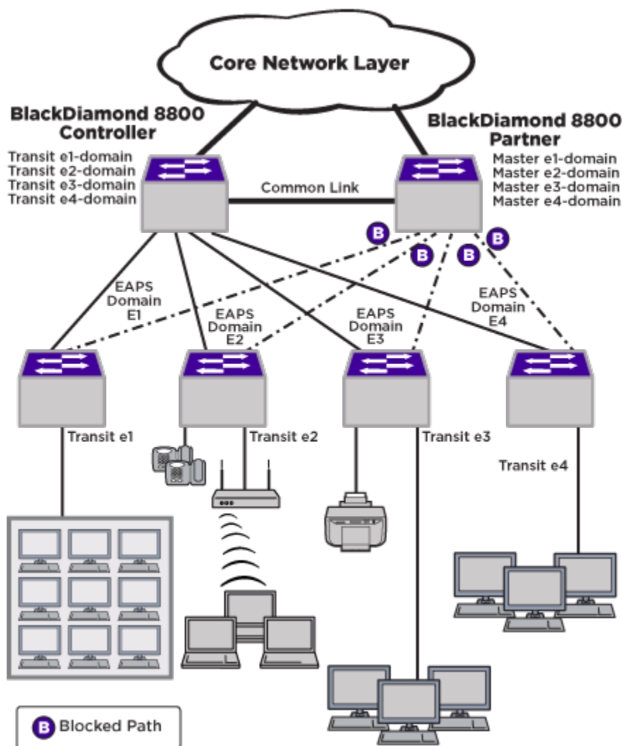
Figure 57: L2 Aggregation Network Layer
