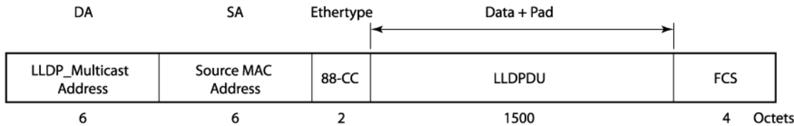
Figure 117: LLDP Packet Format
