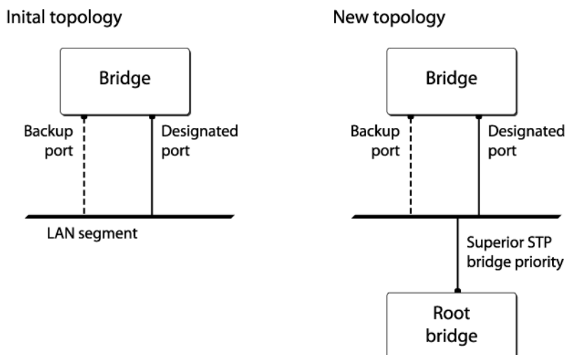
Figure 215: Example of Root Port Rapid Behavior
