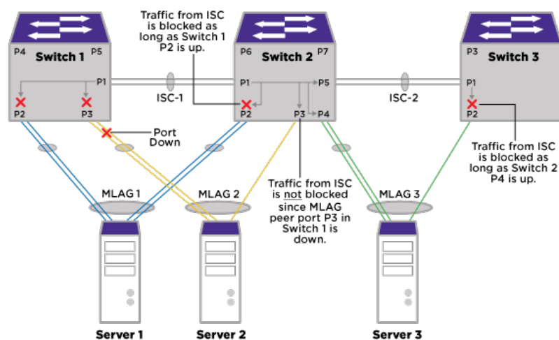
Figure 16: Peer Port Failure
