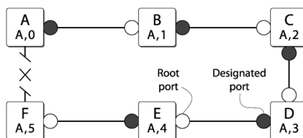
Figure 223: Final Network Configuration
