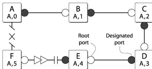
Figure 222: Completing the Topology Change
