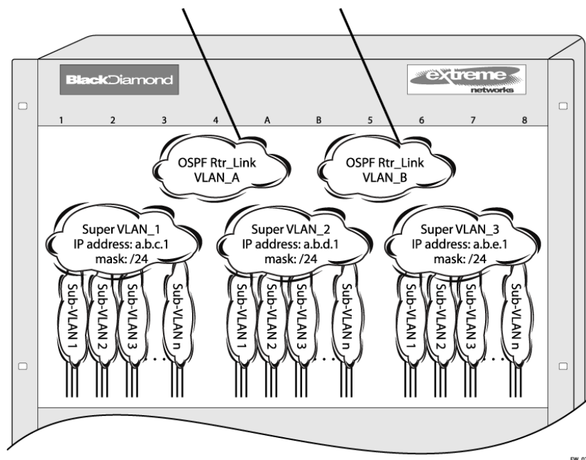
Figure 99: VLAN Aggregation
