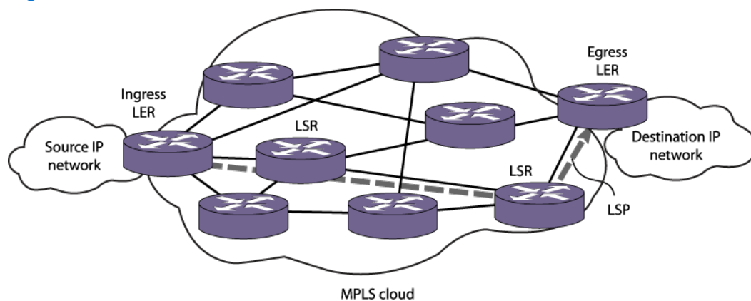
Figure 118: MPLS Network
