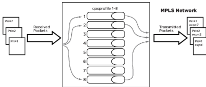
Figure 136: Mapping Dot1p to EXP Bits
