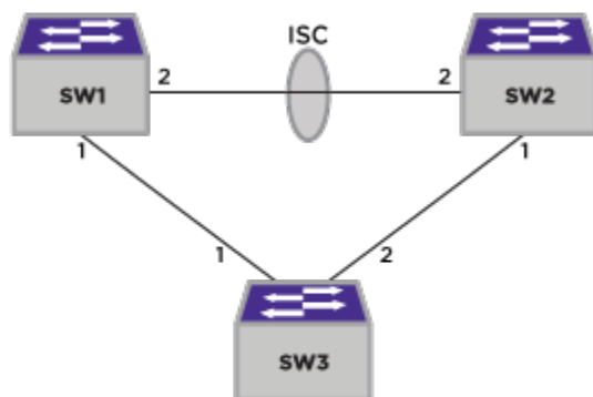
Figure 233: ELRP Egress Port Disable (1)
