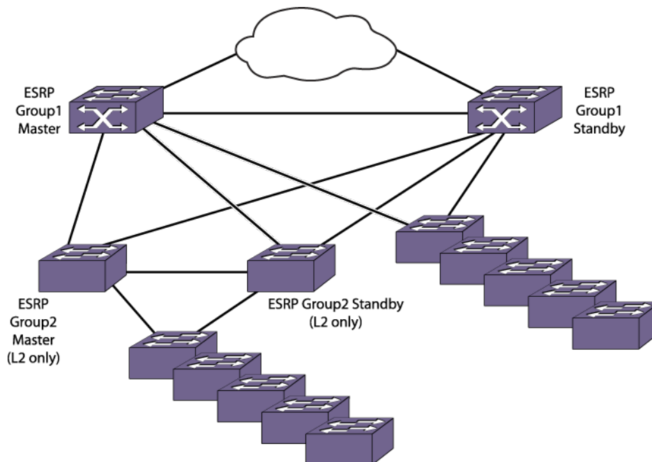
Figure 64: ESRP Groups
