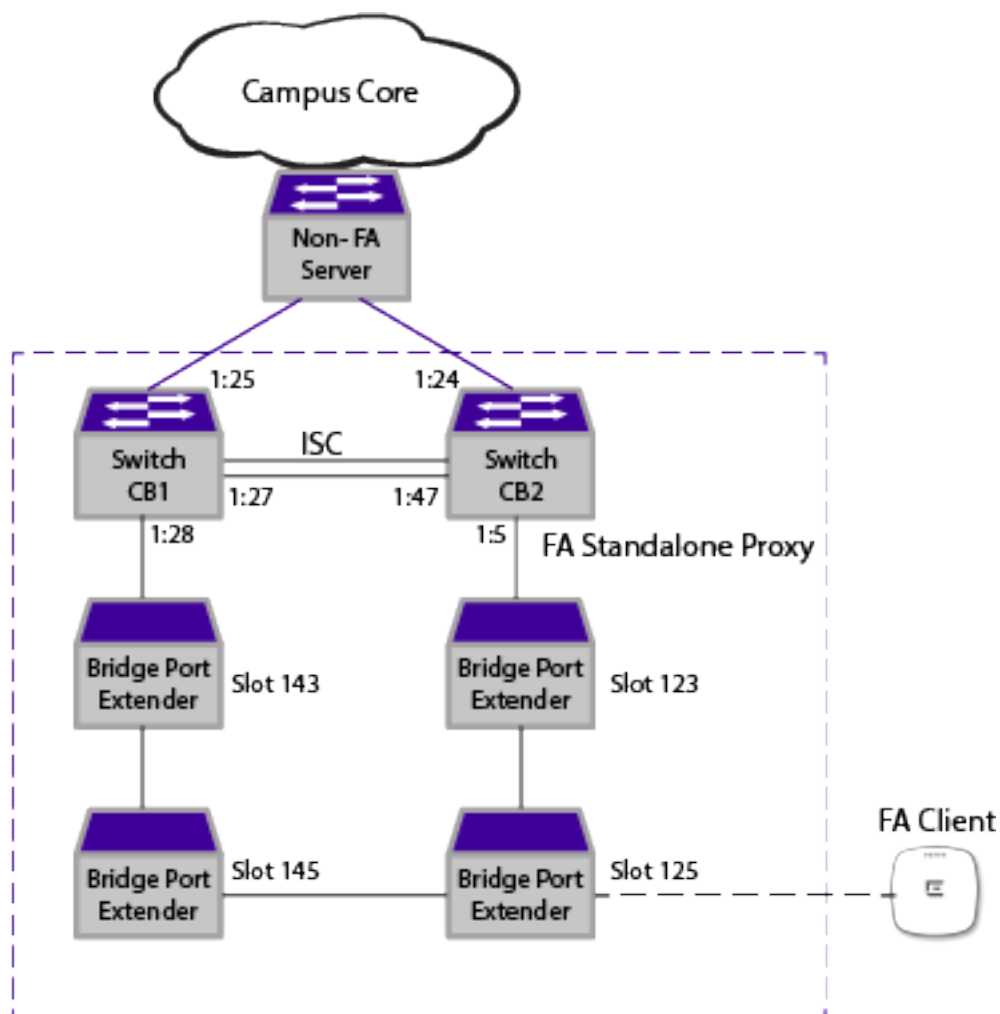
Figure 88: FA Clients Connected to BPEs with Extended Edge Switching Ring MLAG-Connected CBs FA Standalone Peers
