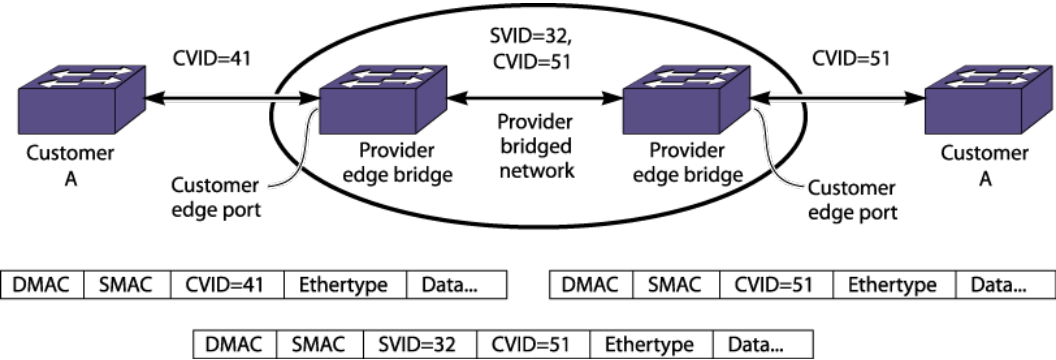
Figure 256: CVID Translation
