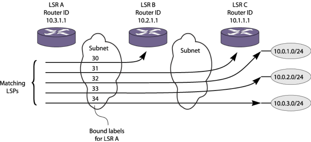
Figure 124: Matching and Calculated LSP Next Hops
