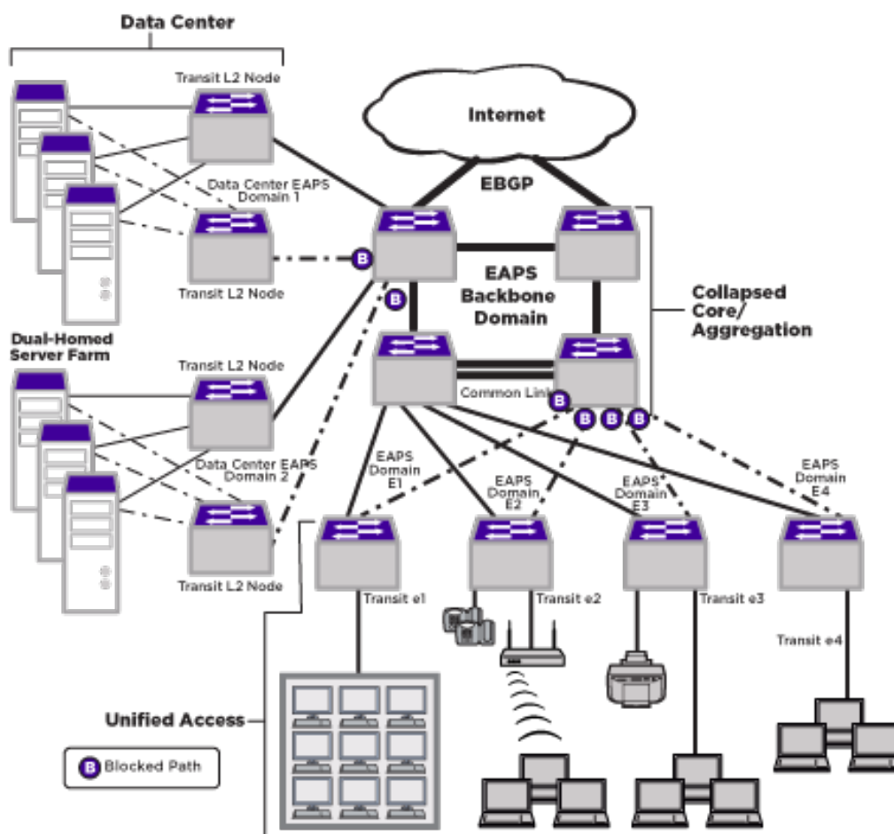
Figure 55: Extreme Networks EAPS Everywhere
