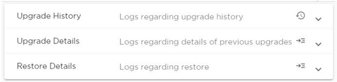
Figure 15: Logs tab
