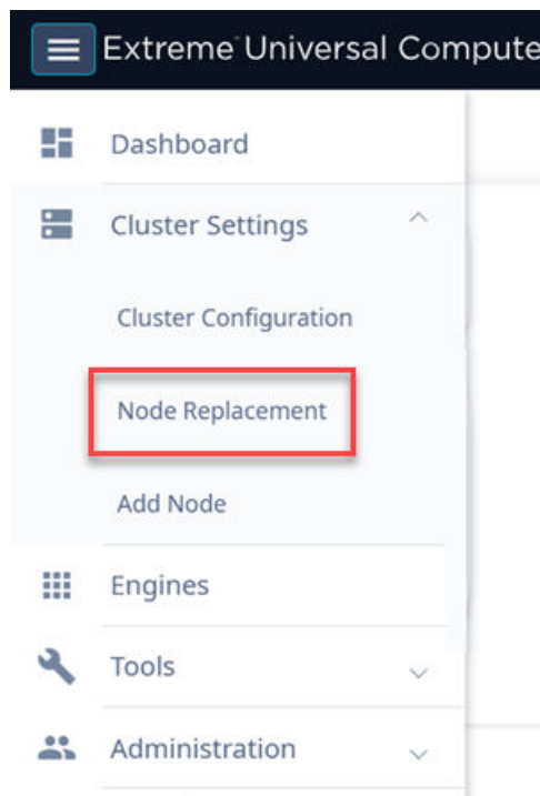
Figure 4: Node Replacement
