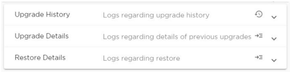
Figure 15: Logs tab
